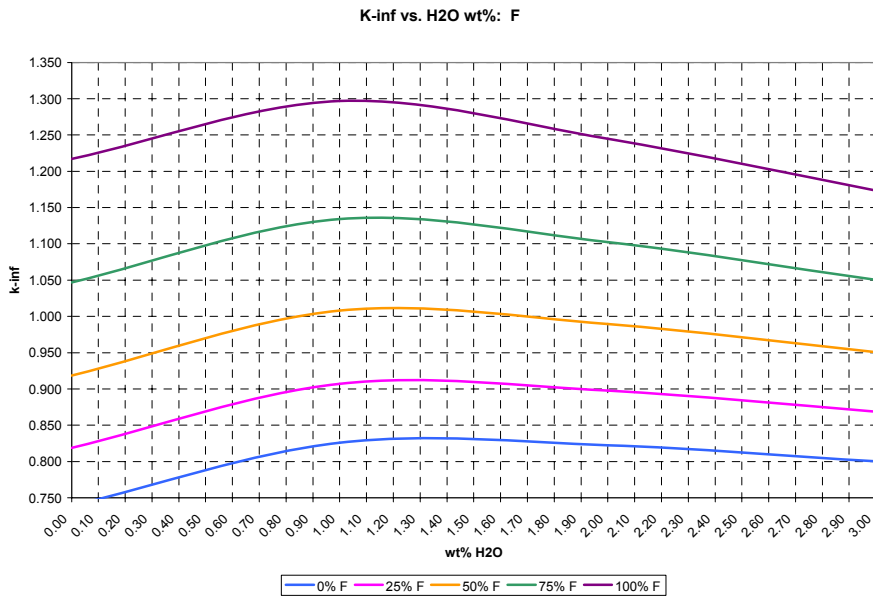
Figure 8. k_{\infty} as a function of water mass concentration (wt%) in an infinite \text{SiO}_2 waste matrix containing uranium enriched to 10% ^{235}\text{U} at the Condition 1 concentration limit, for various fluorine impurity mass concentrations.
