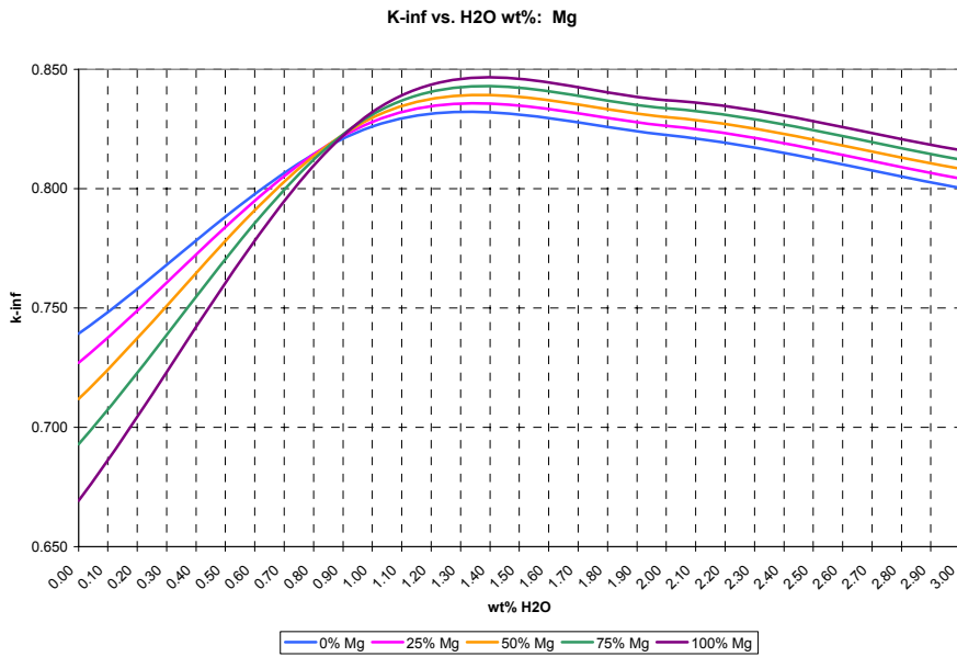
Figure 6. k_{\infty} as a function of water mass concentration (wt%) in an infinite \text{SiO}_2 waste matrix containing uranium enriched to 10% ^{235}\text{U} at the Condition 1 concentration limit, for various magnesium impurity mass concentrations.
