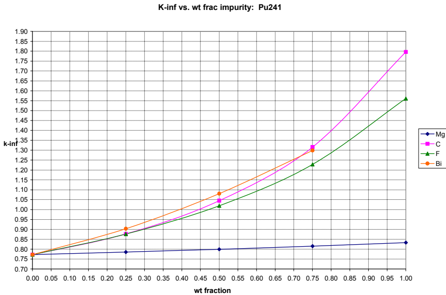
Figure 5. k_{\infty} as a function of Mg, C, F, and Bi impurity mass concentrations in an infinite \text{SiO}_2 waste matrix containing plutonium-241 at the Condition 1 concentration limit
