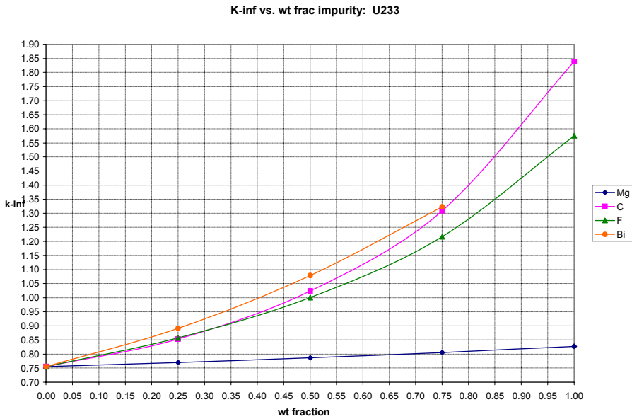
Figure 3. k_{\infty} as a function of Mg, C, F, and Bi impurity mass concentrations in an infinite \text{SiO}_2 waste matrix containing uranium-233 at the Condition 1 concentration limit
