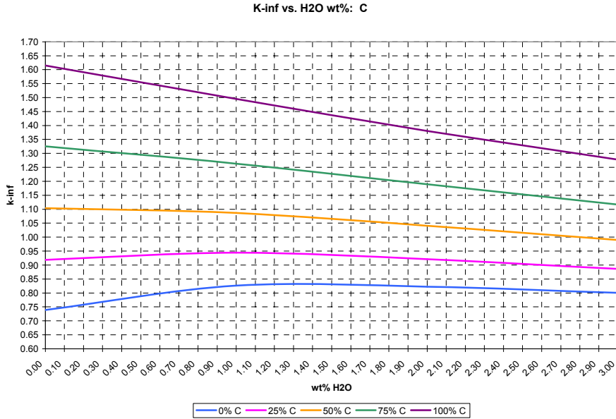
Figure 7. k_{\infty} as a function of water mass concentration (wt%) in an infinite \text{SiO}_2 waste matrix containing uranium enriched to 10% ^{235}\text{U} at the Condition 1 concentration limit, for various carbon impurity mass concentrations.
