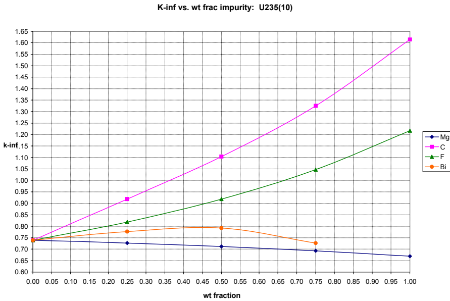
Figure 2. k_{\infty} as a function of Mg, C, F, and Bi impurity mass concentrations in an infinite \text{SiO}_2 waste matrix containing uranium enriched to 10% ^{235}\text{U} at the Condition 1 concentration limit
