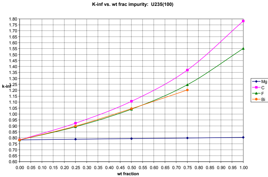
Figure 1. k_{\infty} as a function of Mg, C, F, and Bi impurity mass concentrations in an infinite \text{SiO}_2 waste matrix containing uranium enriched to 100% ^{235}\text{U} at the Condition 1 concentration limit
