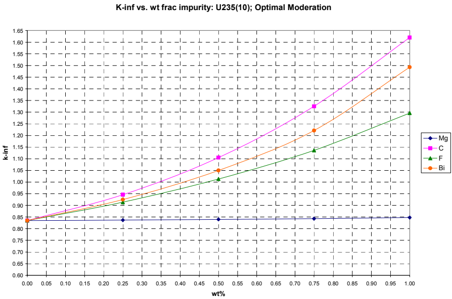
Figure 10. k_{\infty} as a function of impurity mass concentrations at the optimal water mass concentration in an infinite \text{SiO}_2 waste matrix containing uranium enriched to 10% ^{235}\text{U} at the Condition 1 concentration limit.
