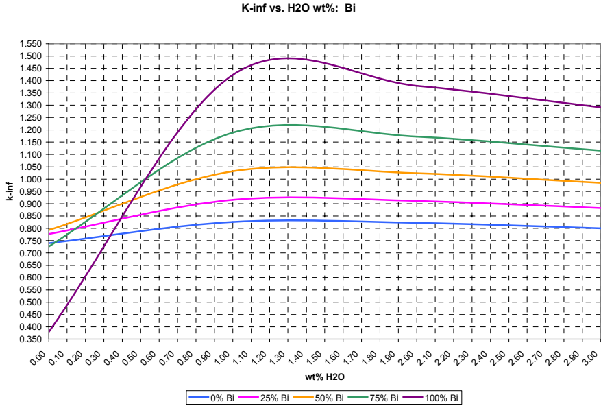
Figure 9. k_{\infty} as a function of water mass concentration (wt%) in an infinite \text{SiO}_2 waste matrix containing uranium enriched to 10% ^{235}\text{U} at the Condition 1 concentration limit, for various bismuth impurity mass concentrations.
