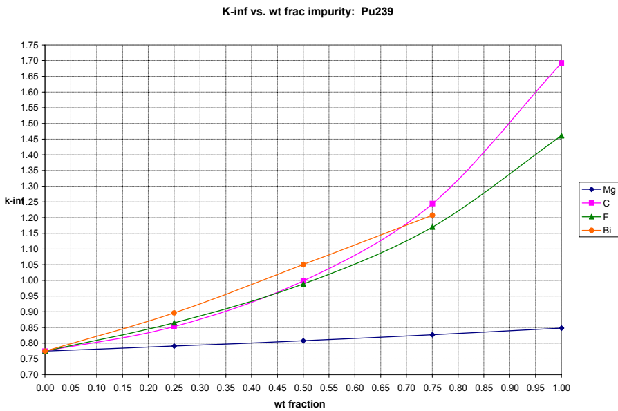
Figure 4. k_{\infty} as a function of Mg, C, F, and Bi impurity mass concentrations in an infinite \text{SiO}_2 waste matrix containing plutonium-239 at the Condition 1 concentration limit
