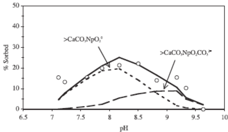
Fig. 10. Np sorption to calcite at 0.03% CO 2 (g) at 24 hours (○). Lines present total and individual species SC model fits.
