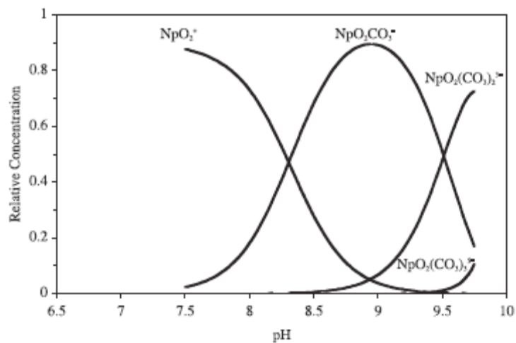
Fig. 3. Speciation of Np(V) at 0.03% \text{CO}_2(\text{g}) , I = 0.1 , and calcite saturation conditions.
