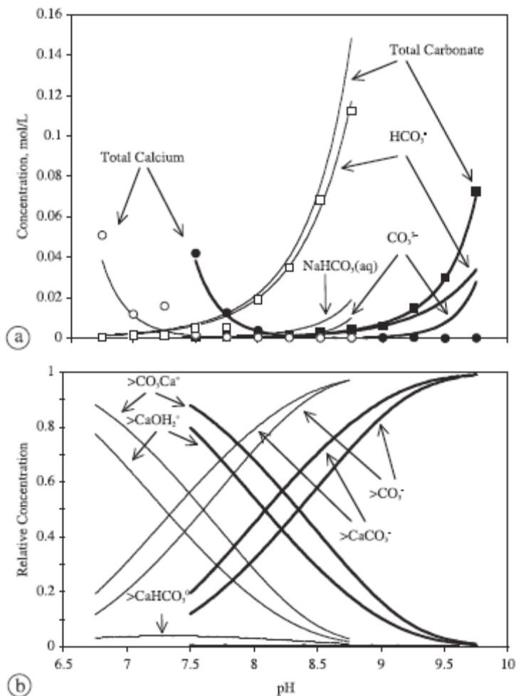
Fig. 1. Predominant (a) aqueous and (b) surface species at calcite saturation conditions. I = 0.1 and 0.03% \text{CO}_2(\text{g}) (thick lines) or 1% \text{CO}_2(\text{g}) (thin lines). \circ and \square represent typical batch solution total calcium and carbonate alkalinity results, respectively (0.03% \text{CO}_2(\text{g}) = filled symbols, 1% \text{CO}_2(\text{g}) = open symbols).
