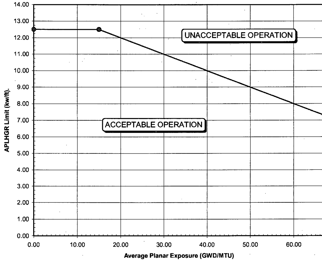
Figure 5 APLHGR Limits for all ATRIUM-10™ Fuel (A10)
