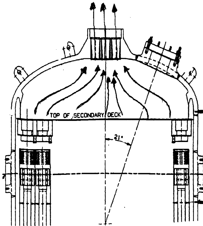
Ginna Steam Separators
