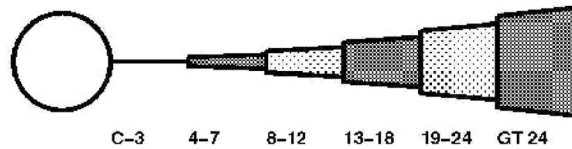
FIGURE 2.7-74 Rev. 0 CCNPP 33' AUGUST PRECIPITATION WIND ROSE FOR RATE CLASS 0.2-0.3 in/hr CCNPP UNIT 3 ER
