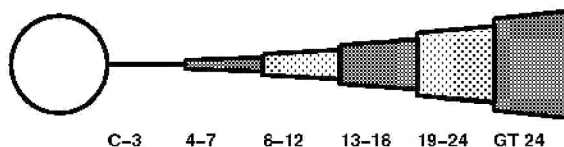
FIGURE 2.7-85 Rev. 0 CCNPP 33' SEPTEMBER PRECIPITATION WIND ROSE FOR RATE CLASS 0.6-0.7 in/hr CCNPP UNIT 3 ER
