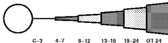
FIGURE 2.7-30 Rev. 0 CCNPP 33' JANUARY PRECIPITATION WIND ROSE FOR RATE CLASS 0.0-0.1 in/hr CCNPP UNIT 3 ER
