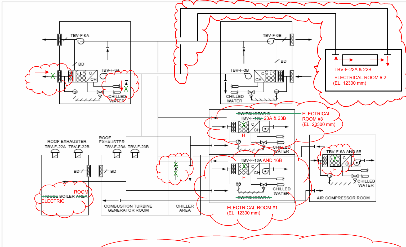
Figure 9.4-2c Electrical Building HVAC System Diagram
