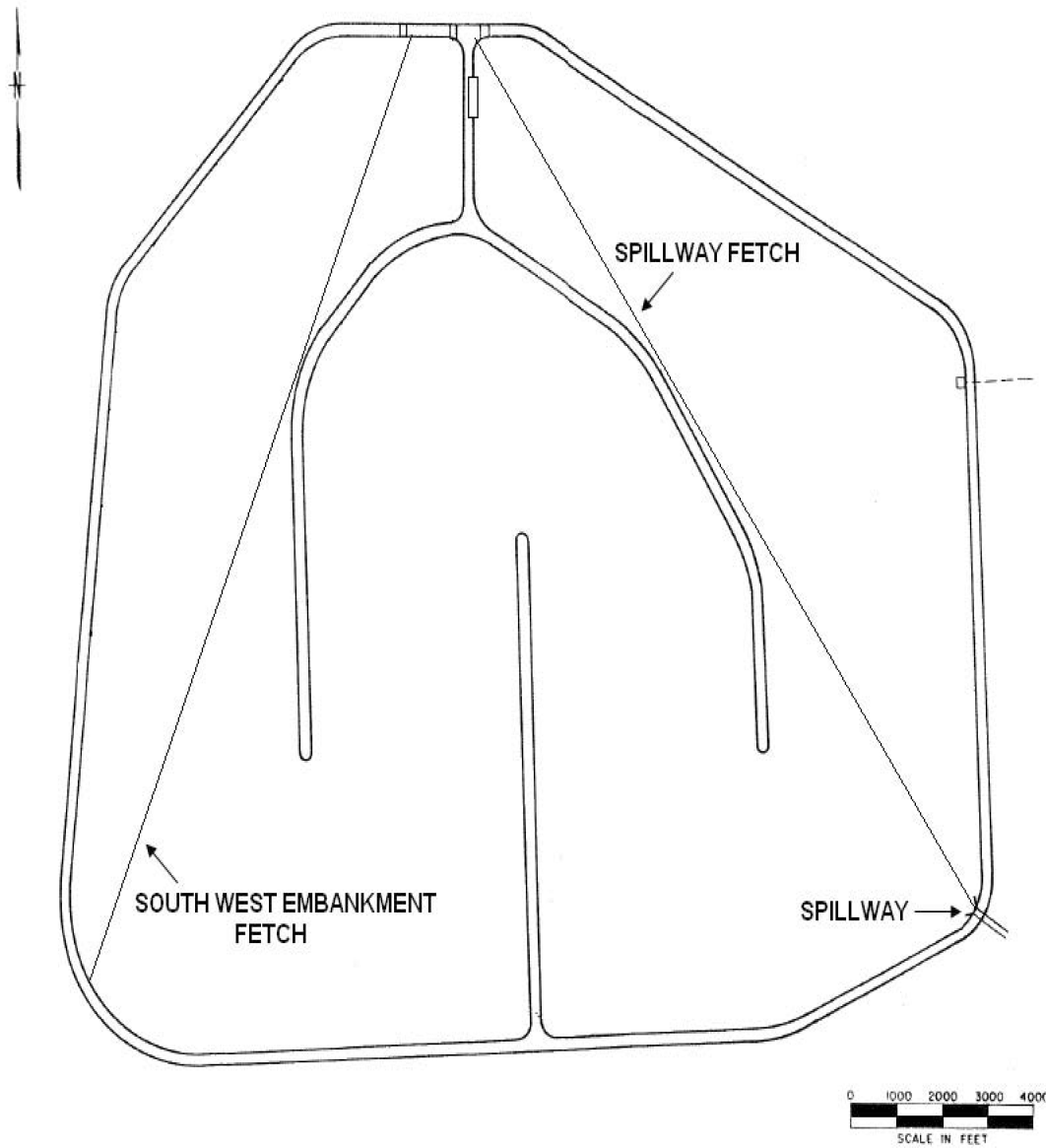
Figure 2.4S.8-4 Determination of Fetch at the Spillway and at the South West Embankment
