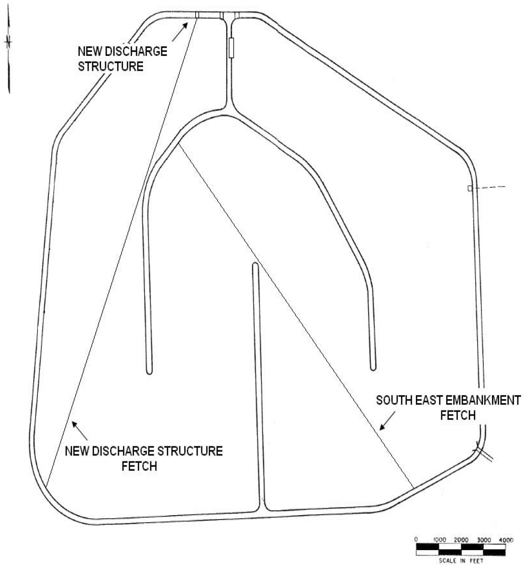
Figure 2.4S.8-5 Determination of Fetch at the Southeast Embankment and at the New Discharge Structure
