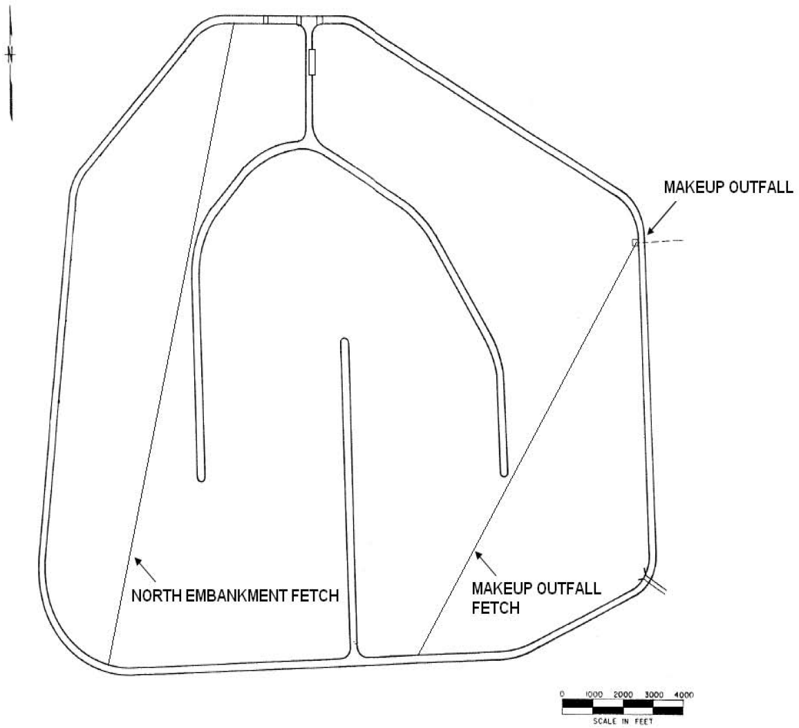
Figure 2.4S.8-3 Determination of Fetch at the Makeup Outfall and at the North Embankment
