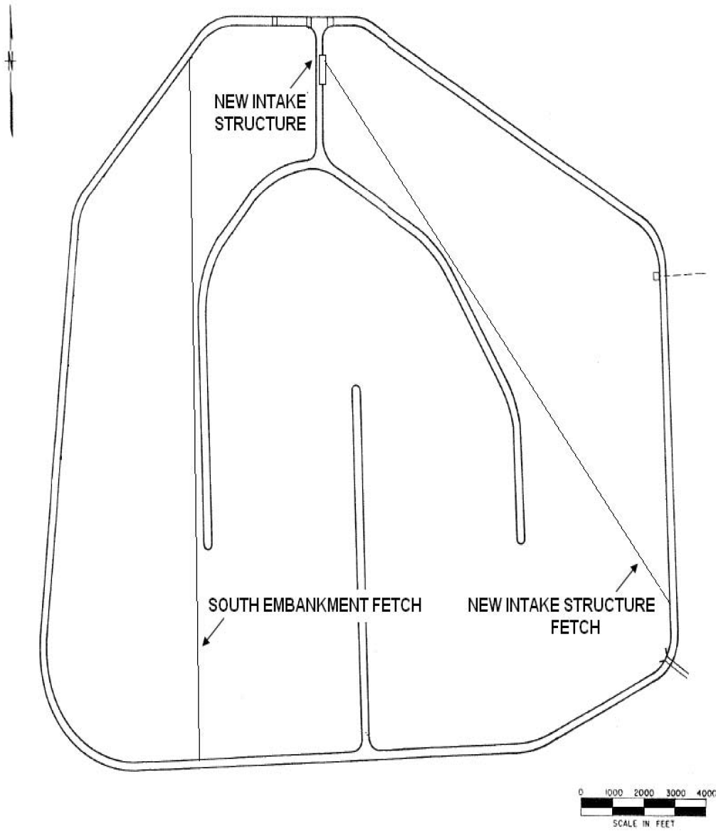
Figure 2.4S.8-2 Determination of Fetch at the New Intake Structure and at the South Embankment
