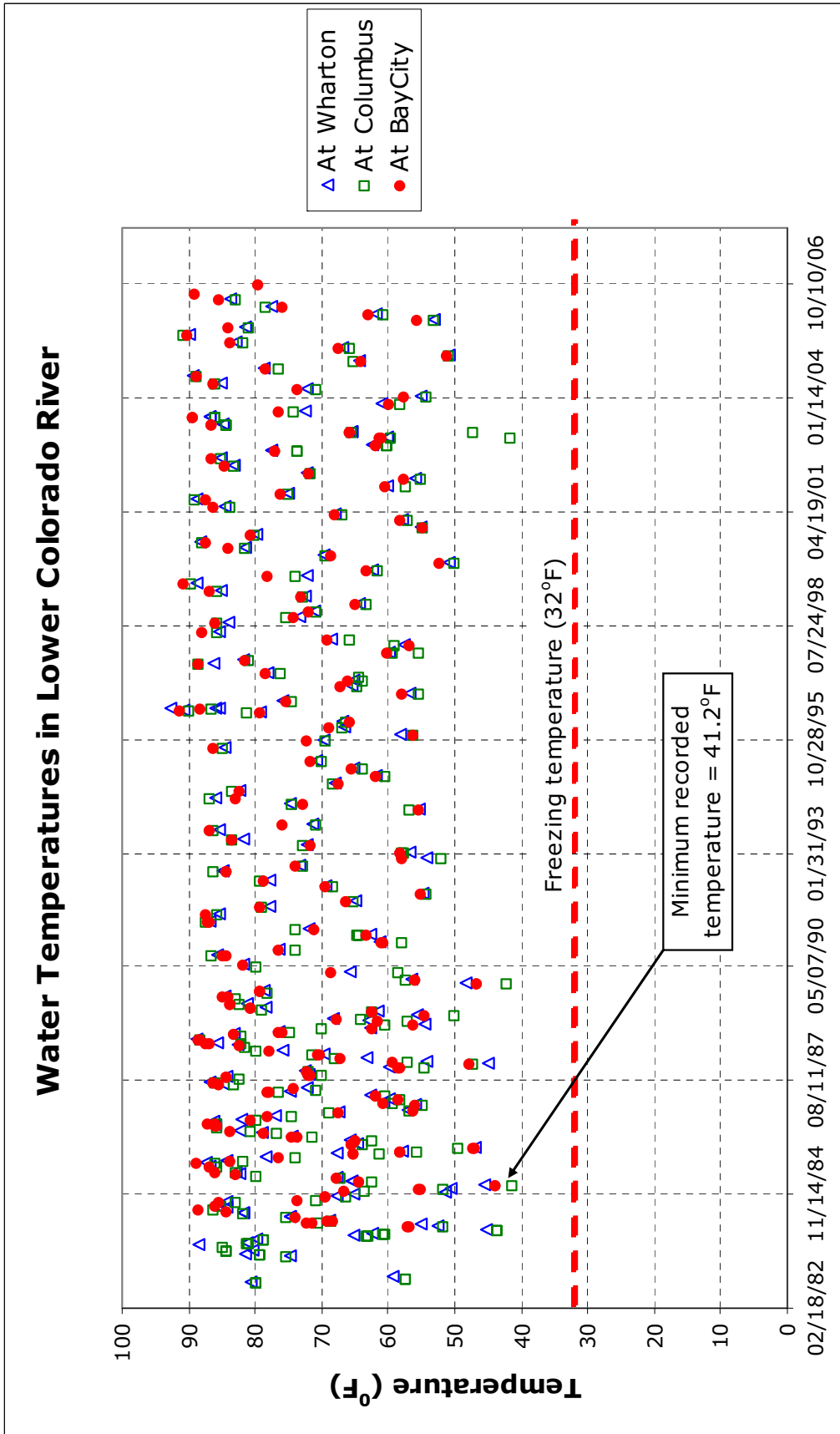
Figure 2.4S.7-1 Recorded Water Temperatures in Lower Colorado River
