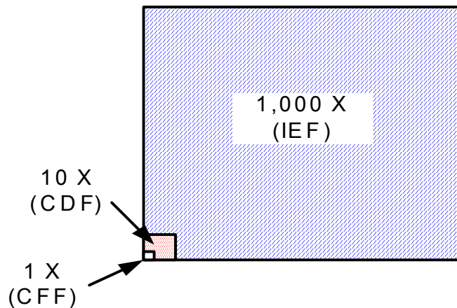
Figure 3.6 - Relative magnitudes of Initiating Event Frequency (IEF), Core Damage Frequency (CDF), and Containment Failure Frequency (CFF) for LOSP and LOCAs based on NUREG-1150 site risk analysis reports for the Surry, Sequoyah, Grand Gulf and Peach Bottom reactors.
