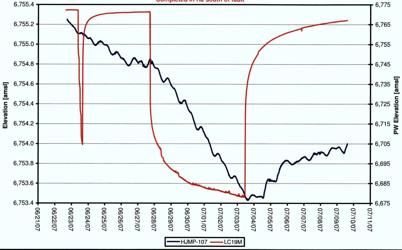
Figure 6-7 Lost Creek Regional Aquifer Test - North Test Completed in HJ south of fault
