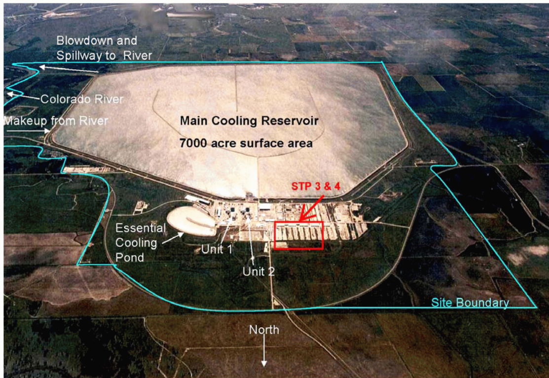
Figure 3.1-4 Aerial Photograph of STP 1 & 2 With Proposed Location of STP 3 & 4
