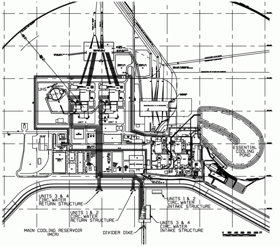
Figure 3.1-3 General Plant Layout
