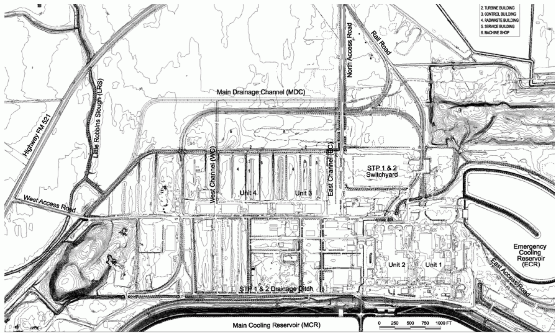
Figure 3.1-6 Topographical Map of the Site and Vicinity
