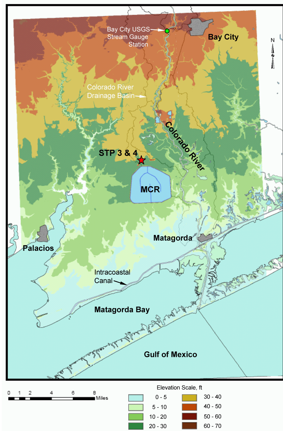
Figure 2.3.1-1 Site Map of STP 3 & 4
