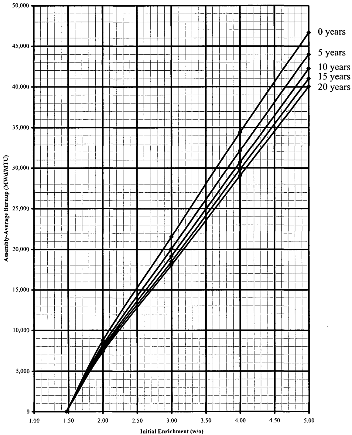
Figure 5-13. Minimum Required Fuel Assembly Burnup versus Initial 235 U Enrichment for the "3-out-of-4" Storage Configuration
