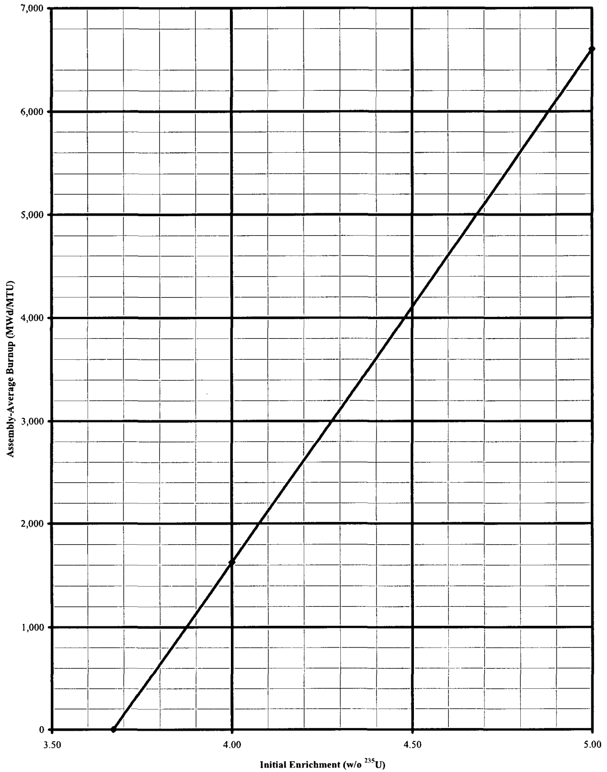
Figure 5-15. Minimum Required Fuel Assembly Burnup versus Initial 235 U Enrichment for the "2-out-of-4" Storage Configuration
