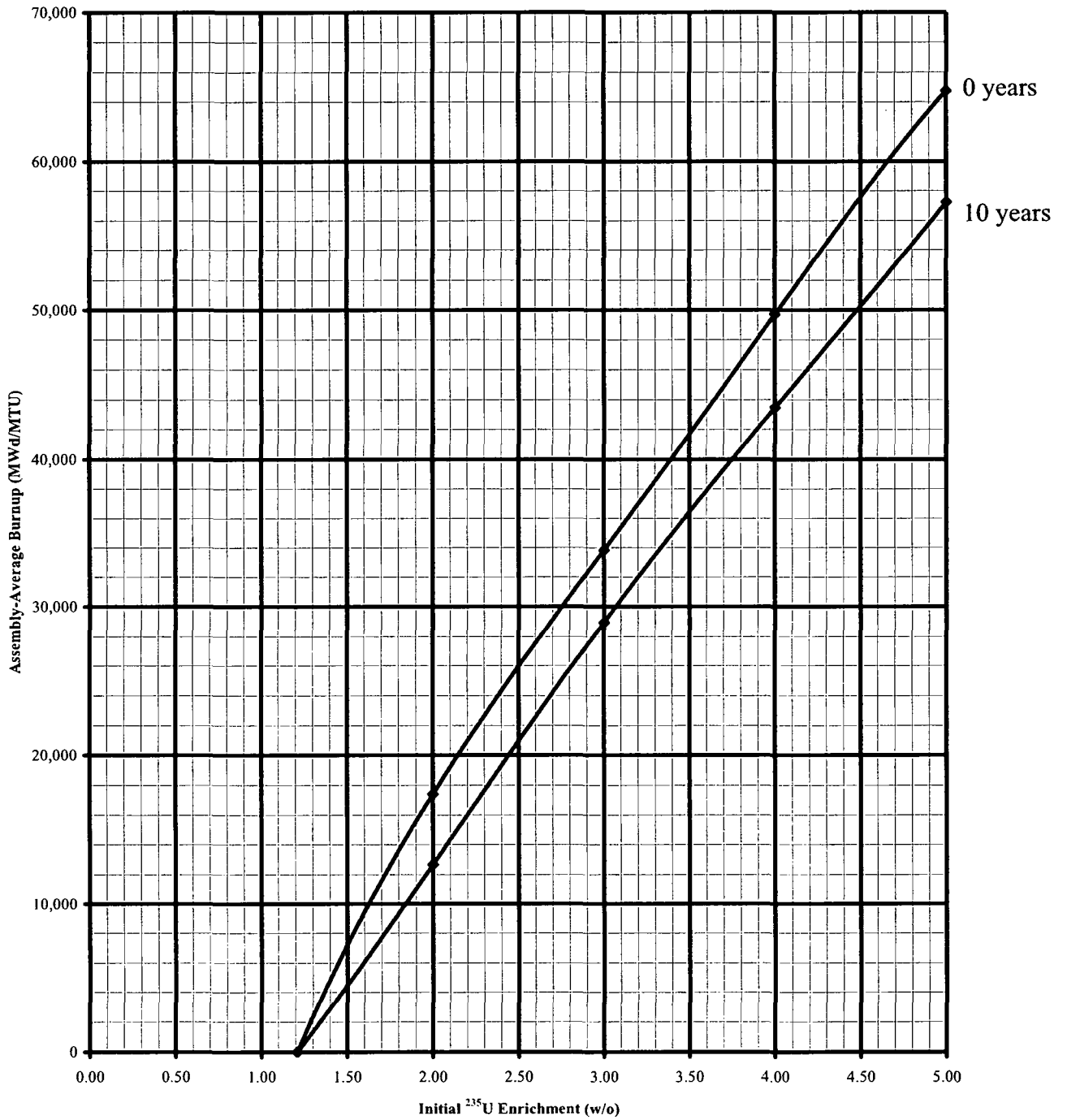
Figure 5-9. Minimum Required Fuel Assembly Burnup versus Initial 235 U Enrichment for the "4-out-of-4 with 1 RCCA" Storage Configuration
