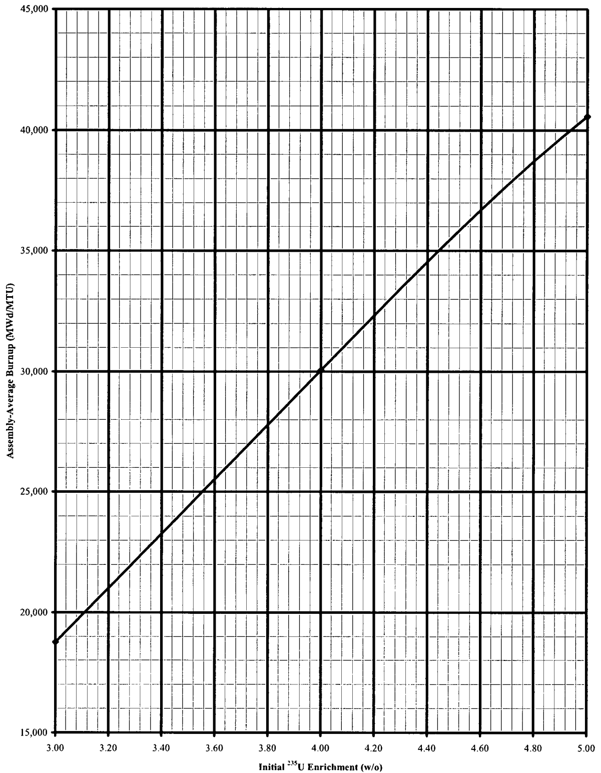
Figure 5-12. Minimum Required Fuel Assembly Burnup versus Initial 235 U Enrichment for the "4-out-of-4 with 3 RackSavers and Axial Blankets" Storage Configuration
