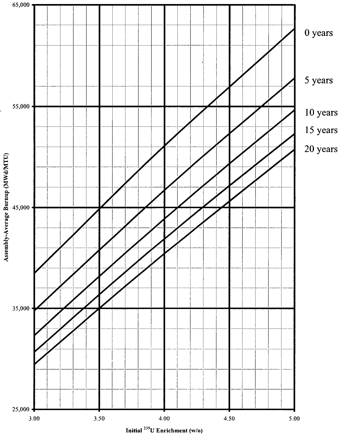
Figure 5-8. Minimum Required Fuel Assembly Burnup versus Initial 235 U Enrichment for the "4-out-of-4 with Axial Blankets" Storage Configuration
