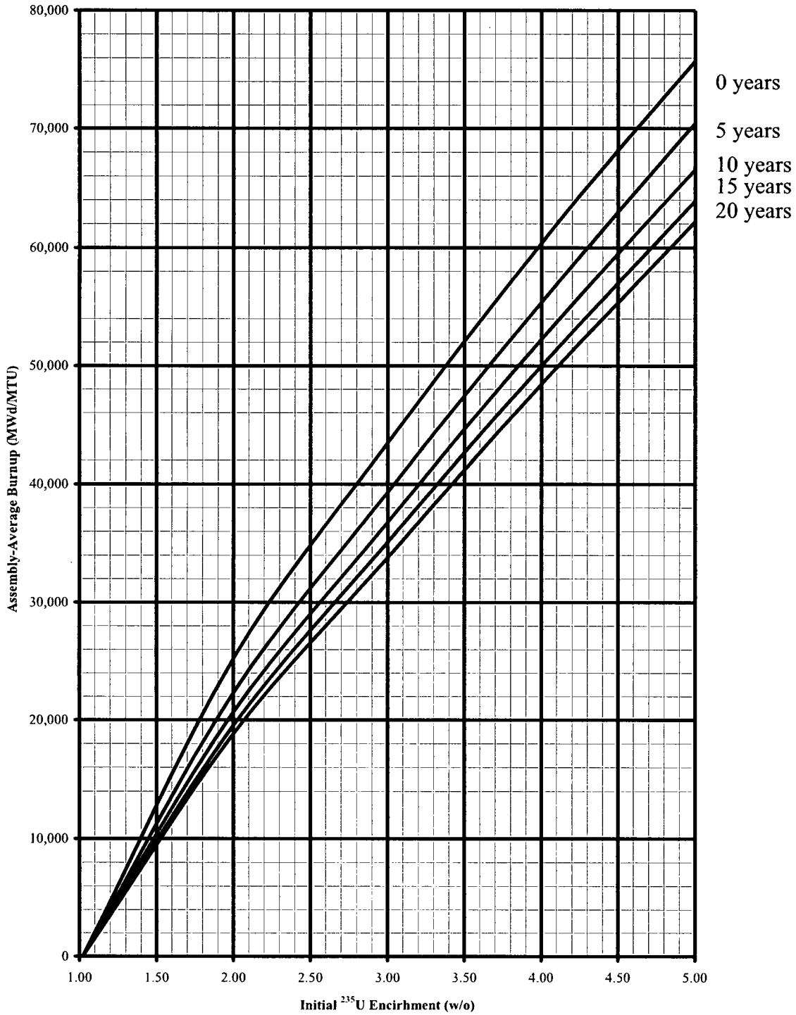
Figure 5-7. Minimum Required Fuel Assembly Burnup versus Initial 235 U Enrichment for the "4-out-of-4" Storage Configuration
