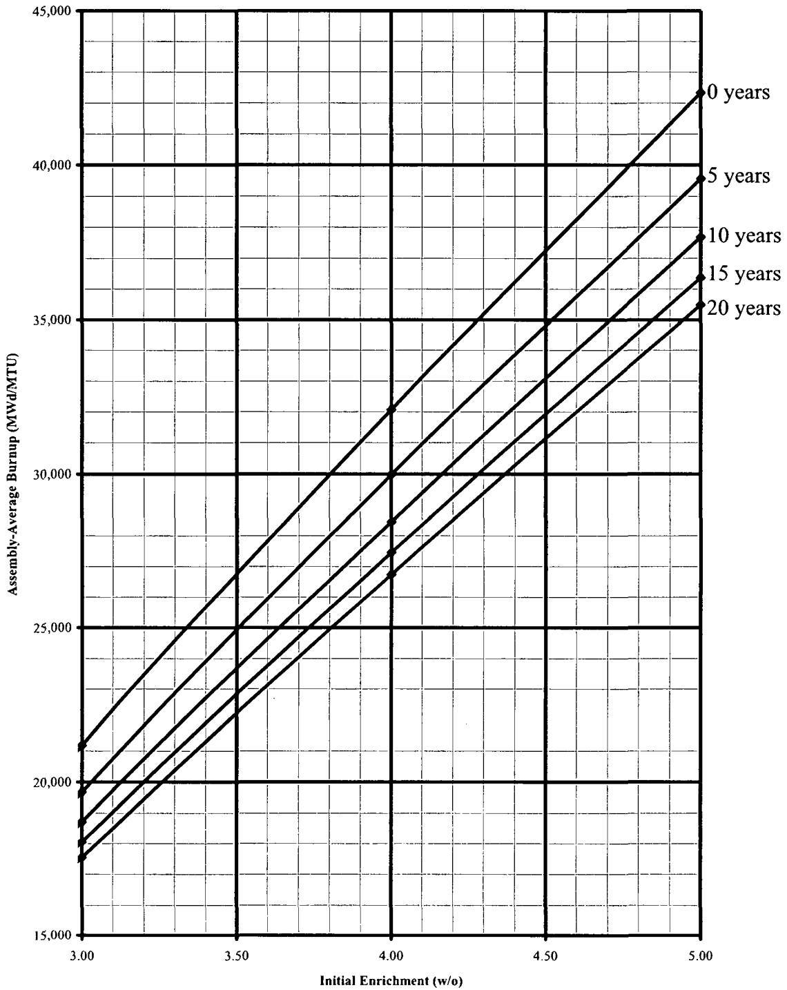
Figure 5-14. Minimum Required Fuel Assembly Burnup versus Initial 235 U Enrichment for the "3-out-of-4 with Axial Blankets" Storage Configuration
