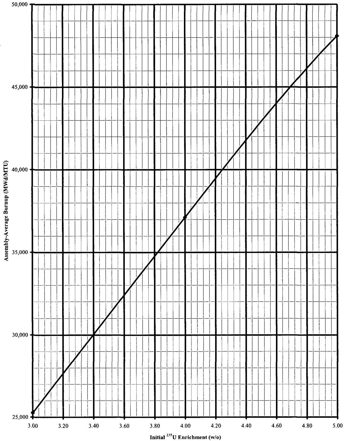
Figure 5-11. Minimum Required Fuel Assembly Burnup versus Initial 235 U Enrichment for the "4-out-of-4 with 2 RackSavers and Axial Blankets" Storage Configuration
