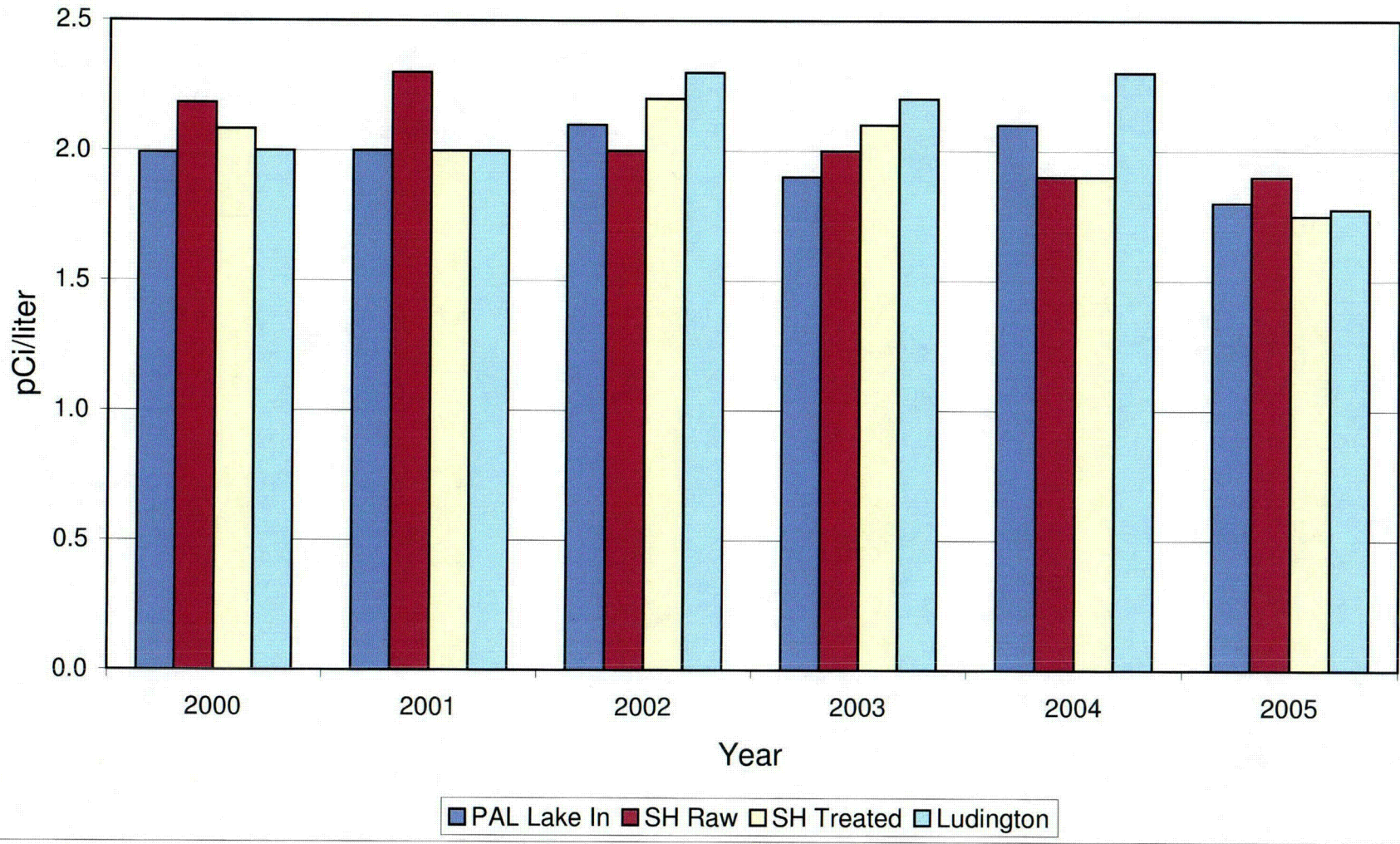
Lake Water Gross Beta 2000 to 2005
