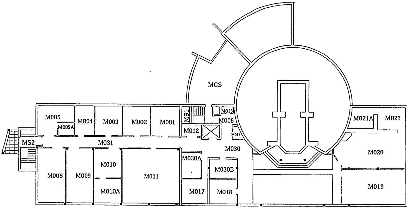
Figure 2-5 UVA Reactor Mezzanine Floor Plan View
