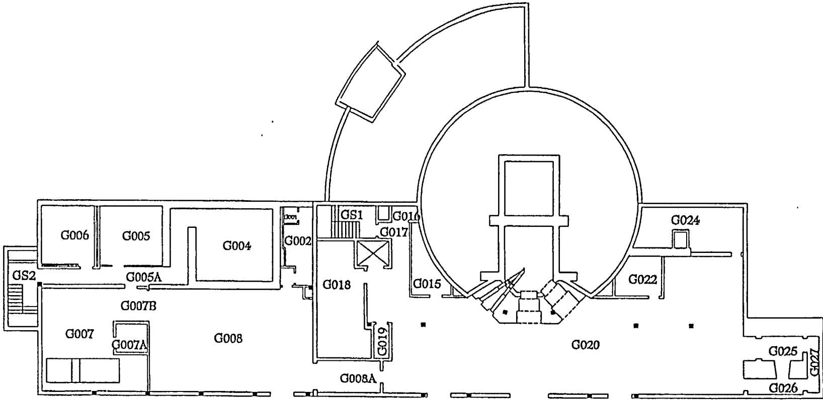
Figure 2-6 UVA Reactor Ground Floor Plan View
