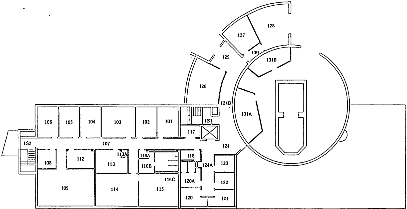
Figure 2-4 UVA Reactor First Floor Plan View
