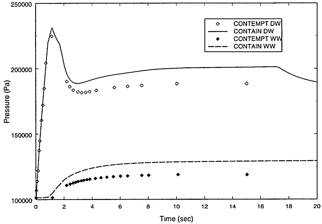
Figure 4-1. Comparison of CONTAIN and CONTEMPT predictions for the Grand Gulf recirculation line break scenario.
