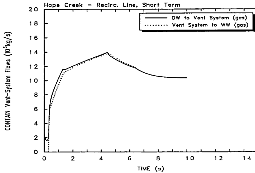
Figure 2-5. CONTAIN mass flow rates from the drywell to the vent system and from the vent system to the wetwell for the Hope Creek recirculation line break short-term scenario.
