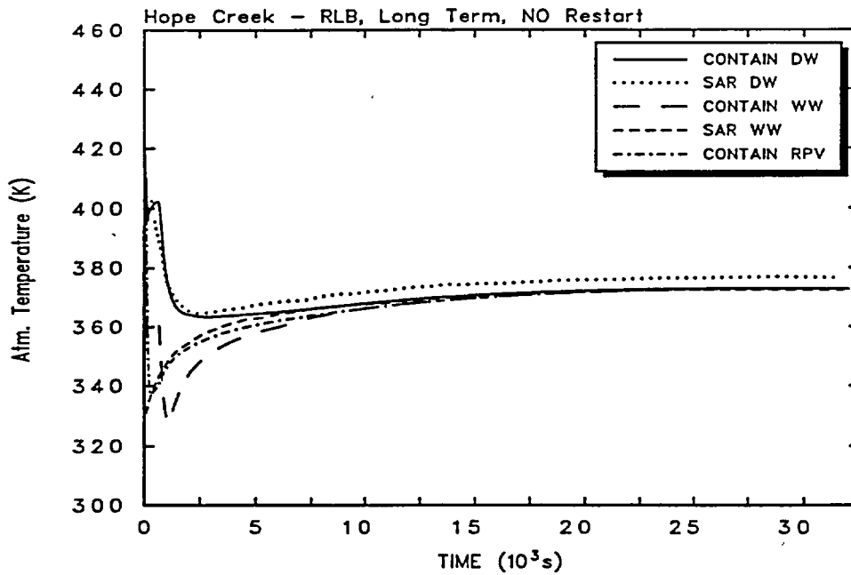
Figure 2-9. CONTAIN (no restart) and SAR drywell and wetwell atmosphere temperatures for the Hope Creek recirculation line break Case C long-term analysis. The CONTAIN RPV-cell atmosphere temperature also is presented.
