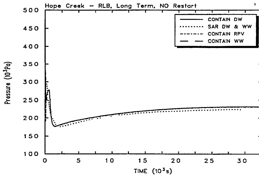
Figure 2-8. CONTAIN (no restart) and SAR drywell and wetwell pressures for the Hope Creek recirculation line break Case C long-term analysis. The CONTAIN RPV-cell pressure also is presented.
