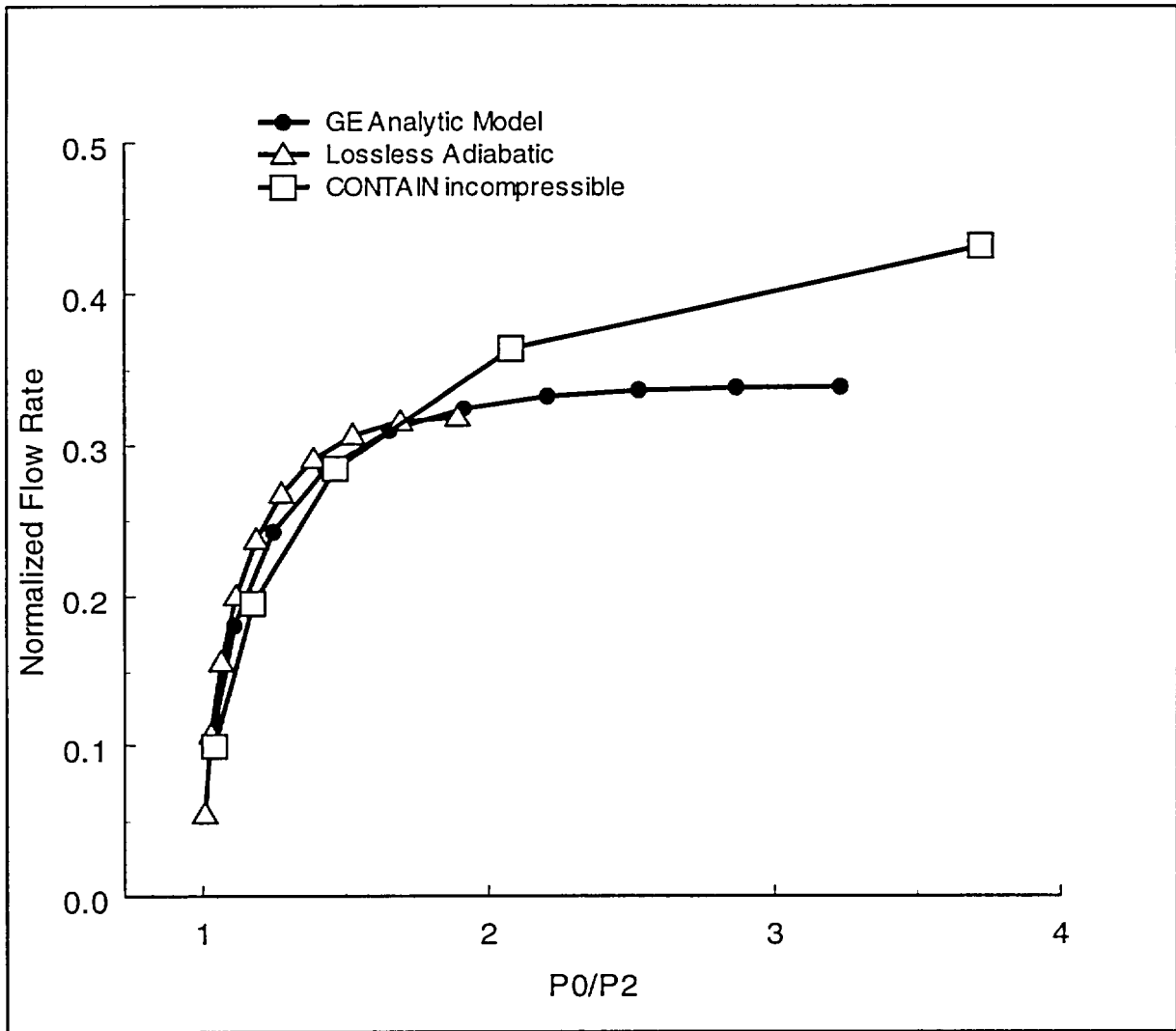
Figure B-5. Comparison of CONTAIN and GE Flow Rates as a function of Upstream to Downstream Pressure Ratio ( P_0/P_2 ), for \nu = 0.55 and K = 3 * 1.4 .
