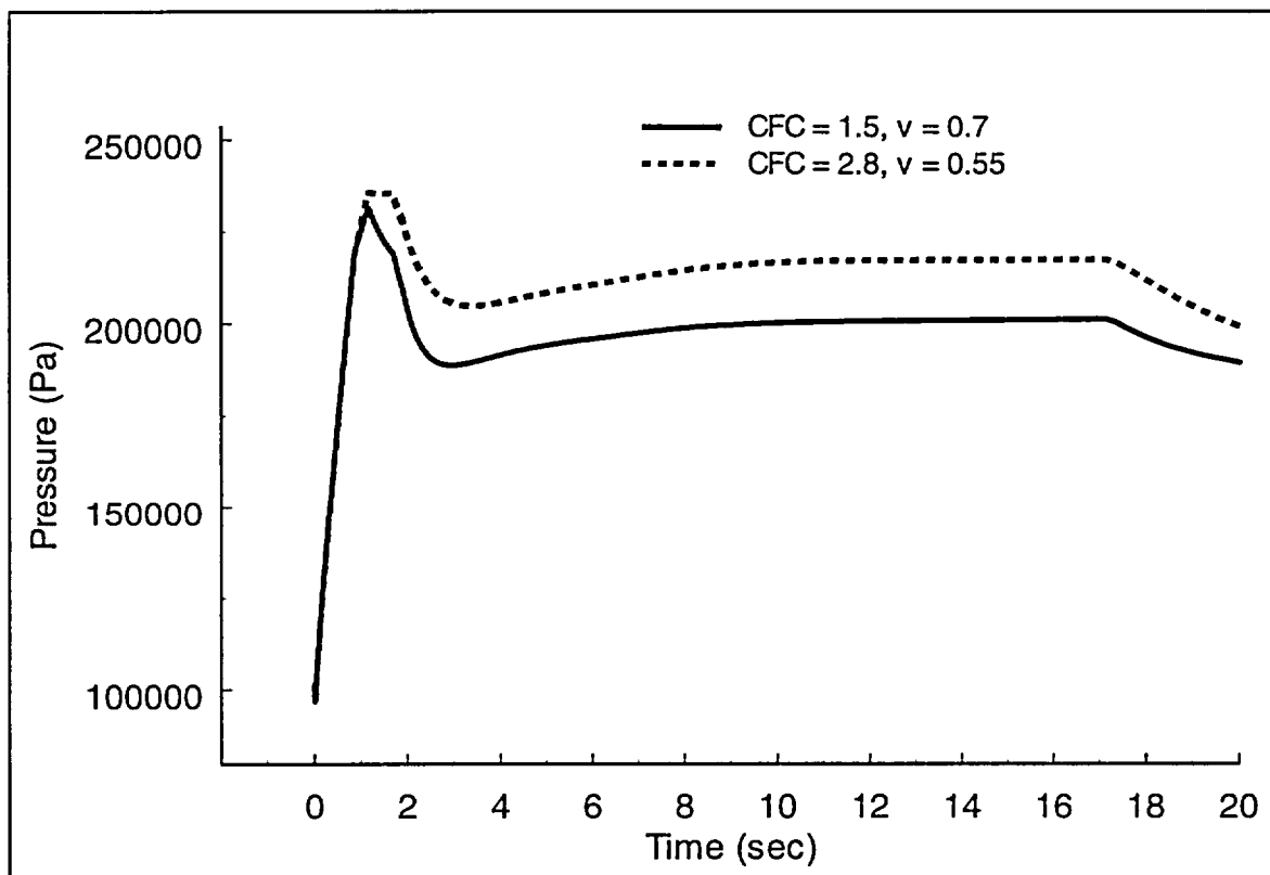
Figure 4-4. CONTAIN sensitivity calculations for the Grand Gulf recirculation line break scenario, where input for the gas vents between the downcomer and wetwell are varied to account for two-phase and compressibility effects.
