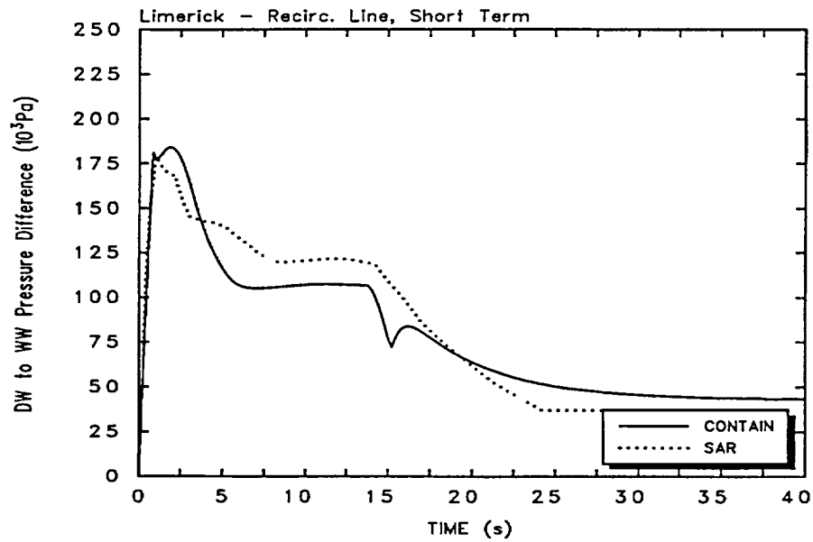
Figure 3-4. CONTAIN and SAR Drywell to Wetwell Pressure Difference for the Limerick Recirculation Line Break Short-Term Scenario.
