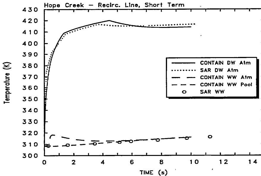
Figure 2-3. CONTAIN and SAR drywell and wetwell temperatures for the Hope Creek recirculation line break short-term scenario.
