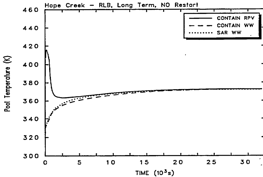
Figure 2-10. CONTAIN (no restart) and SAR wetwell pool temperatures for the Hope Creek recirculation line break Case C long-term analysis. The CONTAIN RPV-cell pool temperature also is presented.
