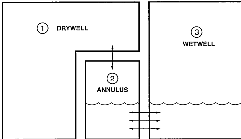
Figure 4-2. CONTAIN three-cell model of a Mark III BWR.
