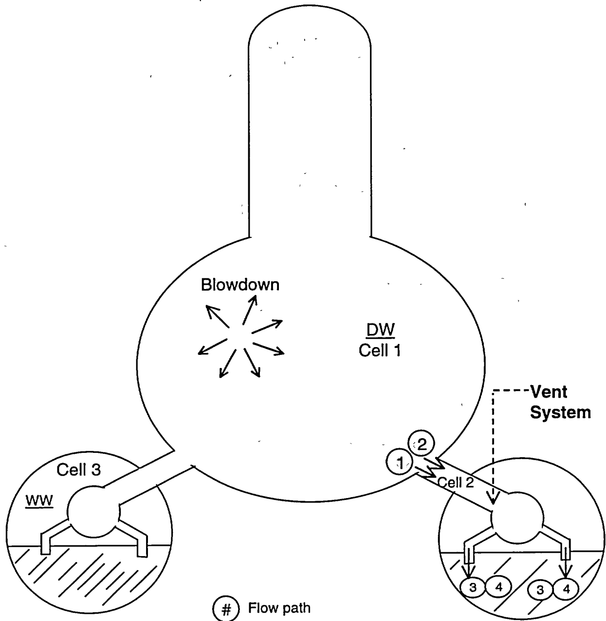
Figure 2-7. CONTAIN Mark I BWR model showing the drywell cell, the vent system cell, the wetwell cell and the flow paths for the Hope Creek recirculation line break short-term scenario.
