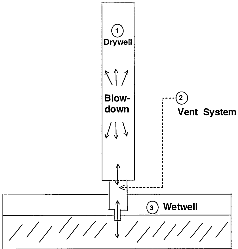
Figure 2-6. Basic CONTAIN three-cell model of a Mark I BWR for the Hope Creek recirculation line break short-term scenario. For additional details, see Figure 2-7.
