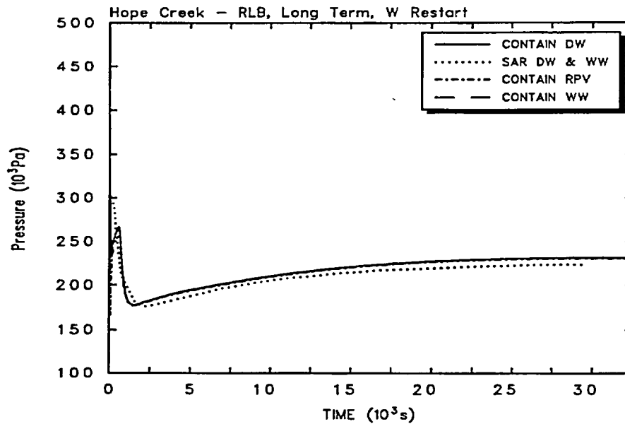
Figure 2-12. CONTAIN (With Restart) and SAR drywell and wetwell pressures for the Hope Creek recirculation line break Case C long-term analysis. The CONTAIN RPV-cell pressure also is presented.
