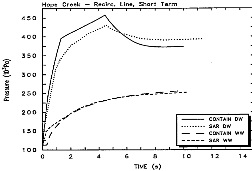
Figure 2-2. CONTAIN and SAR drywell and wetwell pressures for the Hope Creek recirculation line break short-term scenario.
