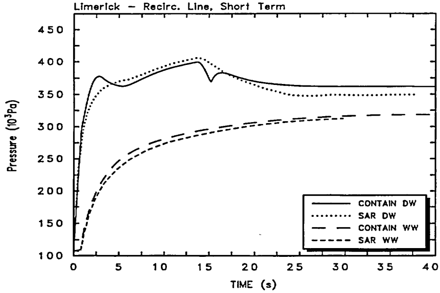
Figure 3-2. CONTAIN and SAR Drywell and Wetwell Pressures for the Limerick Recirculation Line Break Short-Term Scenario.
