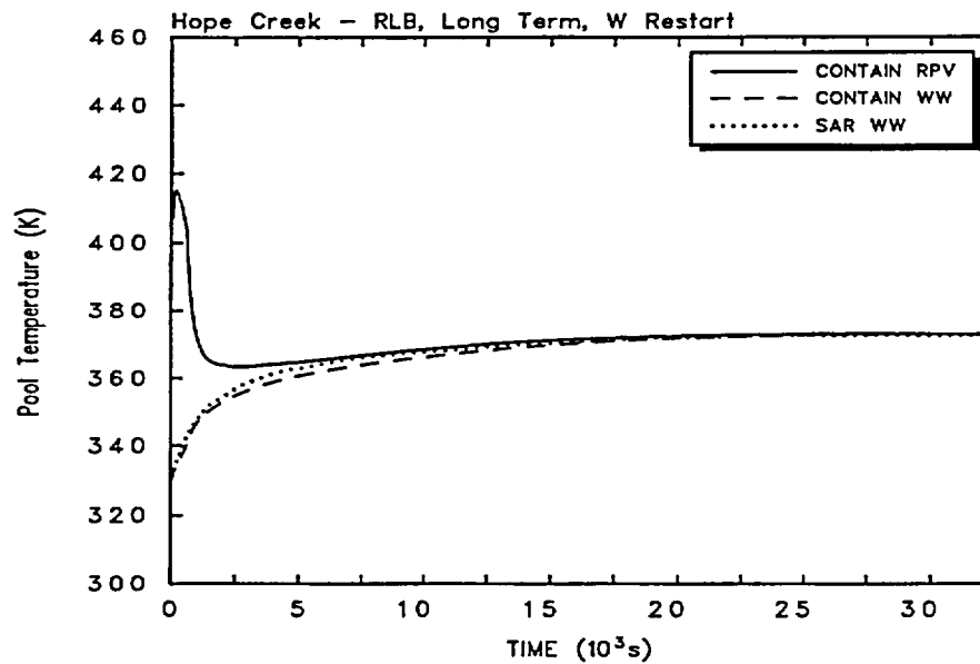
Figure 2-13. CONTAIN (With Restart) and SAR wetwell pool temperature for the Hope Creek Mark I BWR recirculation line break, Case C, long-term analysis. The CONTAIN RPV-cell pool temperature also is presented.
