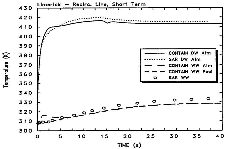
Figure 3-3. CONTAIN and SAR Drywell and Wetwell Temperatures for the Limerick Recirculation Line Break Short-Term Scenario.
