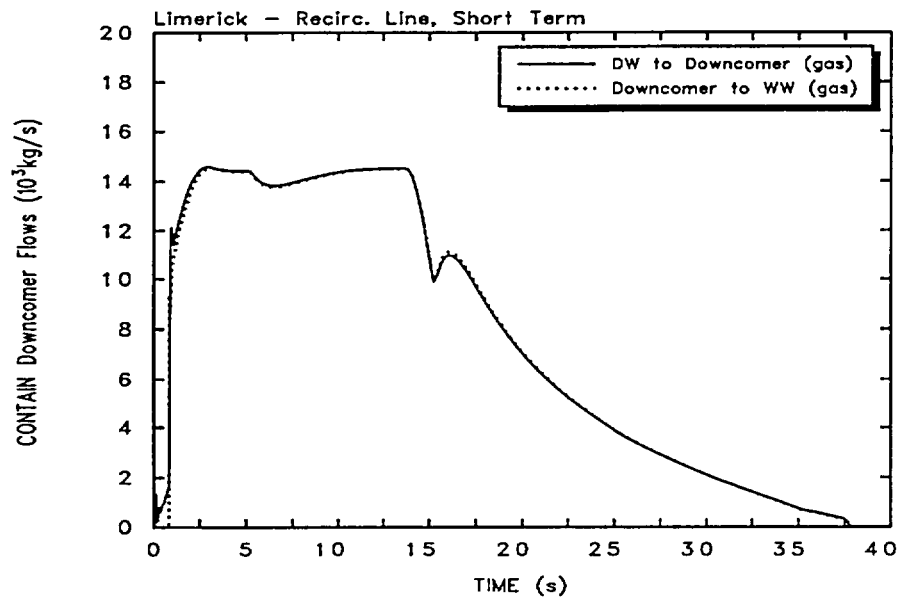
Figure 3-5. CONTAIN Mass Flow Rates from the Drywell to the Downcomer and from the Downcomer to the Wetwell for the Limerick Recirculation Line Break Short-Term Scenario.
