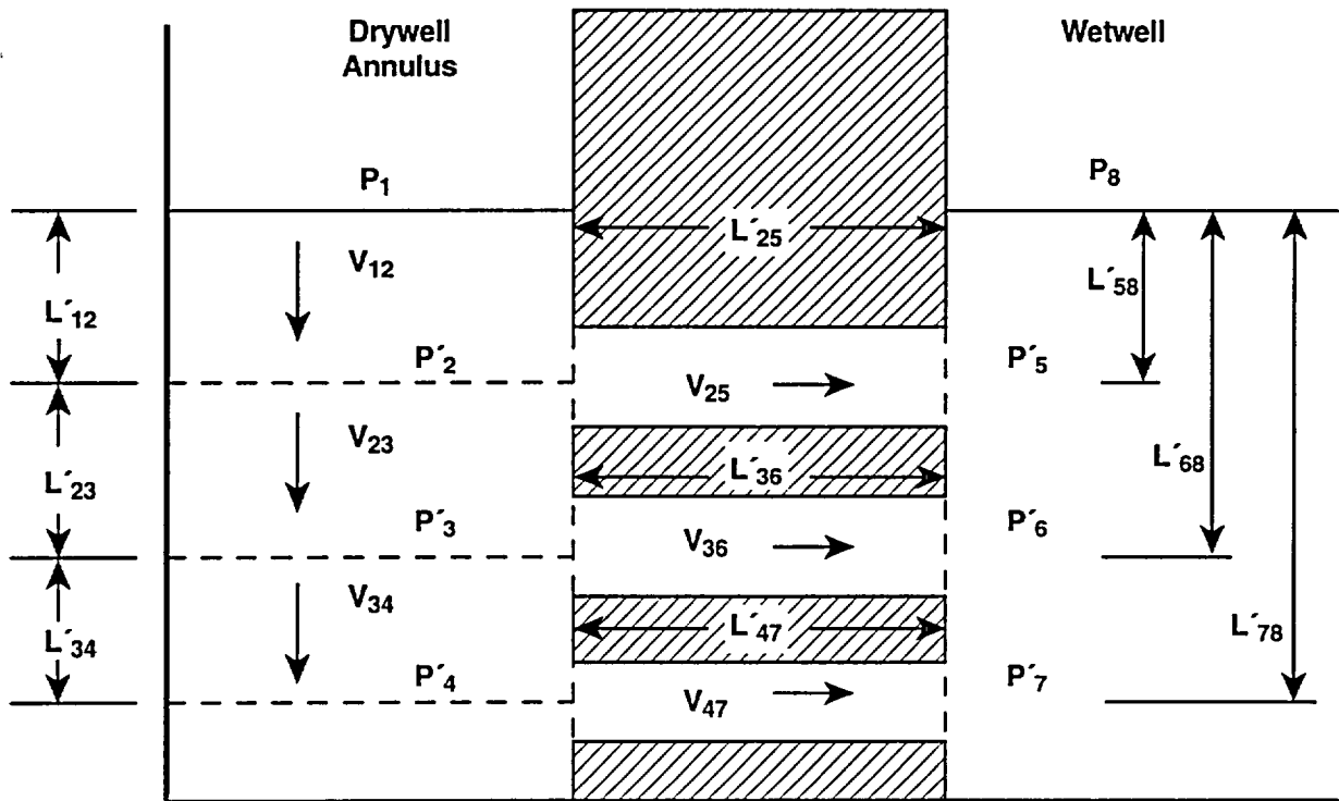
Figure G-1. Illustration of the Seven-Node Representation of Mark III Suppression Vents Used in the Inertial Lengths Derivation. Note that L'_{12} is the top vent submergence, L'_{23} is the vent centerline separation, and L'_{25} is the vent horizontal length.
