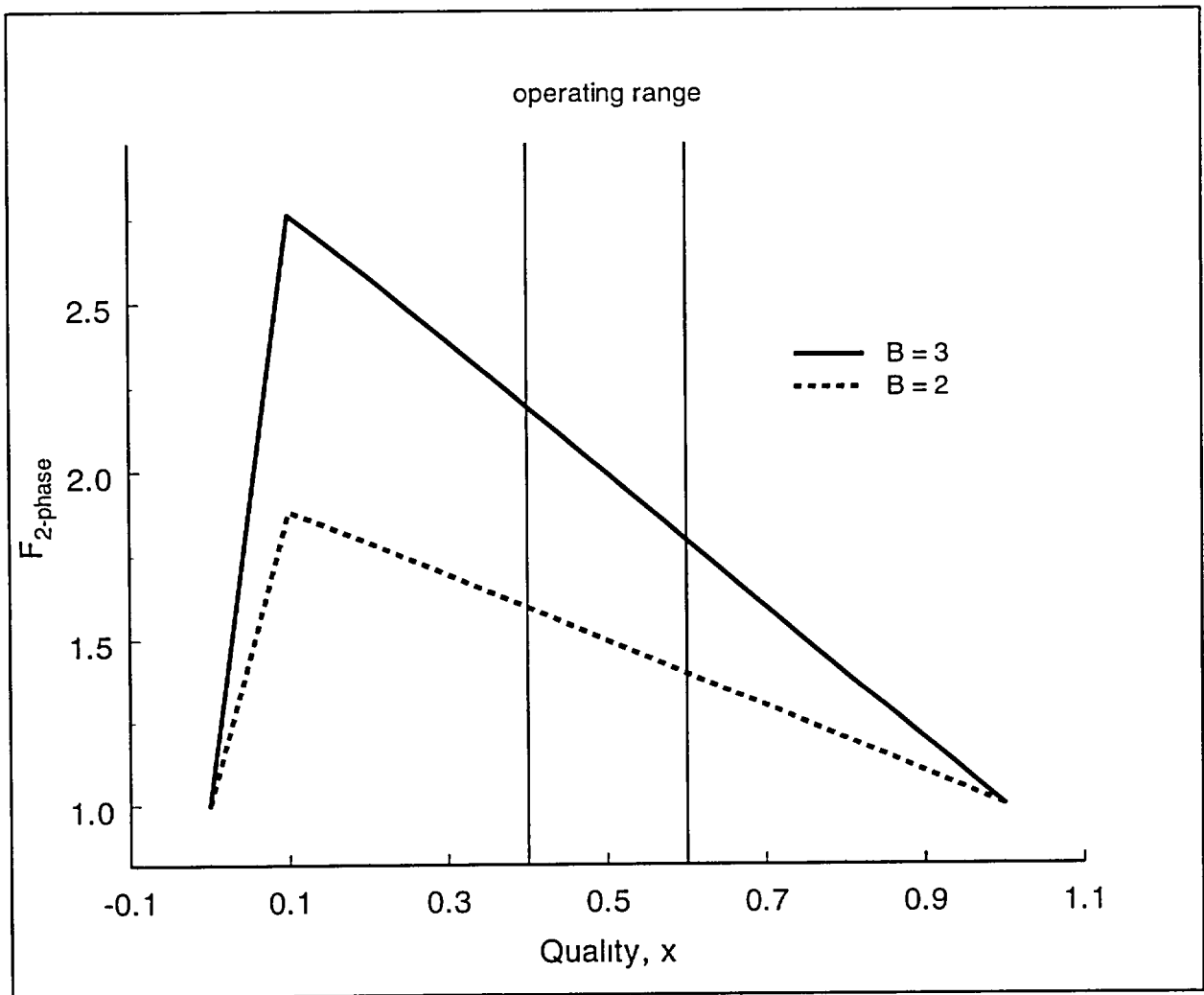
Figure B-2. Calculated two-phase loss factor F_{2-phase} for miter-bend using the B-type empirical correlation of Chisholm [3].
