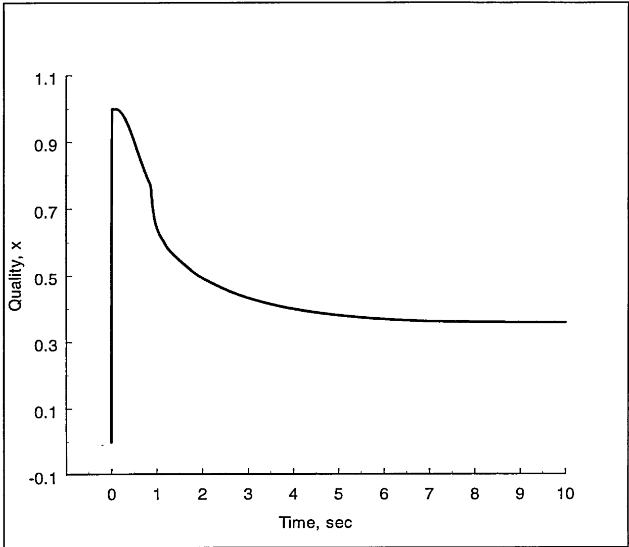
Figure B-1. CONTAIN calculated flow quality in the downcomer of the Grand Gulf plant during a recirculation line break event.
