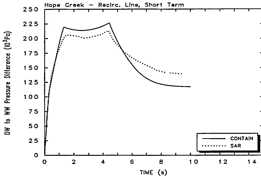
Figure 2-4. CONTAIN and SAR Drywell to Wetwell Pressure Difference for the Hope Creek Recirculation Line Break Short-Term Scenario.
