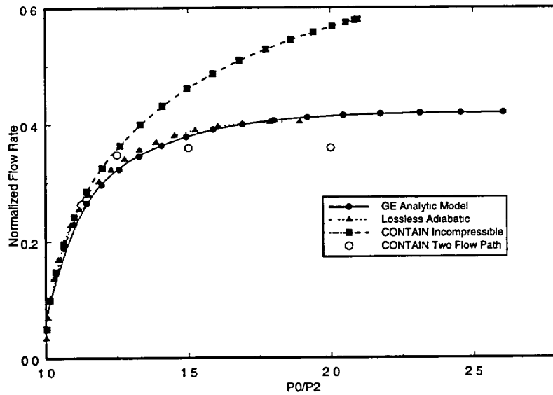
Figure B-3. Comparison of the CONTAIN and GE Analytic Model Flow Rates as a Function of the Upstream to Downstream Pressure Ratio ( P_0/P_2 ), for \nu = 0.7 and K = 1.23 .
