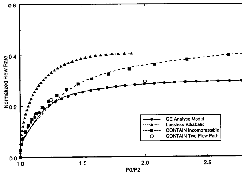
Figure B-4. Comparison of the CONTAIN and GE Analytic Model Flow Rates as a Function of the Upstream to Downstream Pressure Ratio ( P_0/P_2 ), for \nu = 0.7 and K = 4.6 .
