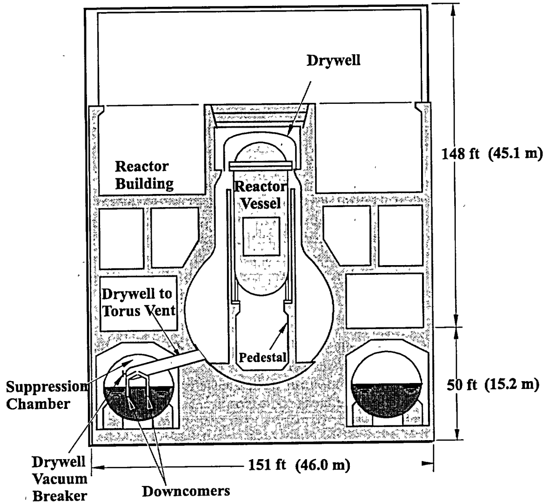
Figure 2-1 Mark I BWR containment showing the drywell, vent-system (vent and downcomers), and the wetwell.
