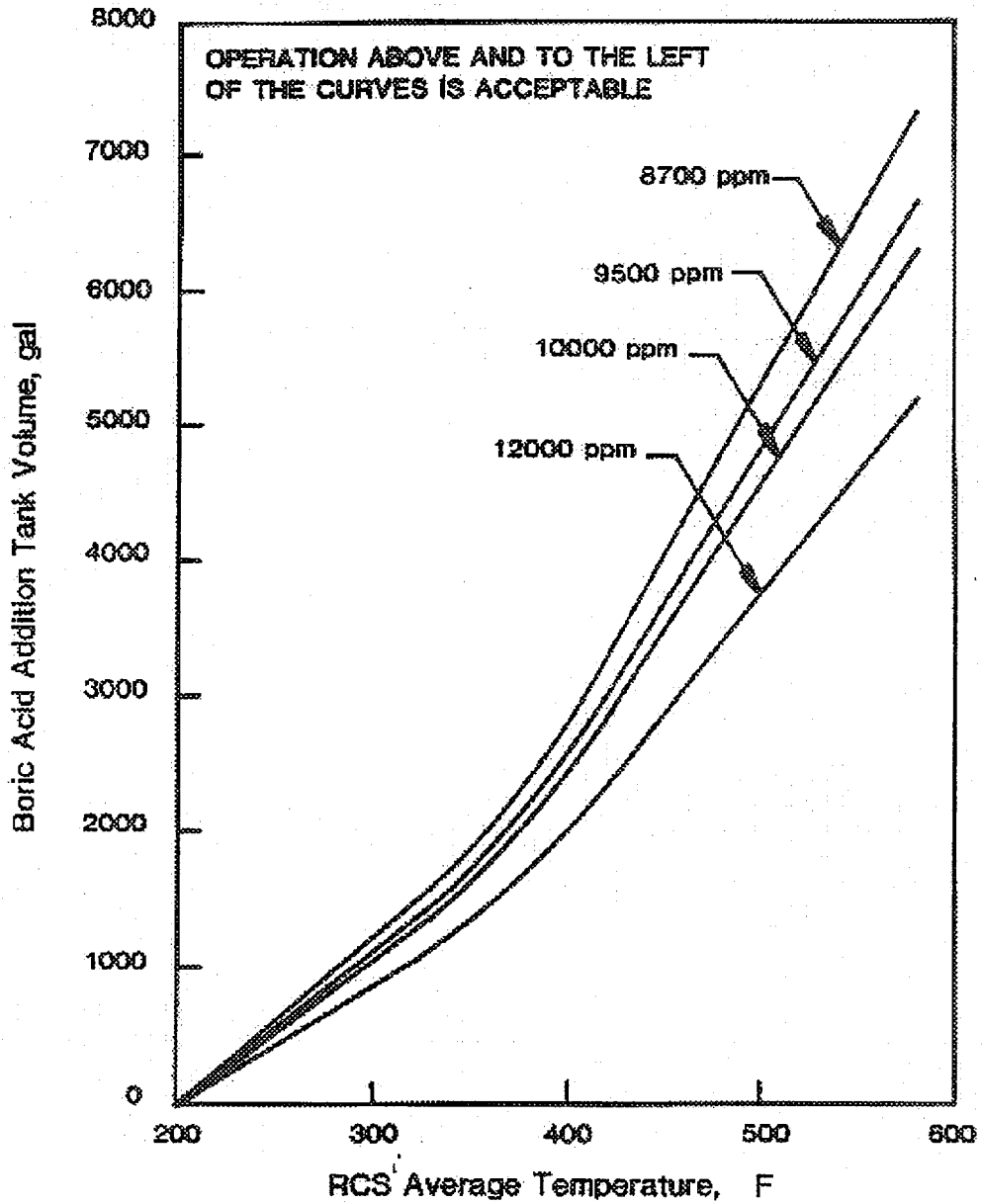
Boric Acid Addition Tank Volume and Concentration Vs RCS Average Temperature
