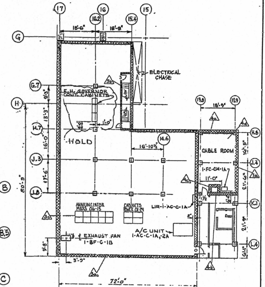
CABLE ROOM PLAN EL. 918'-0"
