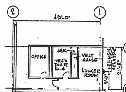
PART PLAN-MACHINE SHOP FLOOR EL. 918'-0"
