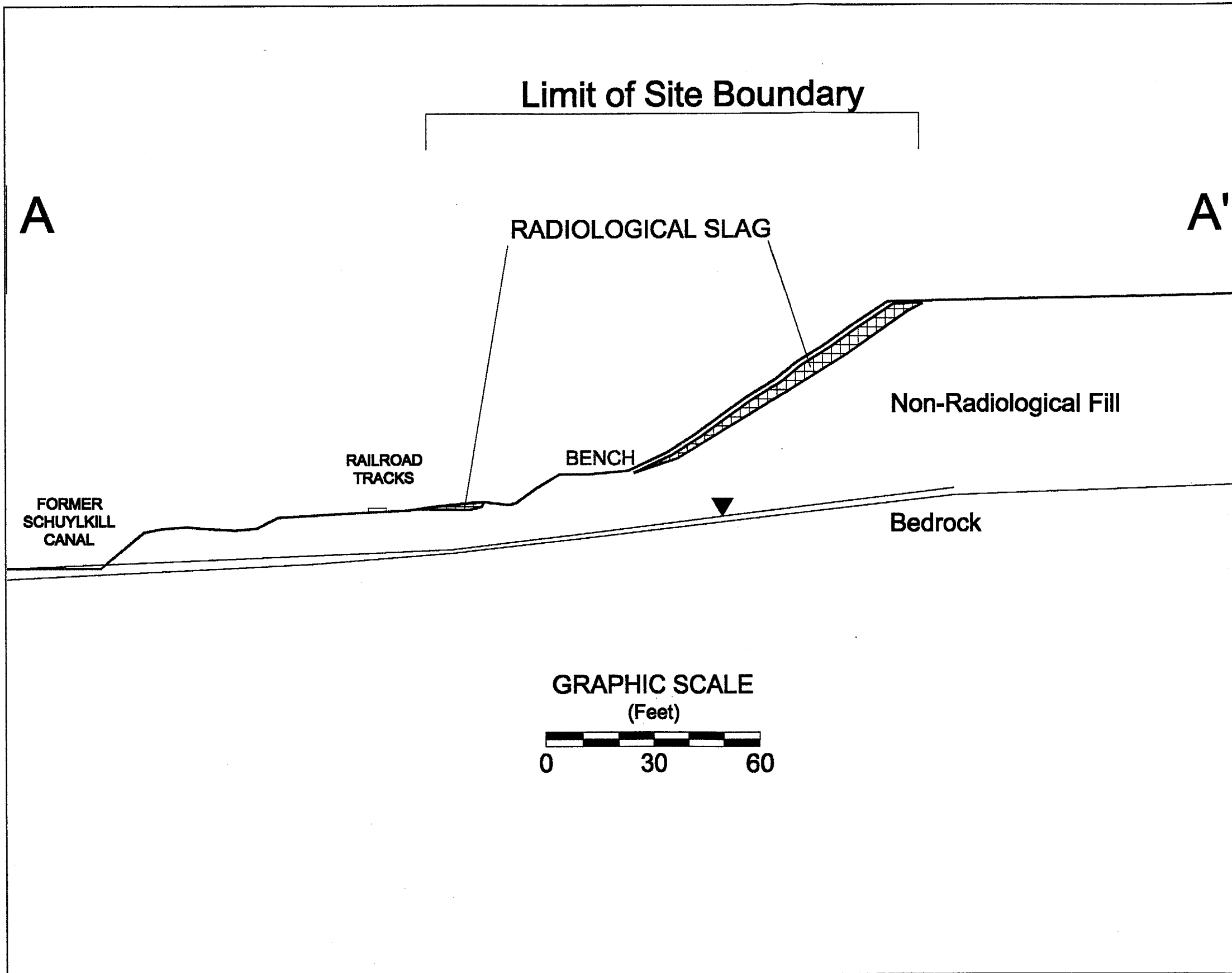
FIGURE 1-6 CROSS SECTION AA'
