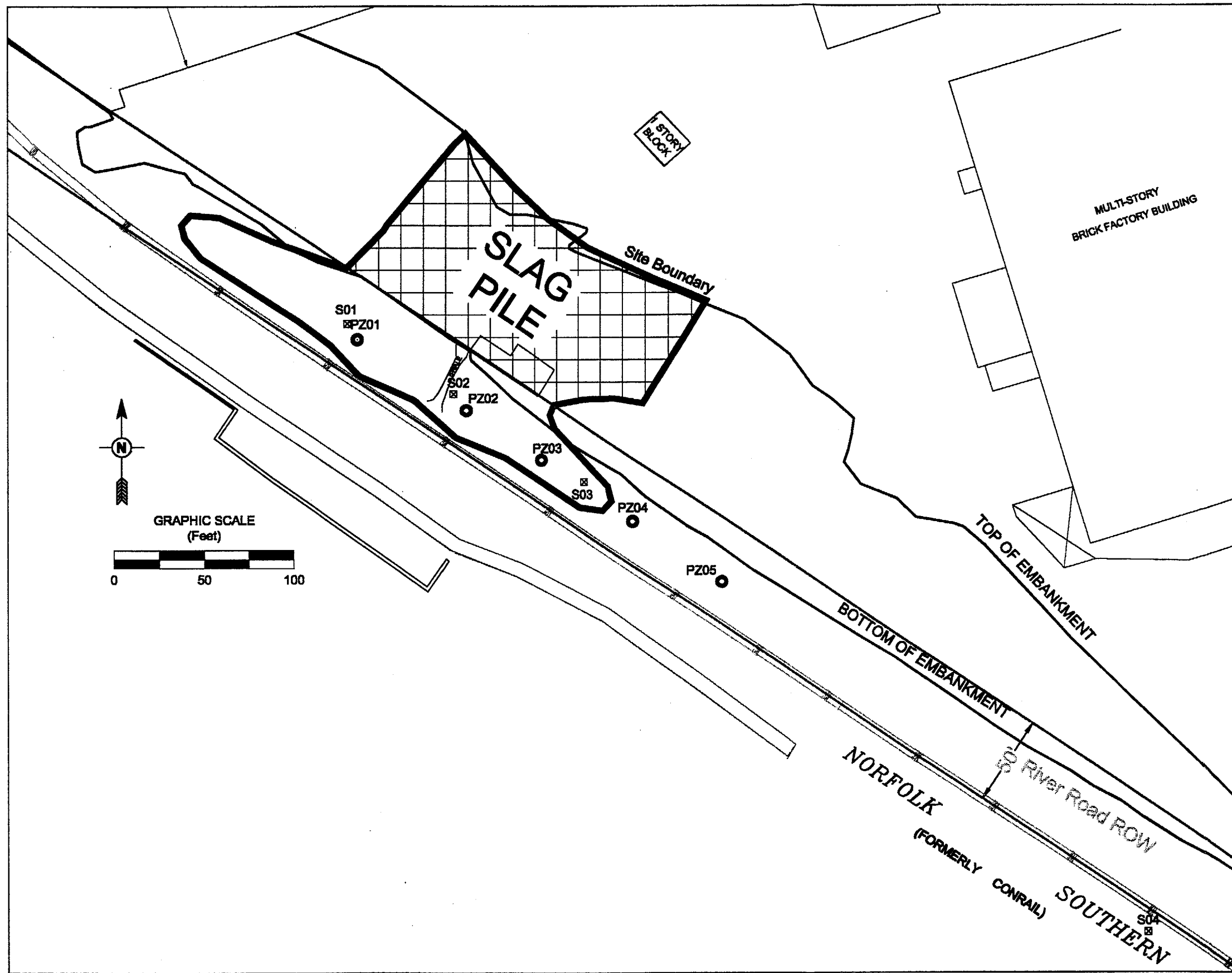
FIGURE 1-10 PIEZOMETER AND SOIL SAMPLING LOCATIONS
