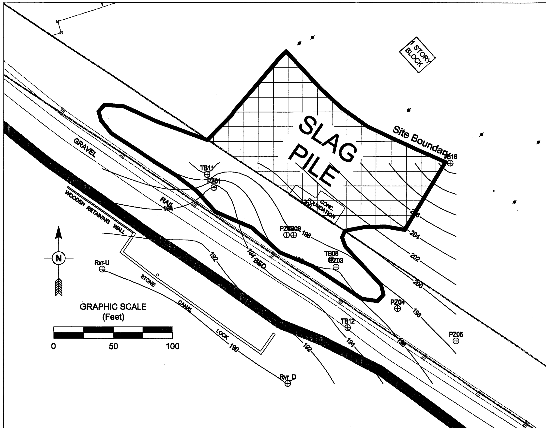
FIGURE 1-5 BEDROCK CONTOUR MAP
