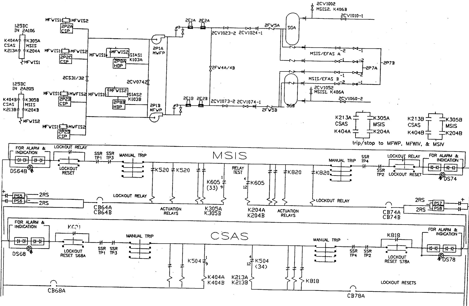
Sketch Two MSIS and CSAS Isolation of MFW and MS (contacts shown for power operation)
