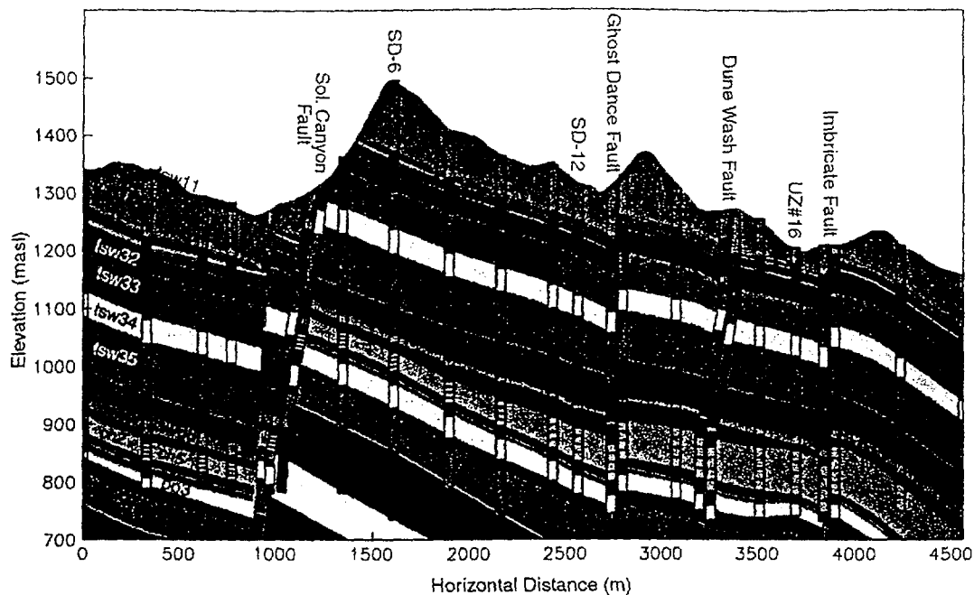
Figure VI-6. East-West Cross-Section Comparison along B-B'. GFM3.1 stratigraphy (DTN: MO9901MWDGFM31.000) overlain with FY99 UZ Model grid layering information (from DTN: LB990701233129.001).
