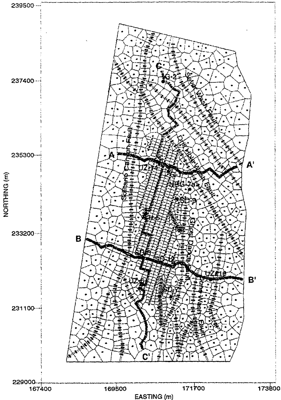
Figure VI-1. 2-D (Plan-View) Grid Design for FY99 UZ Model Flow-Field Calculations (from DTN: LB990701233129.001).
