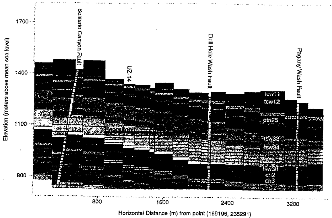
Figure VI-2. East-West Cross Section A-A' from the 3-D UZ Model Flow-Fields Grid (from DTN: LB990701233129.001).
