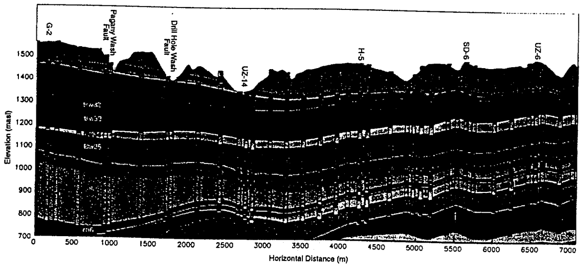
Figure V-8. North-South Cross-Section Comparison along C-C'. GFM3.1 stratigraphy (DTN: MO9901MWDGFM31.000) overlain with FY99 UZ Model calibration grid layering Information (from DTN: LB990501233129.004).
