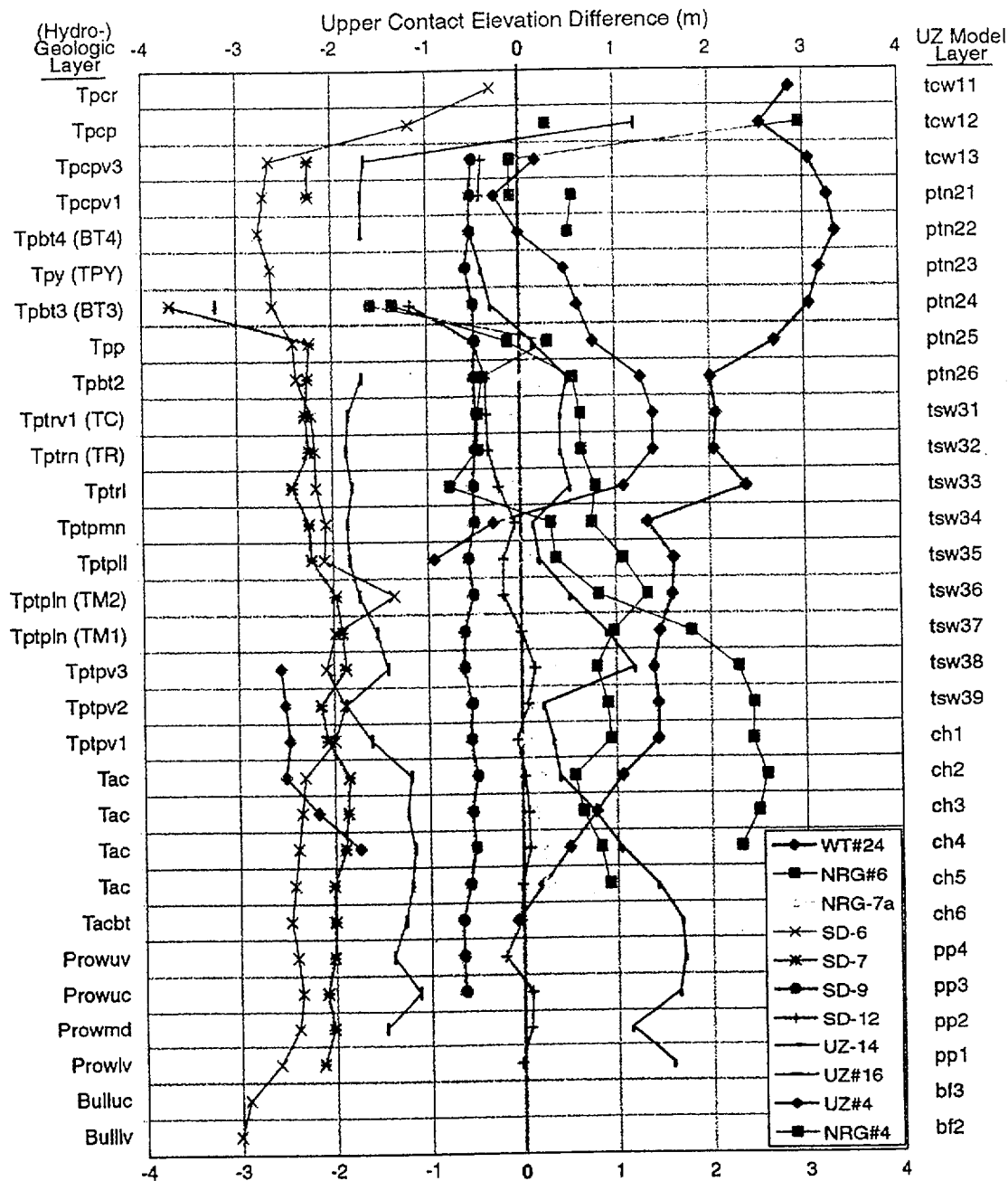
Figure VI-5. Upper Contact Elevation Differences: GFM3.1 "pix99el.dat" (DTN: MO9901MWDGFM31.000) Minus 3-D UZ Model (Flow-Fields) Grid (DTN: LB990701233129.001) at Selected Borehole Locations. [A negative value means the UZ Model layer contact elevation is higher than the stratigraphic pick.]
