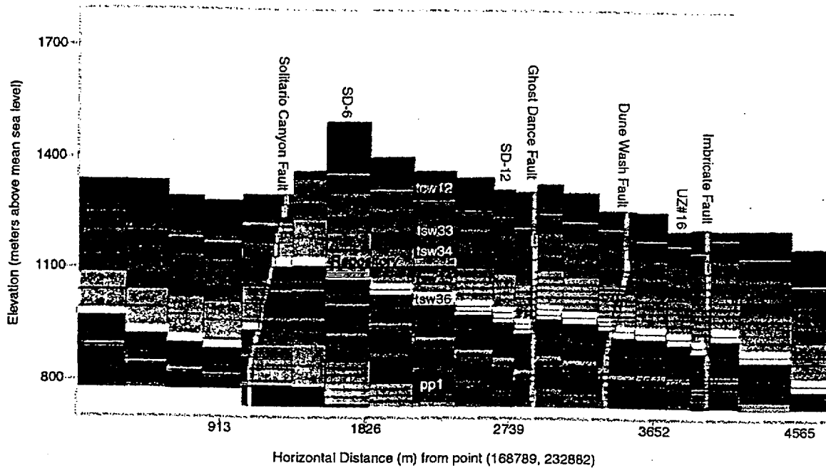
Figure VI-3. East-West Cross Section B-B' from the 3-D UZ Model Flow-Fields Grid (from DTN: LB990701233129.001).
