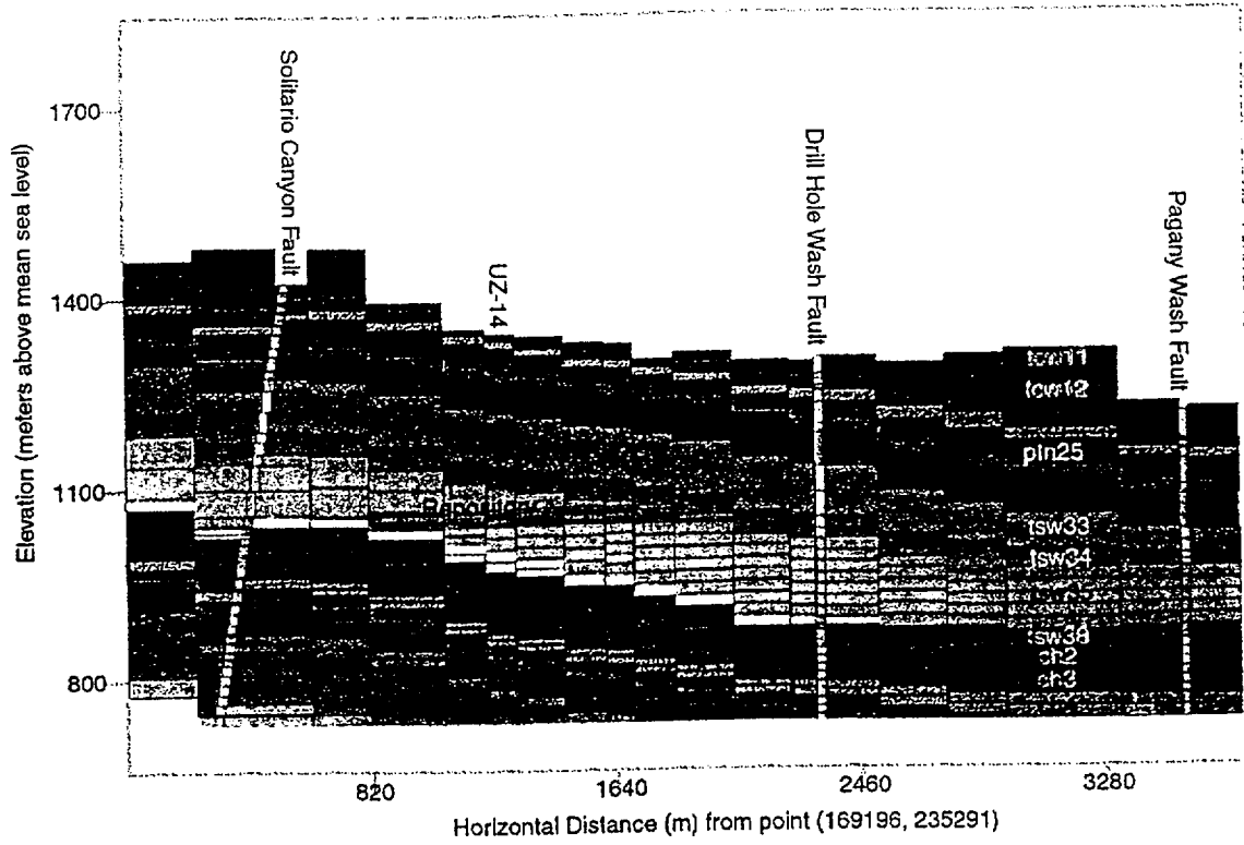
Figure V-2. East-West Cross Section A-A' from the 3-D UZ Model Calibration Grid (from DTN: LB990501233129.004).
