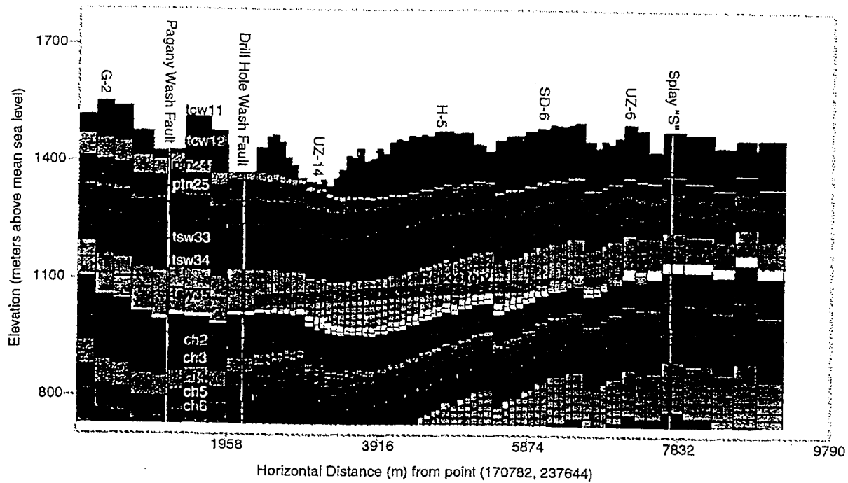
Figure VI-4. North-South Cross Section C-C' from the 3-D UZ Model Flow-Fields Grid (from DTN: LB990701233129.001).
