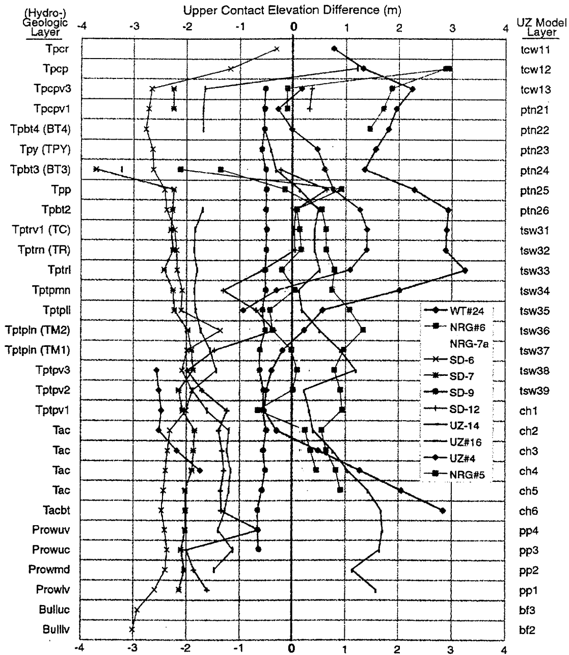
Figure V-5. Upper Contact Elevation Differences: GFM3.1 "pix99el.dat" (DTN: MO9901MWDGFM31.000) Minus 3-D UZ Model (Calibration) Grid (from DTN: LB990501233129.004) at Selected Borehole Locations. [A negative value means the UZ Model layer contact elevation is higher than the stratigraphic pick.]
