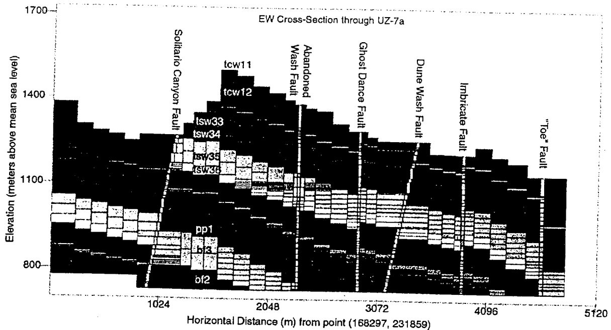
Figure IV-1. UZ-7a Cross-Sectional Grid (from DTN: LB990501233129.003).
