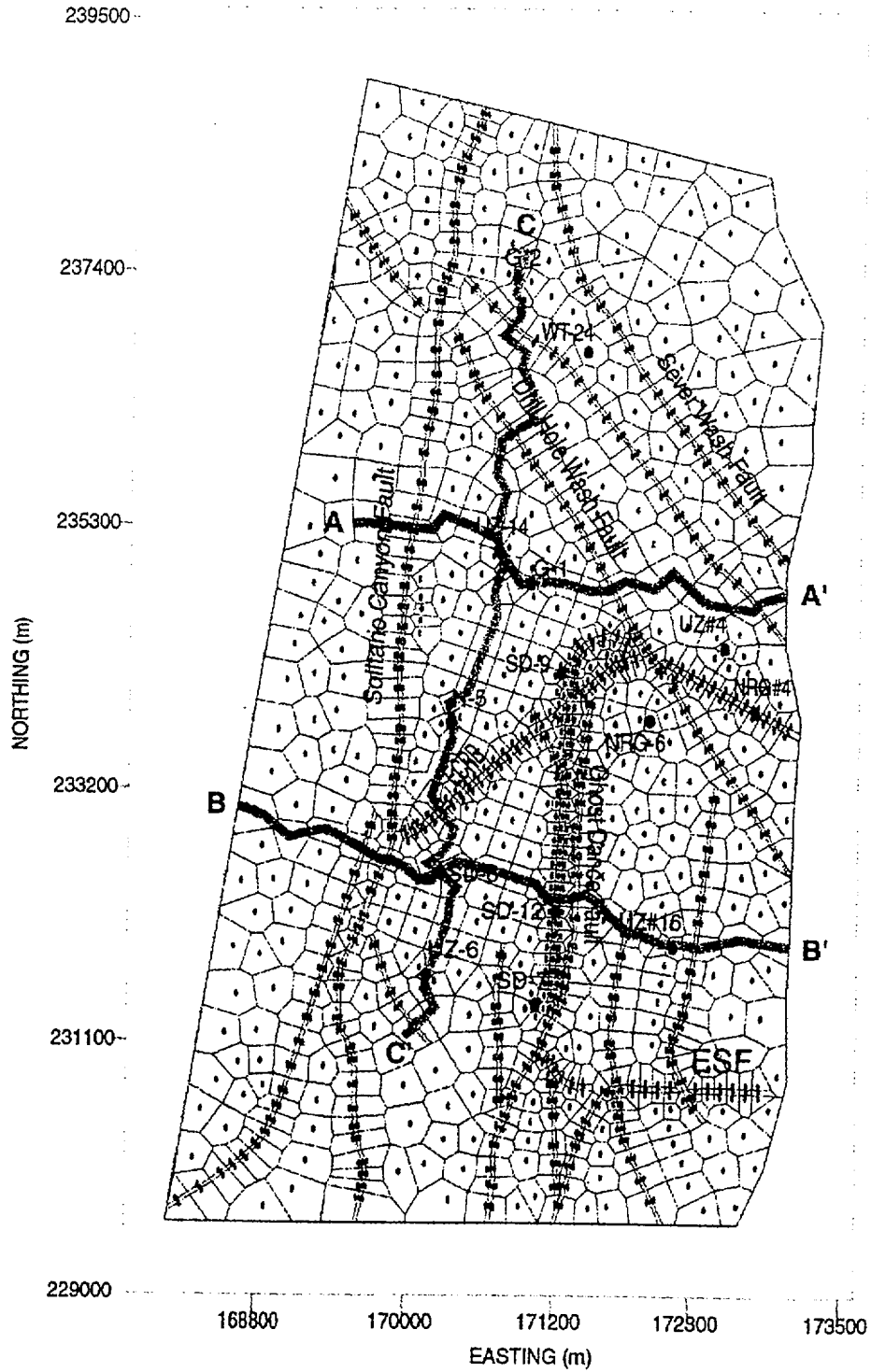
Figure V-1. 2-D (Plan-View) Grid Design for FY99 UZ Model Calibration (from DTN: LB990501233129.004).
