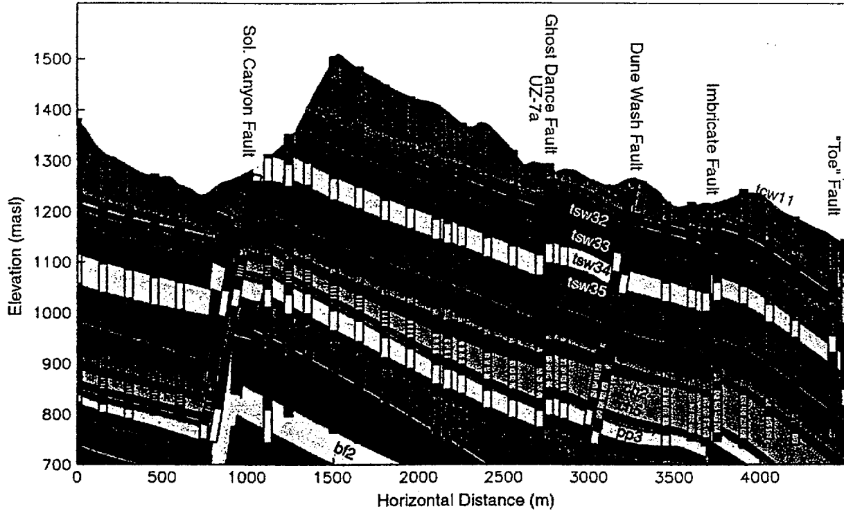
Figure IV-2. Comparison Between GFM3.1 (DTN: MO9901MWDGFM31.000) and Columns from the UZ-7a Cross-Sectional Grid (DTN: LB990501233129.003).
