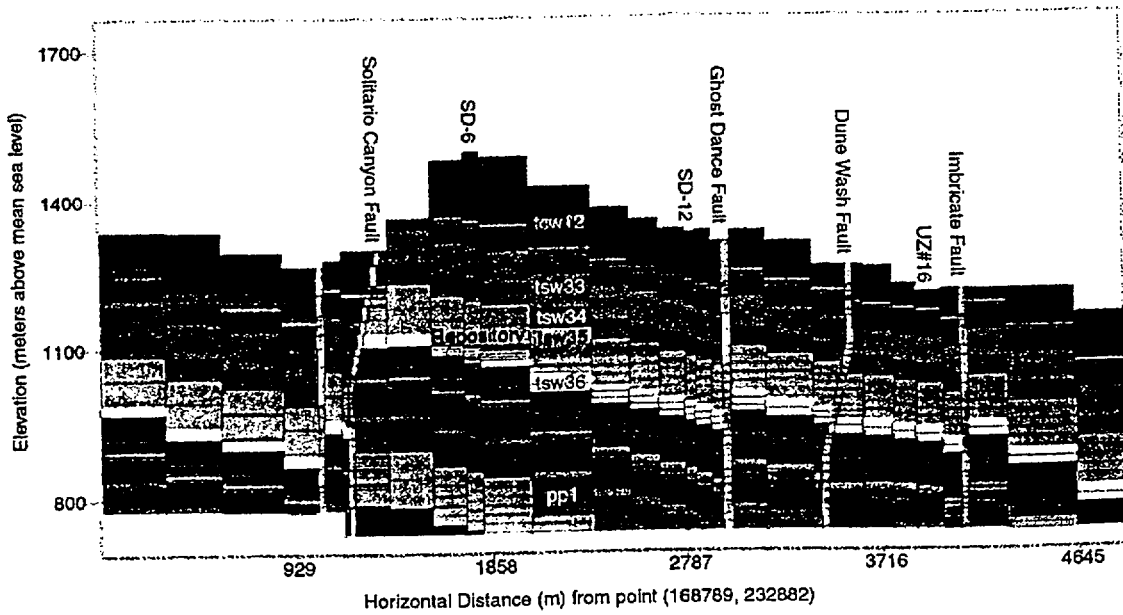
Figure V-3. East-West Cross Section B-B' from the 3-D UZ Model Calibration Grid (from DTN: LB990501233129.004).
