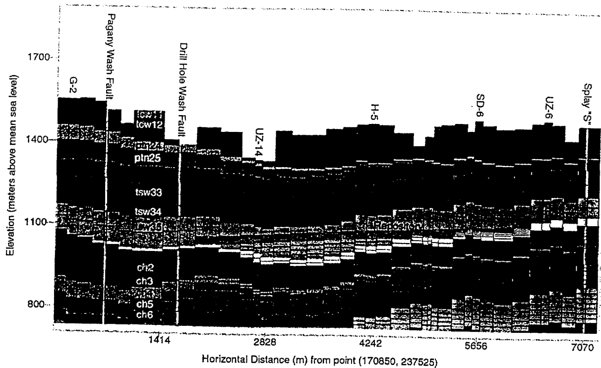
Figure V-4. North-South Cross Section C-C' from the 3-D UZ Model Calibration Grid (from DTN: LB990501233129.004).
