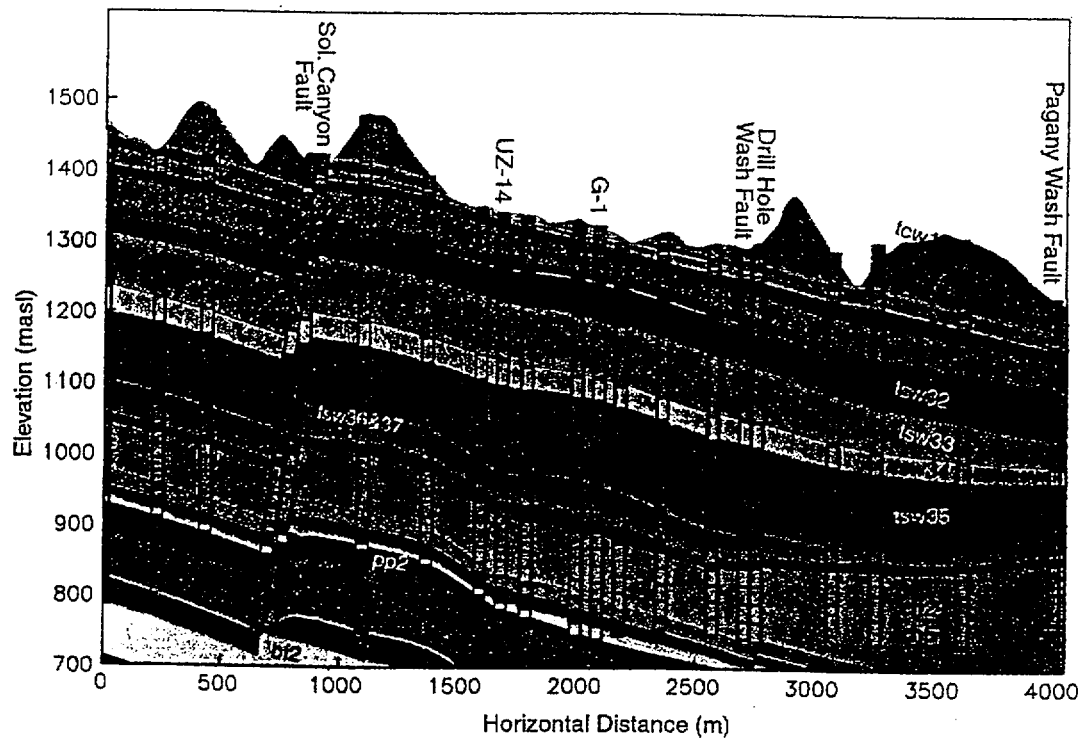
Figure V-6. East-West Cross-Section Comparison along A-A'. GFM3.1 stratigraphy (DTN: MO9901MWDGFM31.000) overlain with FY99 UZ Model calibration grid layering information (from DTN: LB990501233129.004).
