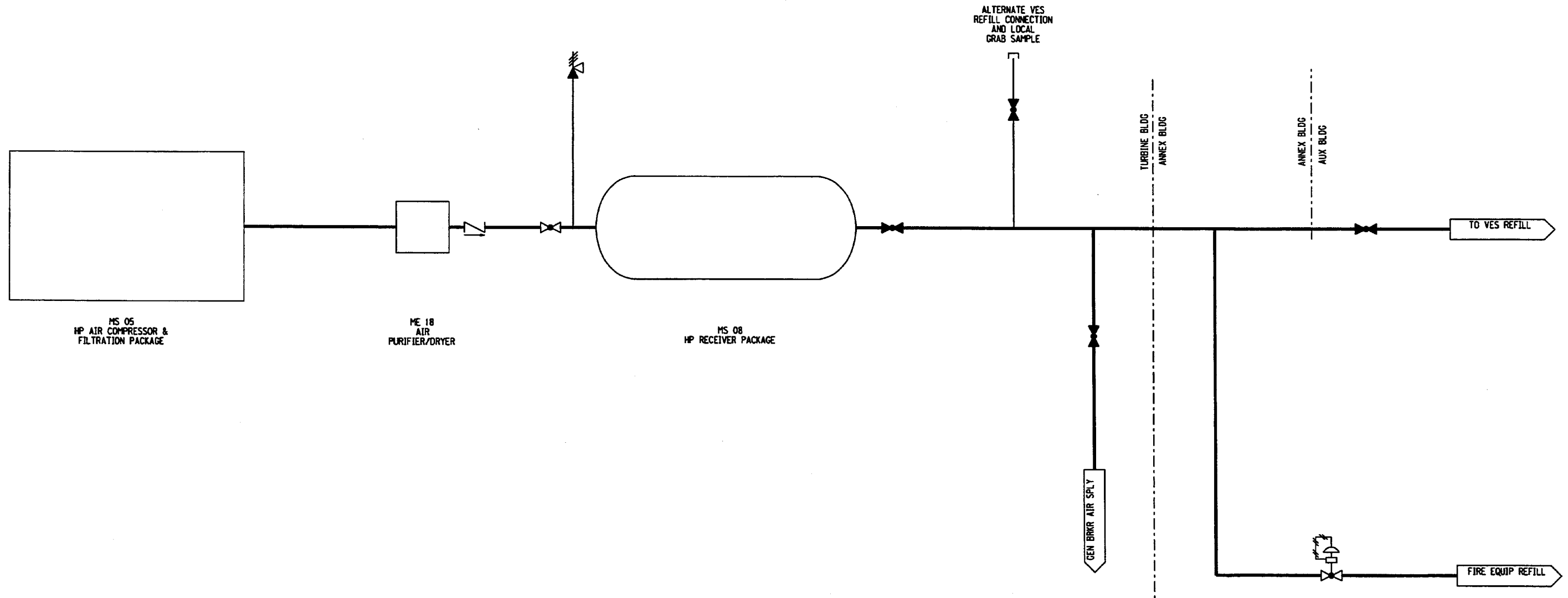
Figure 9.3.1-1 (Sheet 3 of 3)
