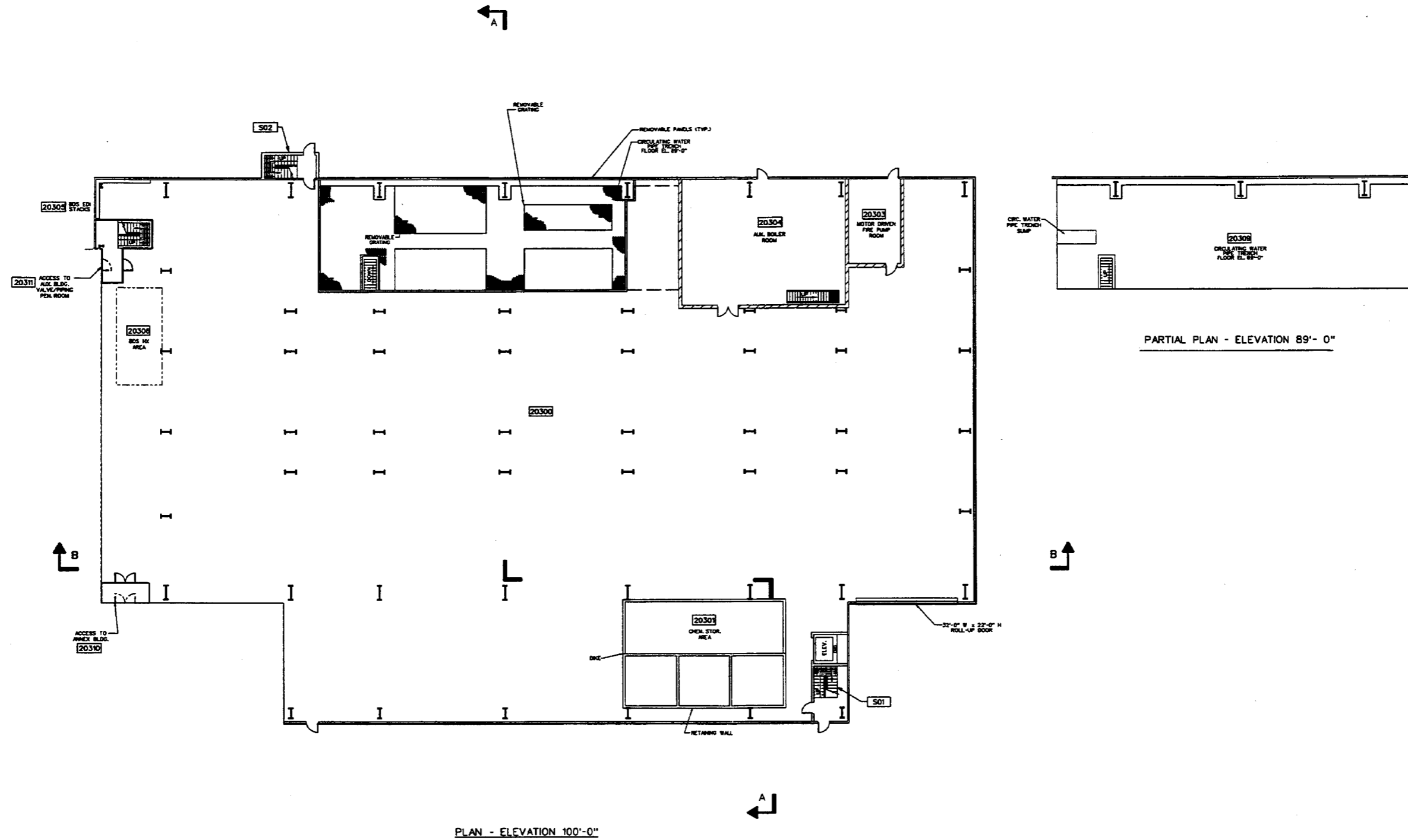
Turbine Building General Arrangement Plan at Elevation 89'-0" & 100'-0"
