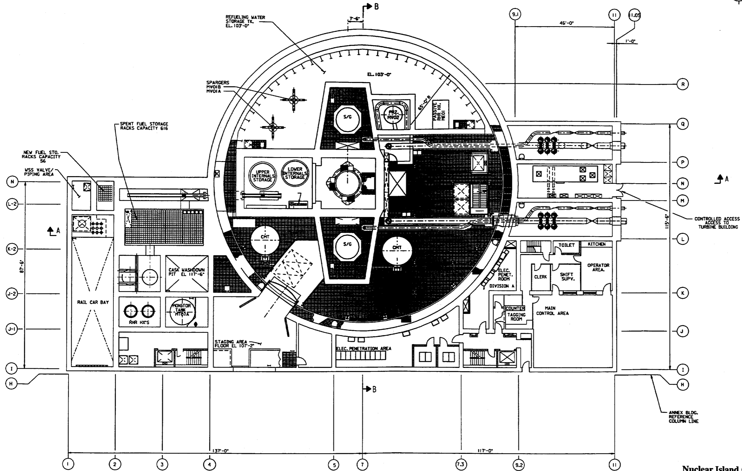
Nuclear Island General Arrangement Plan at Elevation 117'-6" with Equipment
