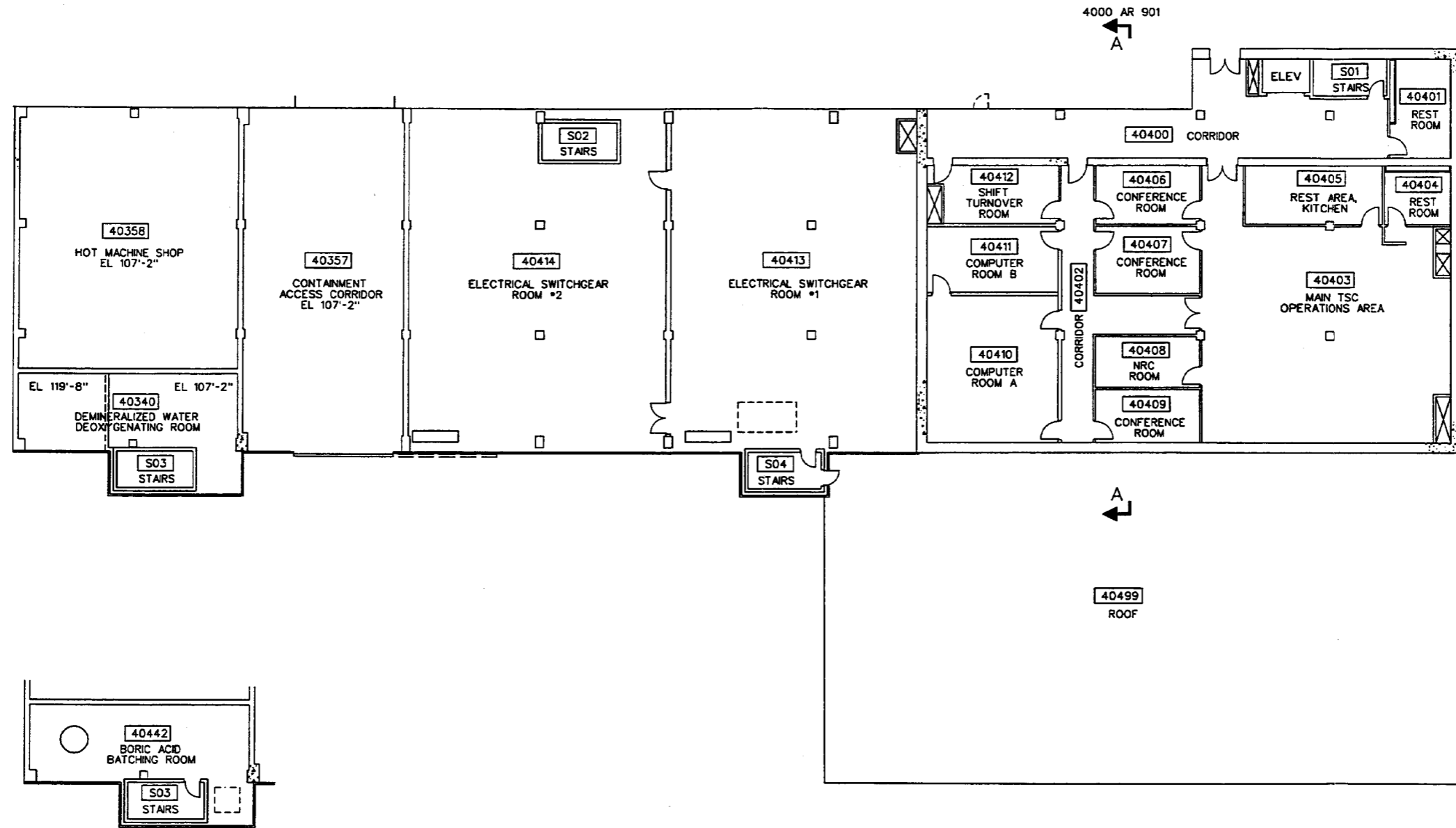
PART PLAN EL 126'-3"
