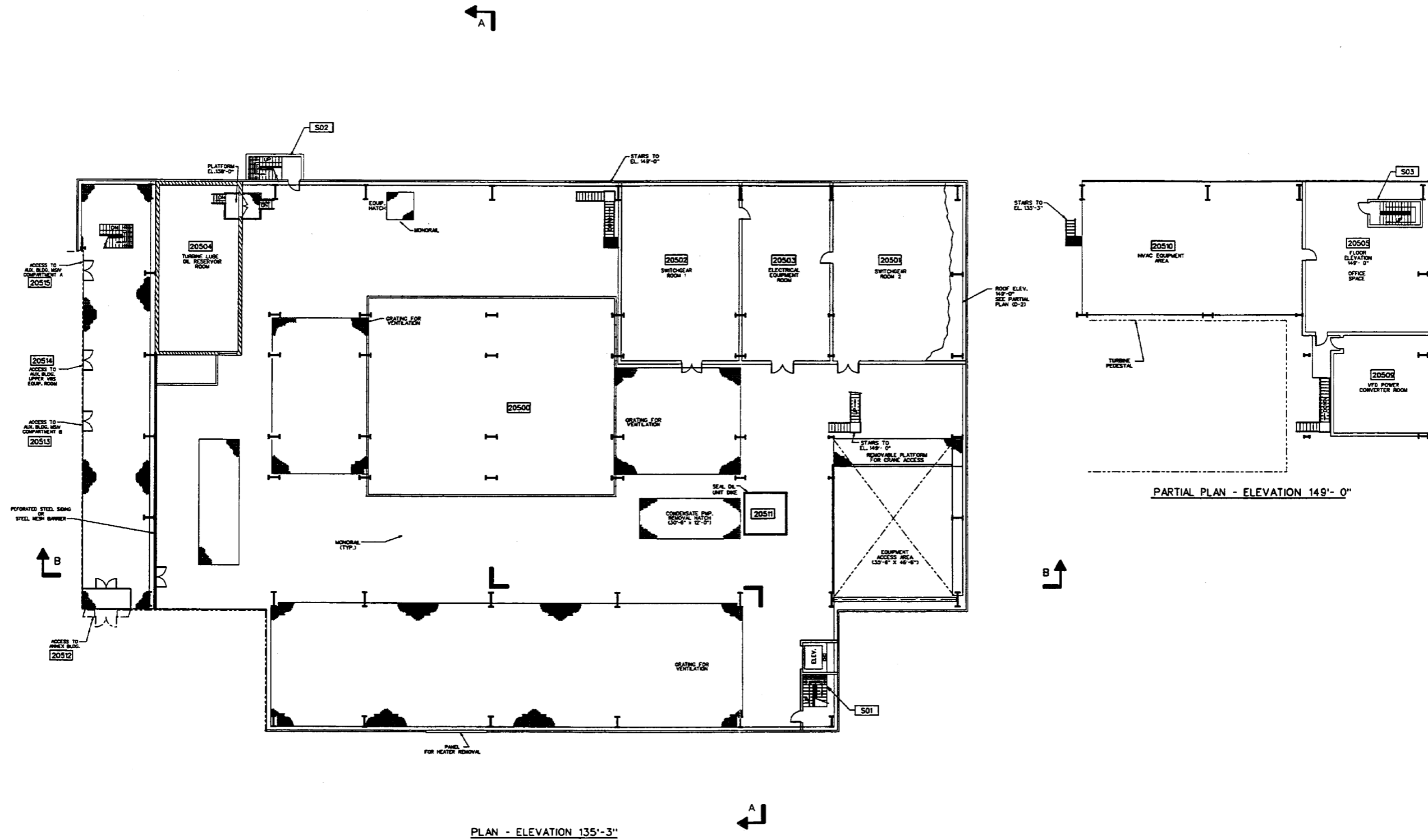
Turbine Building General Arrangement Plan at Elevation 135'-3"
