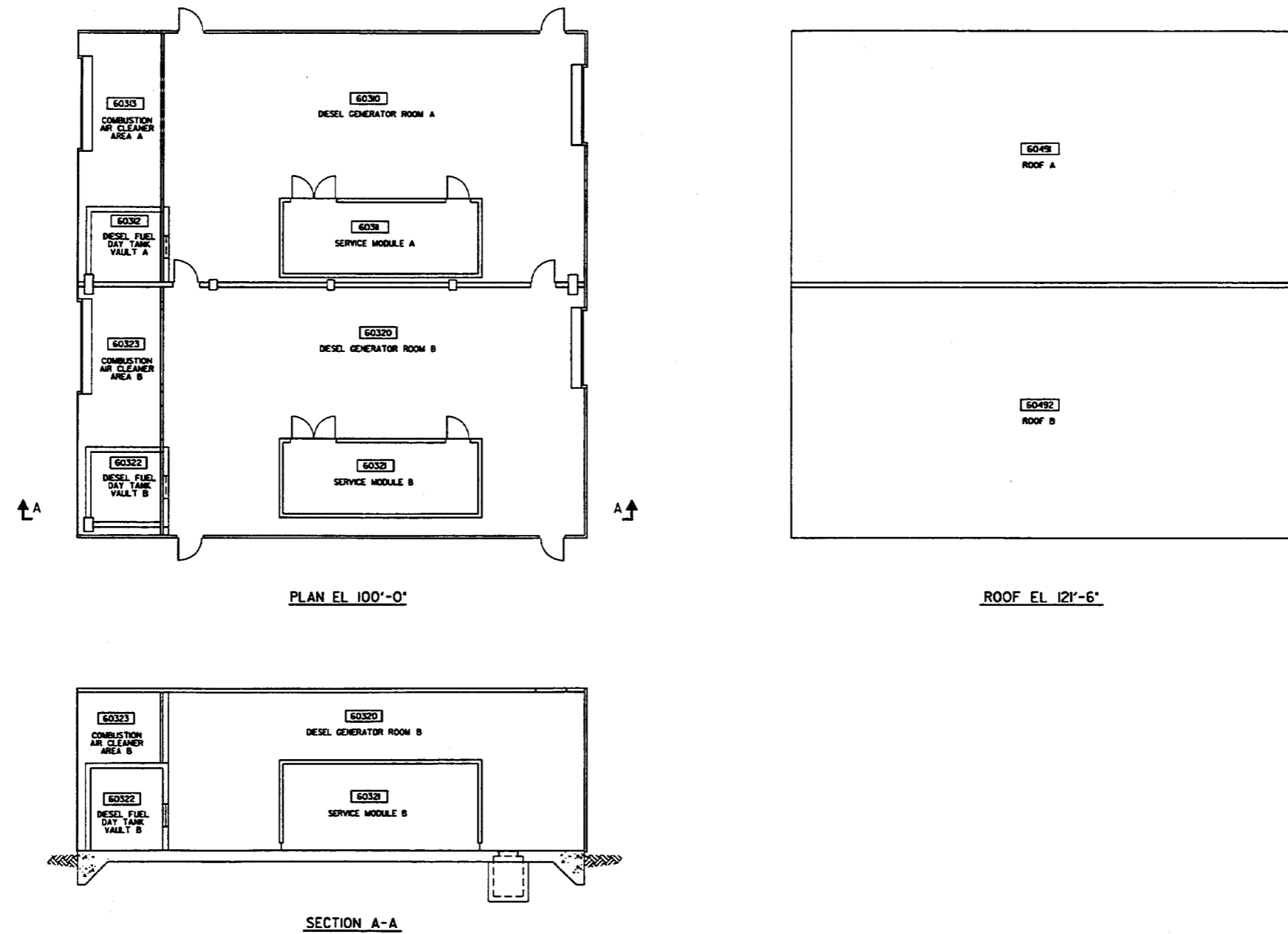
Diesel Generator Building General Arrangement Plan at Elevation 100'-0" & Section A-A
