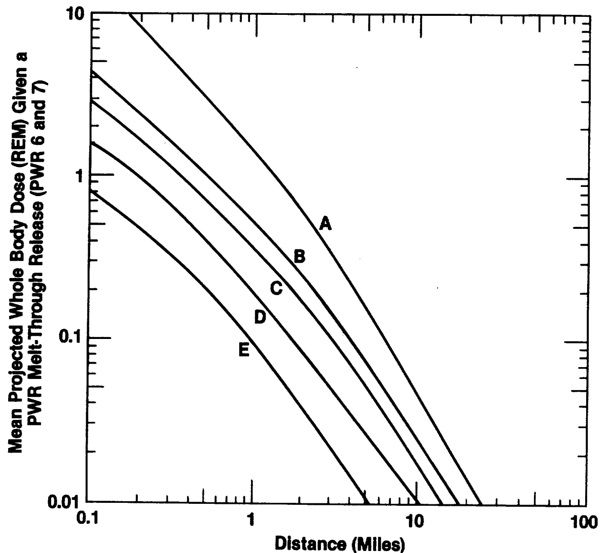
Figure 3.5-8 Conditional mean projected whole-body dose versus distance for sheltering and evacuation strategies. Projected doses are conditional on a PWR "melt-through" release (PWR 6 and 7) (from Reference 102).
