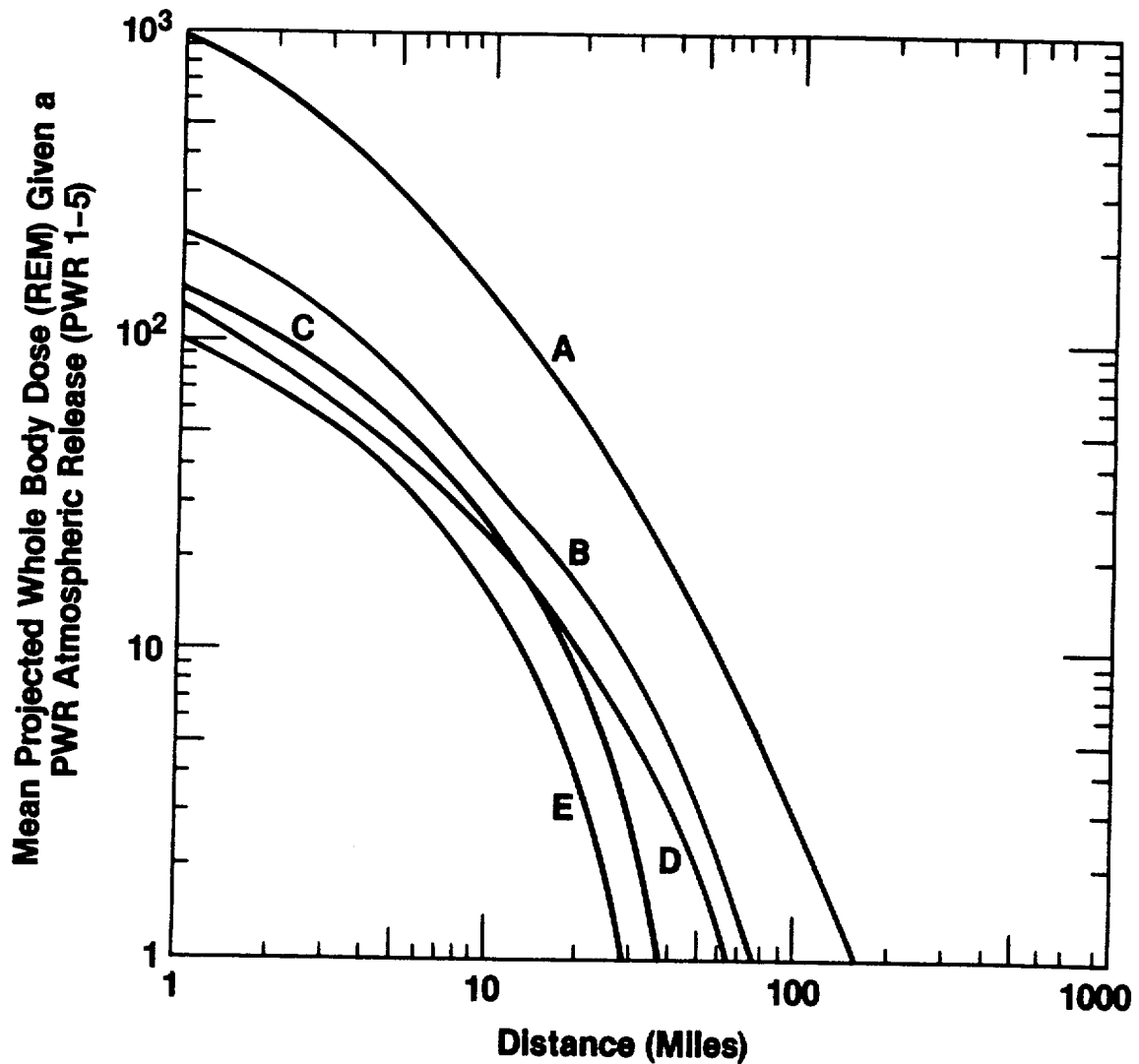
Figure 3.5-10 Conditional mean projected whole-body dose versus distance for sheltering and evacuation strategies. Projected doses are conditional on a PWR "atmospheric" release (PWR 1-5) (from Reference 102).
