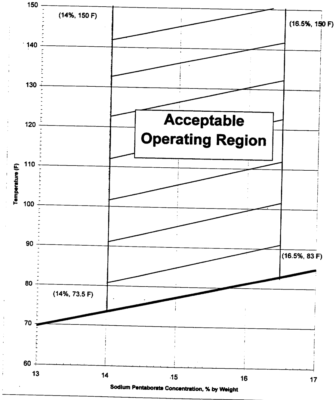
Figure 3.1.7-2 (page 1 of 1) Sodium Pentaborate Temperature Requirements
