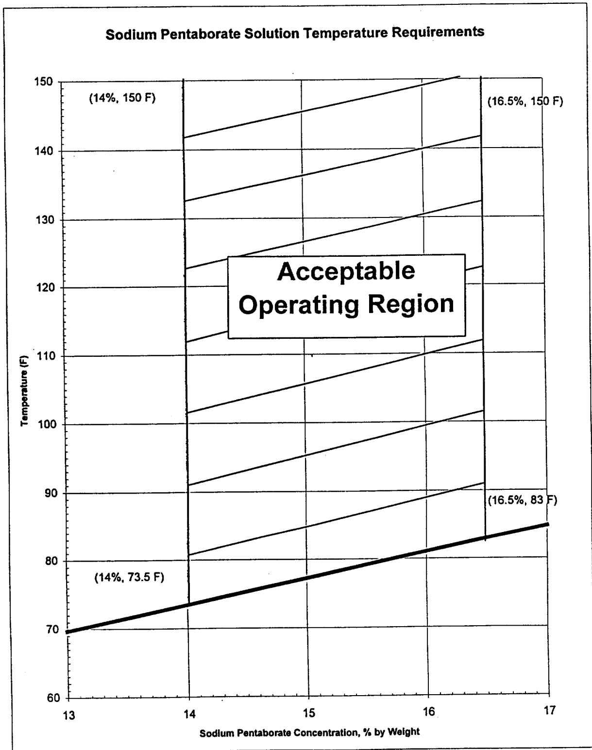
Figure 3.1.7-2 (page 1 of 1) Sodium Pentaborate Temperature Requirements
