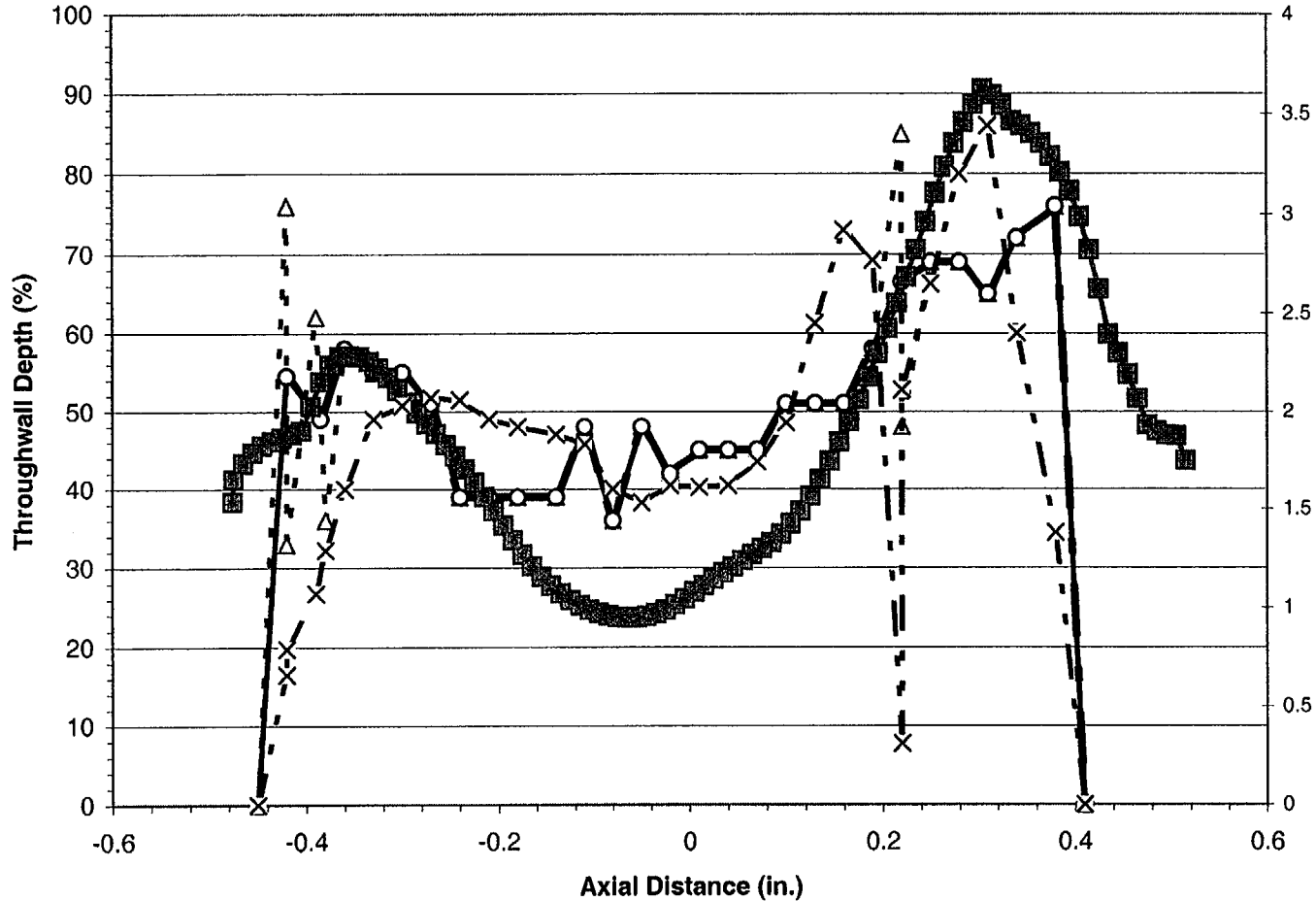
Figure D-44 Specimen R 29 - C 41 - 01H - Crack 1 - Year 1998 Comparison of Unadjusted, Adjusted, Burst and Voltage with Exam NDE Depth vs. Axial Length
