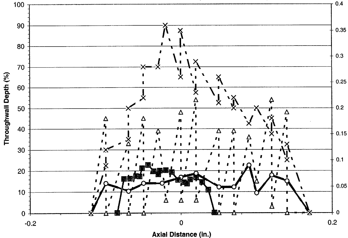
Figure D-42 Specimen R 29 - C 34 - 01H - Crack 1 - Year 1998 Comparison of Unadjusted, Adjusted, Burst and Voltage with Exam NDE Depth vs. Axial Length
