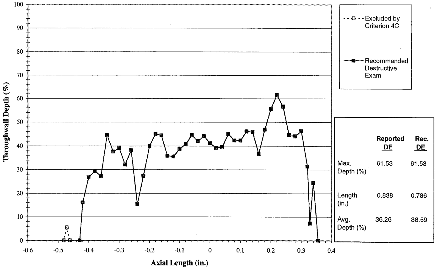
Figure C-10 Sample 9, TSP 2H - Crack 2 Depth vs. Axial Length
