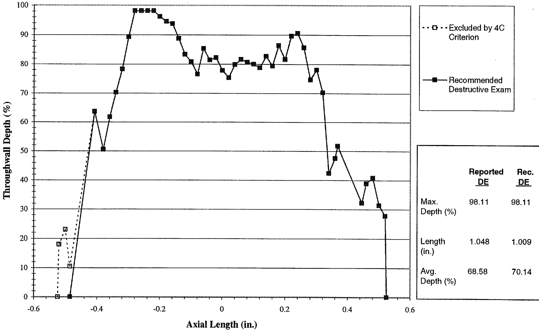
Figure C-16 Sample 11, TSP 4H - Crack 1 Depth vs. Axial Length
