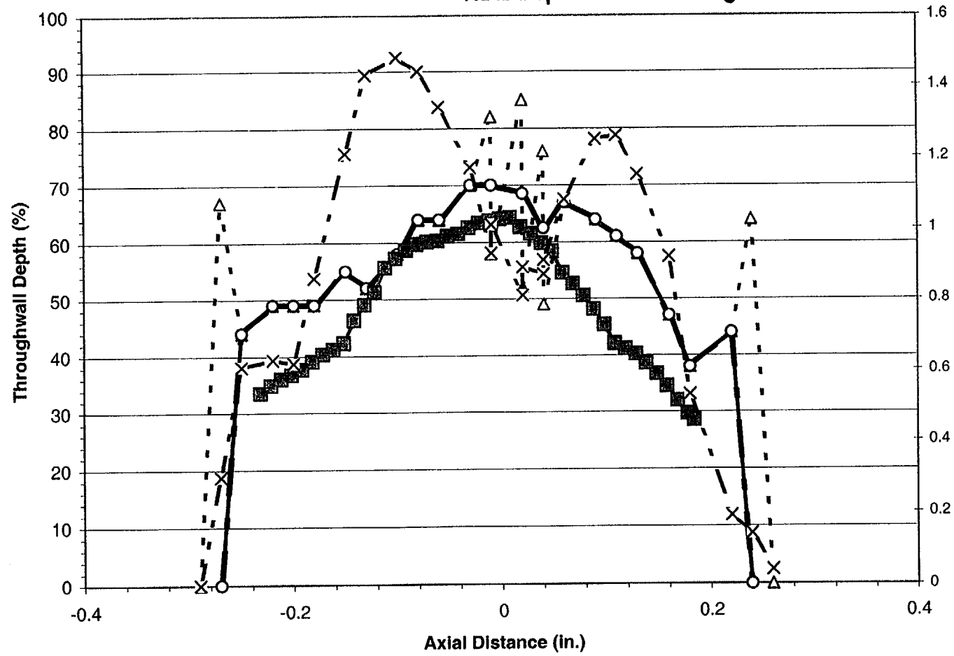
Figure D-35 Specimen R 21 - C 79 - 01H - Crack 1 - Year 1998 Comparison of Unadjusted, Adjusted, Burst and Voltage with Exam NDE Depth vs. Axial Length
