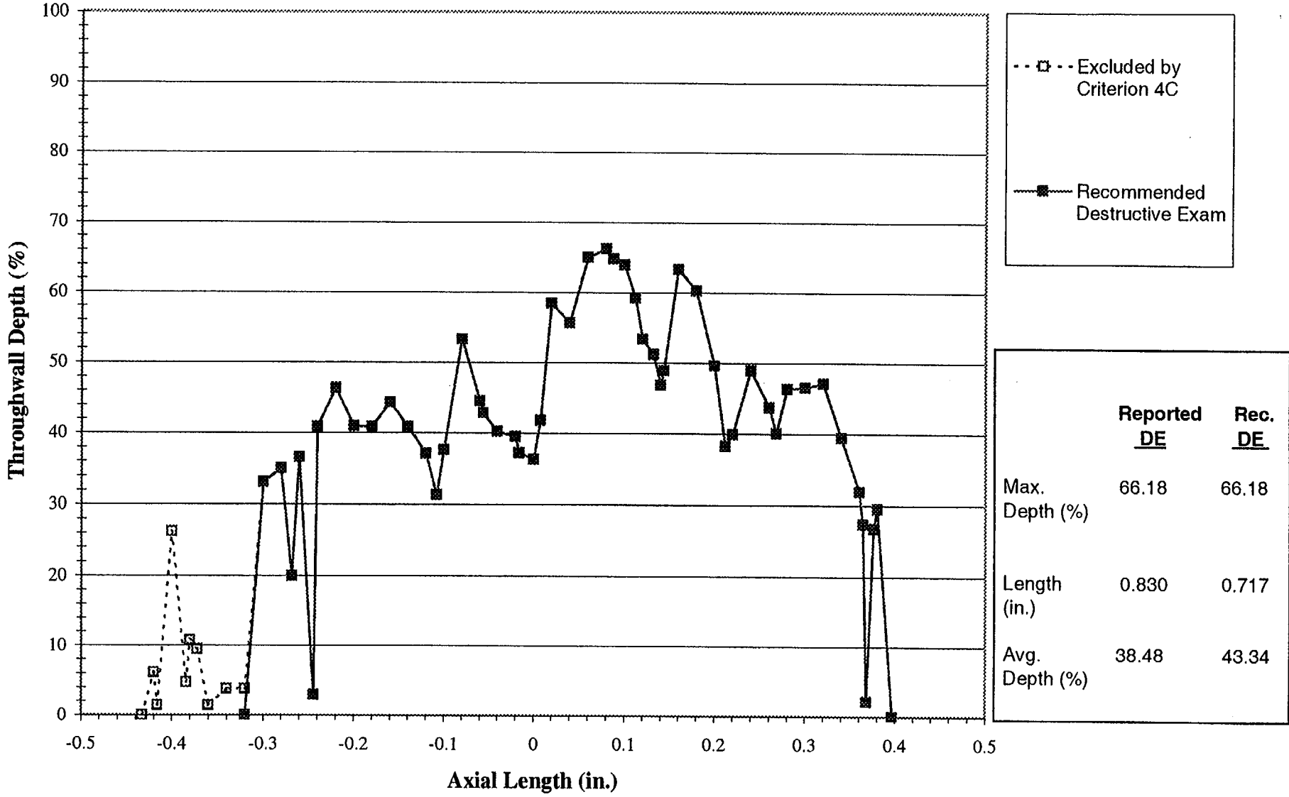
Figure C-12 Sample 9, TSP 3H - Crack 2 Depth vs. Axial Length
