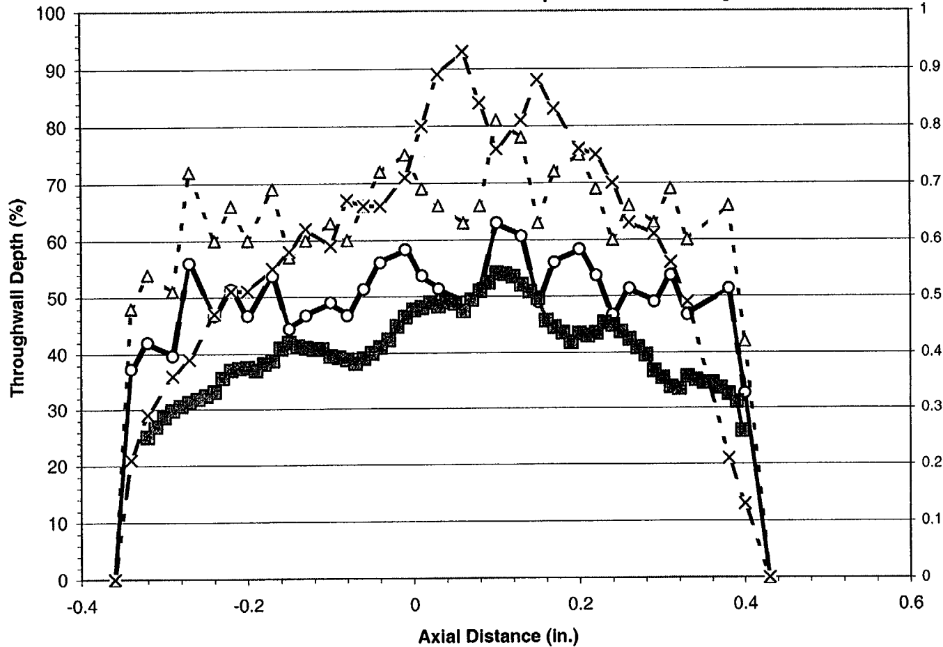
Figure D-33 Specimen R 21 - C 31 - 01H - Crack 2 - Year 1998 Comparison of Unadjusted, Adjusted, Burst and Voltage with Exam NDE Depth vs. Axial Length
