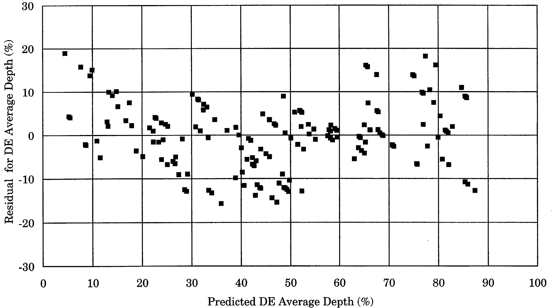
Figure 4-12 Dented TSP Axial PWSCC -- NDE Performance Test Scatter Plot Of Residuals - Adjusted NDE, Average Depth
