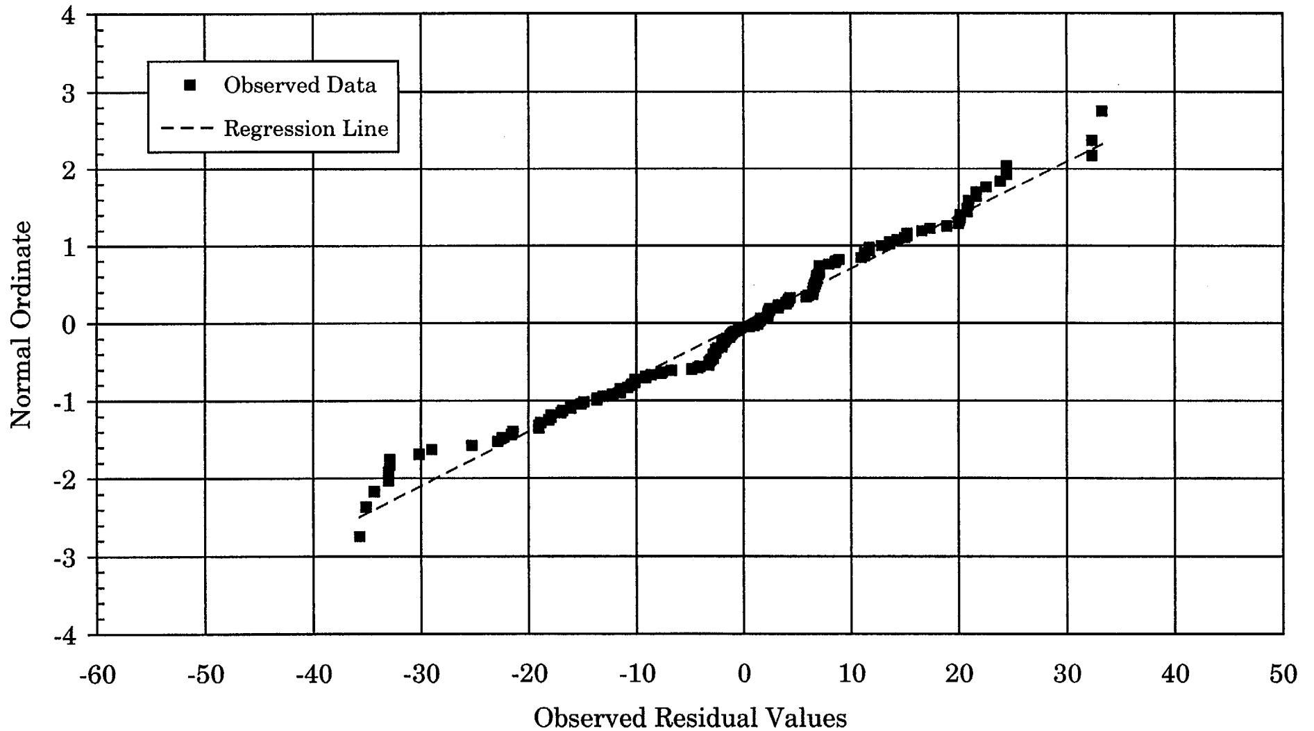
Figure 4-10 Dented TSP Axial PWSCC -- NDE Performance Test Normal Plot Of Residuals - Adjusted NDE, Maximum Depth
