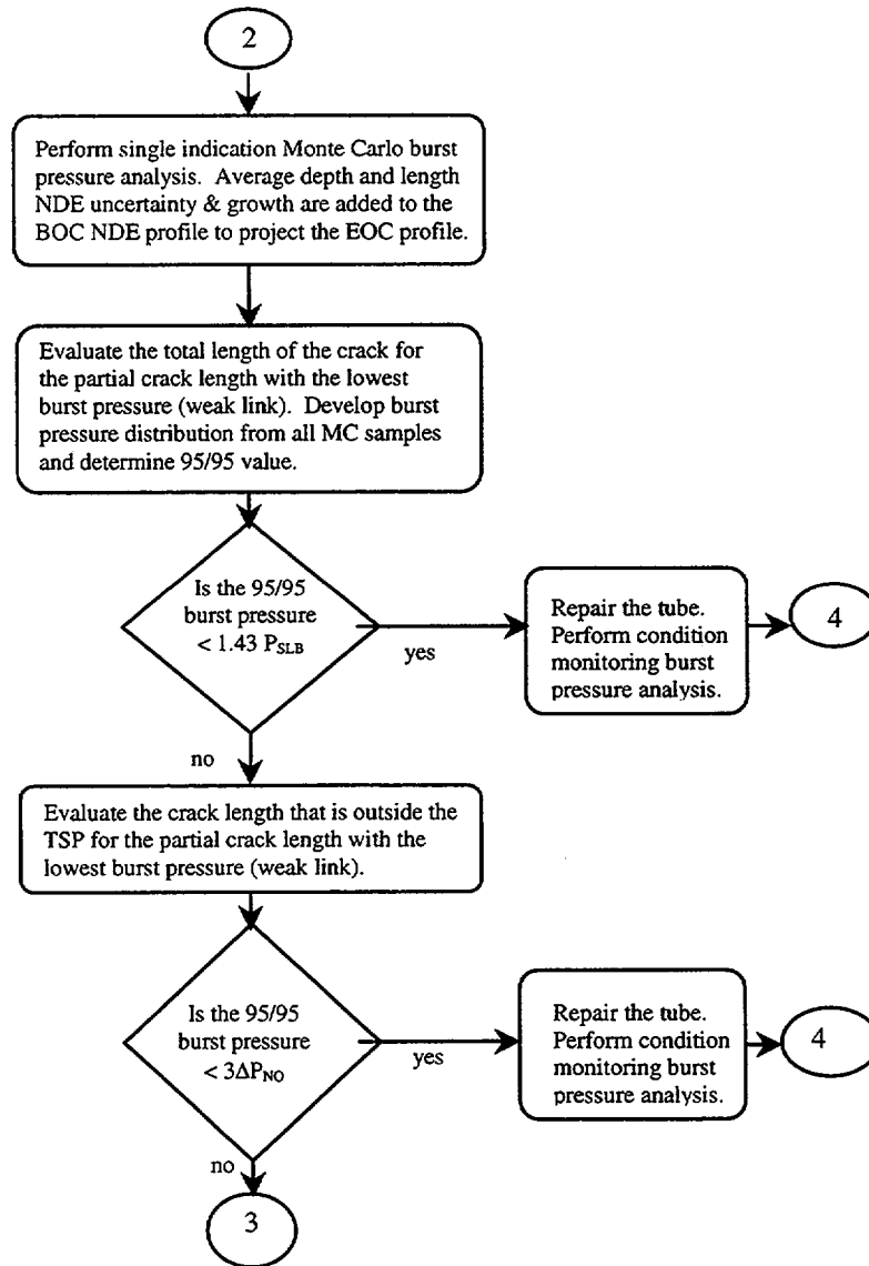
Figure 7-3. Burst Pressure Operational Assessment Repair Decision
