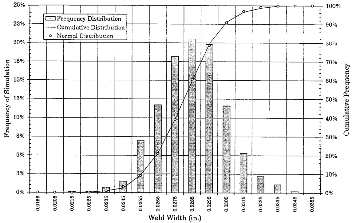
Figure 5: Results of the Monte Carlo Simulation
