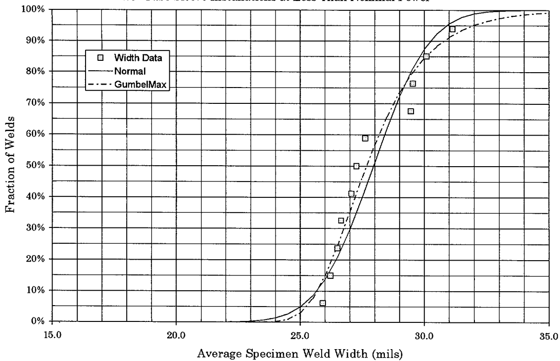
Figure 4: CDFs of Characterizing Distributions
