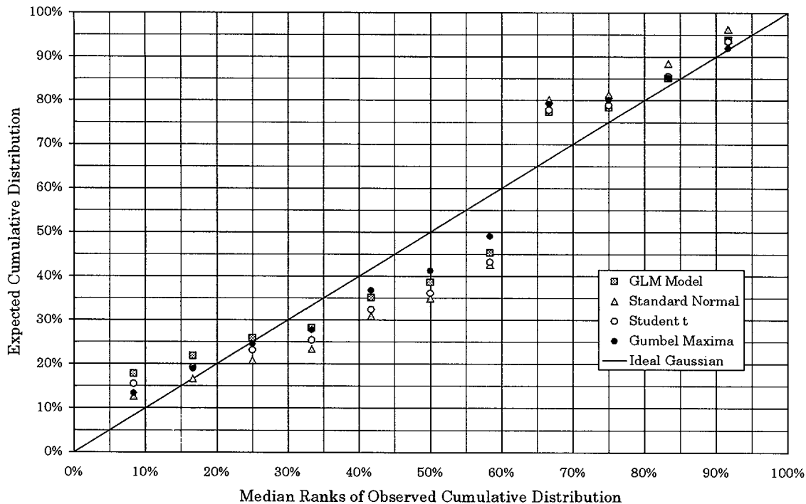
Figure 3: Correlation of Characterizing Distributions
