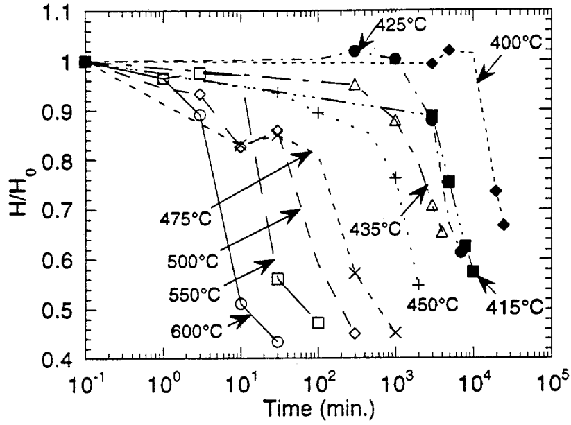
Fig. 5. Variations of normalized Vickers Hardness Number (VHN) of the Electroslieve material with time under isothermal aging at various temperatures.
