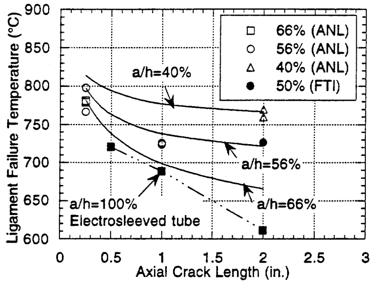
Fig. 22. Comparison of experimental ligament failure temperatures (from NUREG/CR-6575) with predicted values (using flow stress model) for unsleeved Alloy 600 tube with part-throughwall axial cracks under EPRI ramp. Also shown are FTI data for an unsleeved tube with a 2 in./50%TW crack (filled circle) and Electrosleeved tubes (filled squares) with throughwall cracks in the parent tubes.
