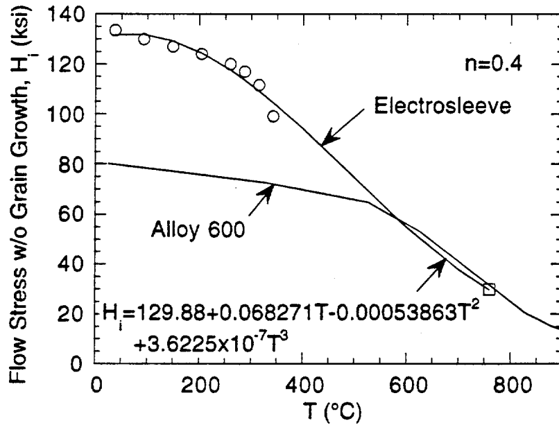
Fig. 10. Flow stress ("unaged") vs. temperature plot for electrosleeve material and Alloy 600. The Electrosleeve data (square symbol) at 760°C was estimated from tensile data on a single specimen pre-aged and tested at 760°C, using n=0.4 .
