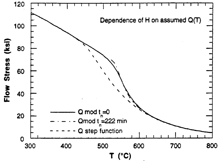
Fig. 30. Effect of the shape of the variation of activation energy with temperature on the calculated loss of flow stress for a 1°C min ramp. Note also that the nucleation time has little effect on the flow stress at the temperatures of interest.
