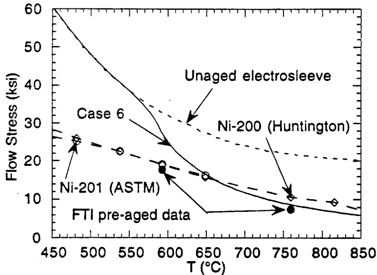
Fig. 33. Comparison of calculated flow stresses (including aging) of Electro sleeve (solid line) with flow stress data (open symbols) of Ni 200 (Huntington) and Ni-201 (ASTM). Also shown are the flow stress of the unaged electro sleeve (short dashed line) and two FTI flow stress data (filled circle) on 30-min aged specimens.
