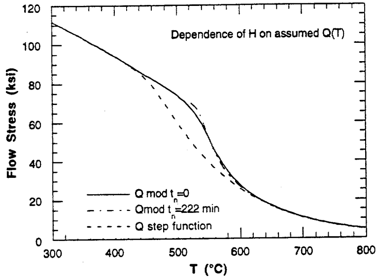
Fig. 30. Effect of the shape of the variation of activation energy with temperature on the calculated loss of flow stress for a 1^\circ\text{C}/\text{min} ramp. Note also that the nucleation time has little effect on the flow stress at the temperatures of interest.
