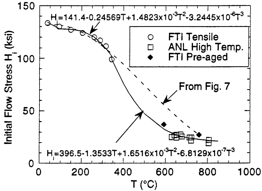
Fig. 18. Original unaged flow stress curve (dashed line) of the Electro sleeve estimated from FTI tensile data before the ANL tests were conducted and revised unaged flow stress curve (solid line) of the Electro sleeve calculated using the ANL tests.
