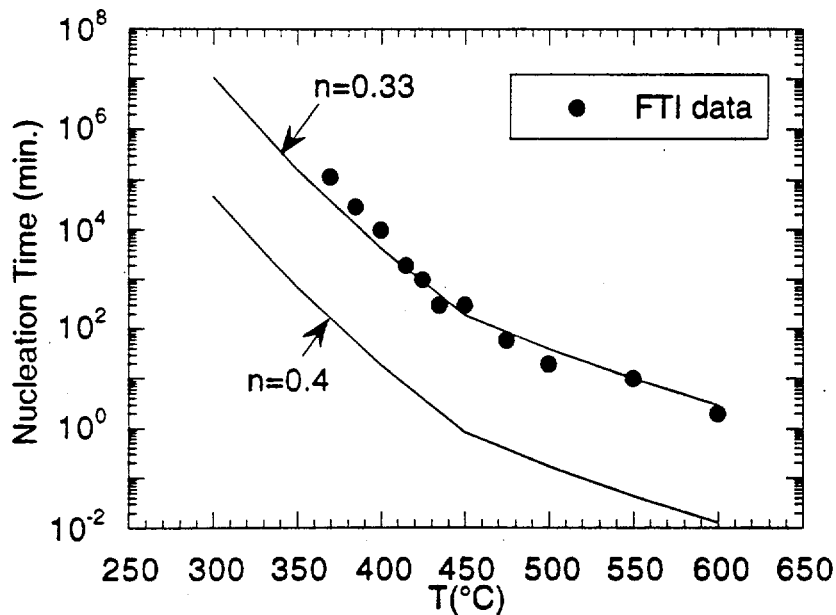
Fig. 11. Variation of calculated "nucleation" times to onset of rapid loss of flow stress (or grain growth) under isothermal aging with aging temperature for Hall-Petch exponents of n = 0.33 and n = 0.40 , using a temperature-dependent activation energy given by the step function in Fig. 6. Also shown are nucleation times for rapid loss of flow stress derived from the FTI data shown in Fig. 5.
