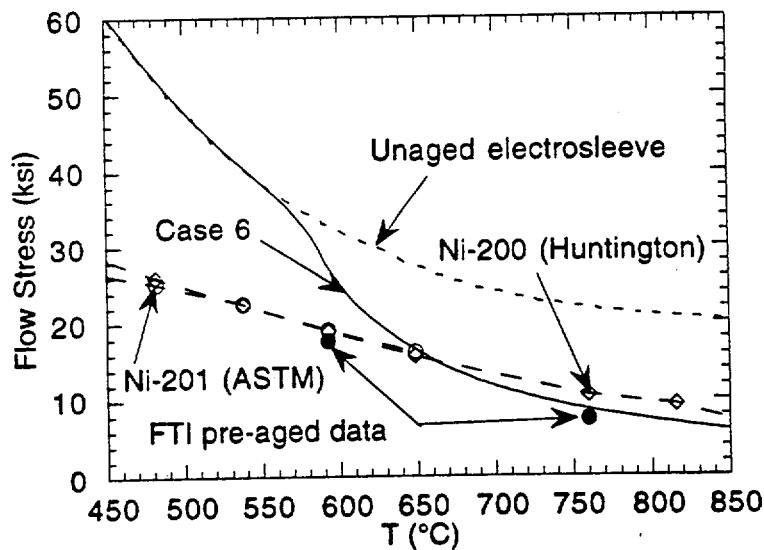
Fig. 33. Comparison of calculated flow stresses (including aging) of Electro sleeve (solid line) with flow stress data (open symbols) of Ni 200 (Huntington) and Ni-201 (ASTM). Also shown are the flow stress of the unaged electro sleeve (short dashed line) and two FTI flow stress data (filled circle) on 30-min aged specimens.
