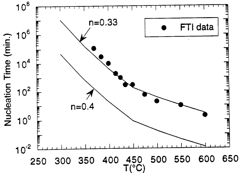
Fig. 11. Variation of calculated "nucleation" times to onset of rapid loss of flow stress (or grain growth) under isothermal aging with aging temperature for Hall-Petch exponents of n=0.33 and n=0.40 , using a temperature-dependent activation energy given by the step function in Fig. 6. Also shown are nucleation times for rapid loss of flow stress derived from the FTI data shown in Fig. 5.
