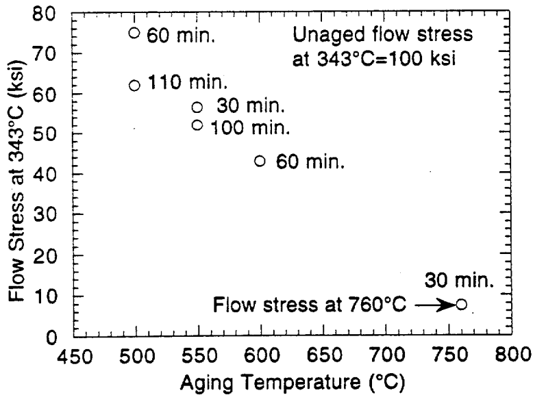
Fig. 8. Flow stress data on the Electro sleeve material pre-aged for various times at high temperatures. All the tensile tests were conducted at 343°C, except for the test on the specimen pre-aged at 760°C, which was conducted at 760°C.
