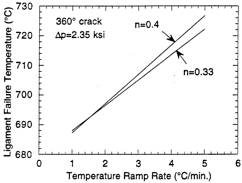
Fig. 16. Predicted ligament failure temperatures by the Hall-Petch model for Electrosleeved tubes with a throughwall 360^\circ circumferential crack under various temperature ramps.
