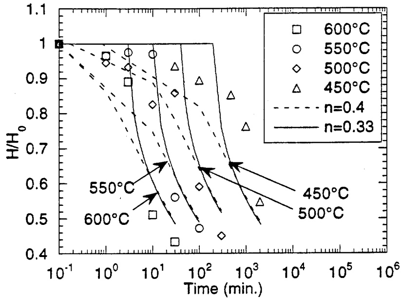
Fig. 12. Comparison of the calculated variations of normalized Vickers Hardness Number (VHN) of the Electro sleeve, using the Hall-Petch model with n=0.33 and n=0.4 , with the experimentally measured variations under isothermal aging at various temperatures.
