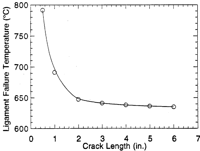
Fig. 29. Effect of crack length on the predicted ligament failure temperature of the reference Electrosleeved tube with throughwall axial cracks in the parent tube during the Case 6 SBO severe accident ramp.
