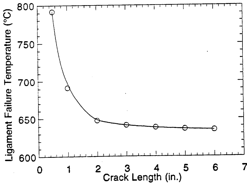
Fig. 29. Effect of crack length on the predicted ligament failure temperature of the reference Electroslieved tube with throughwall axial cracks in the parent tube during the Case 6 SBO severe accident ramp.
