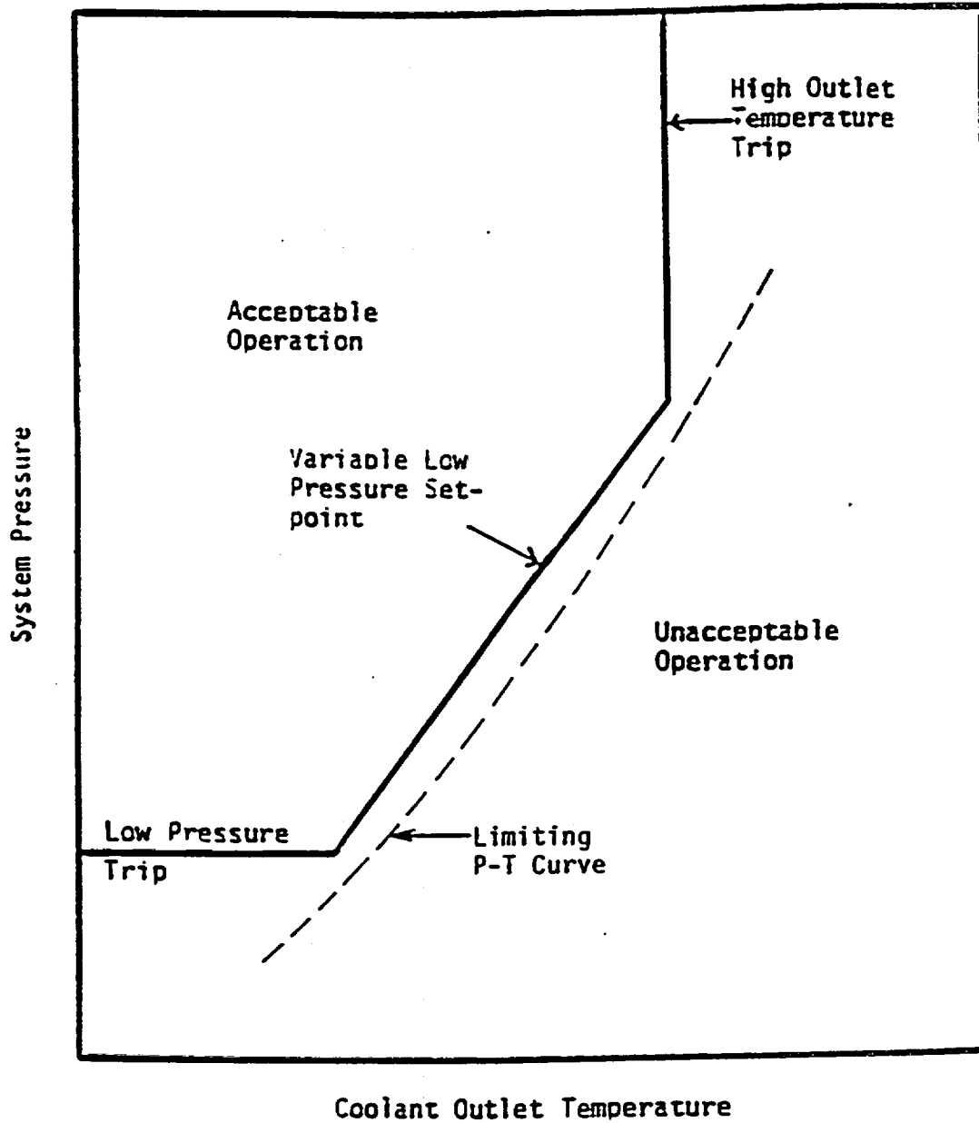
FIGURE 6-2. RPS P-T CORE PROTECTION ENVELOPE
