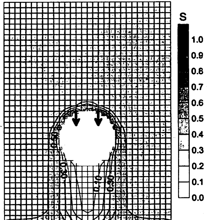
Figure 2. Rectangular element grid 2. Saturation is contoured and arrows denote locations of the first drips.
