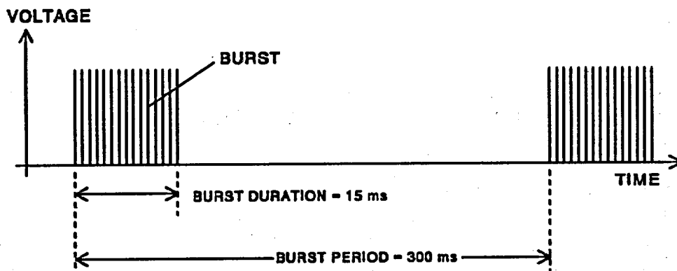
Figure 6.5 Pattern of EFT Bursts
