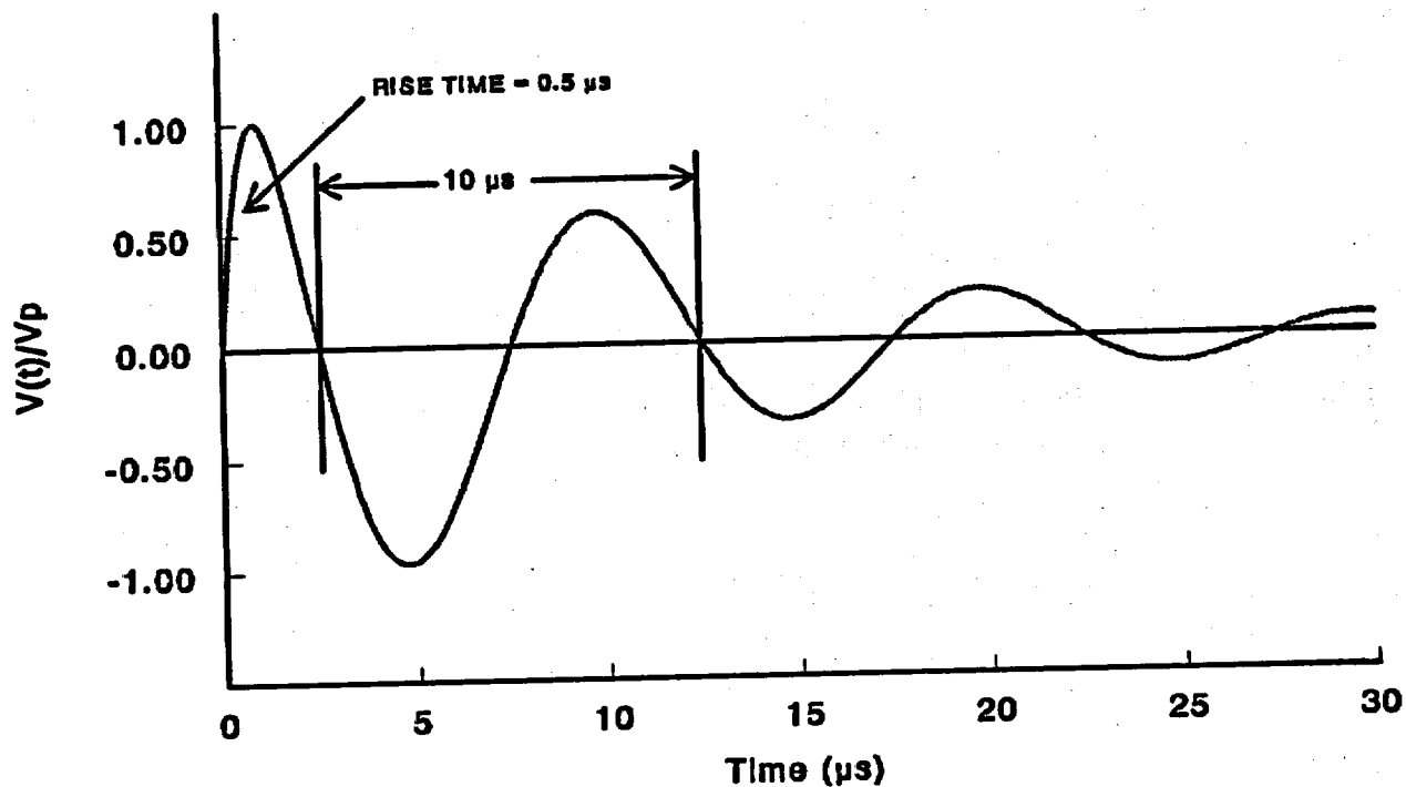
Figure 6.1 100-kHz Ring Wave
