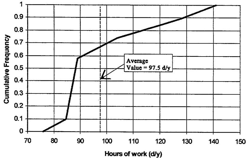
Figure 5.2 Cumulative Distribution Function for t .
