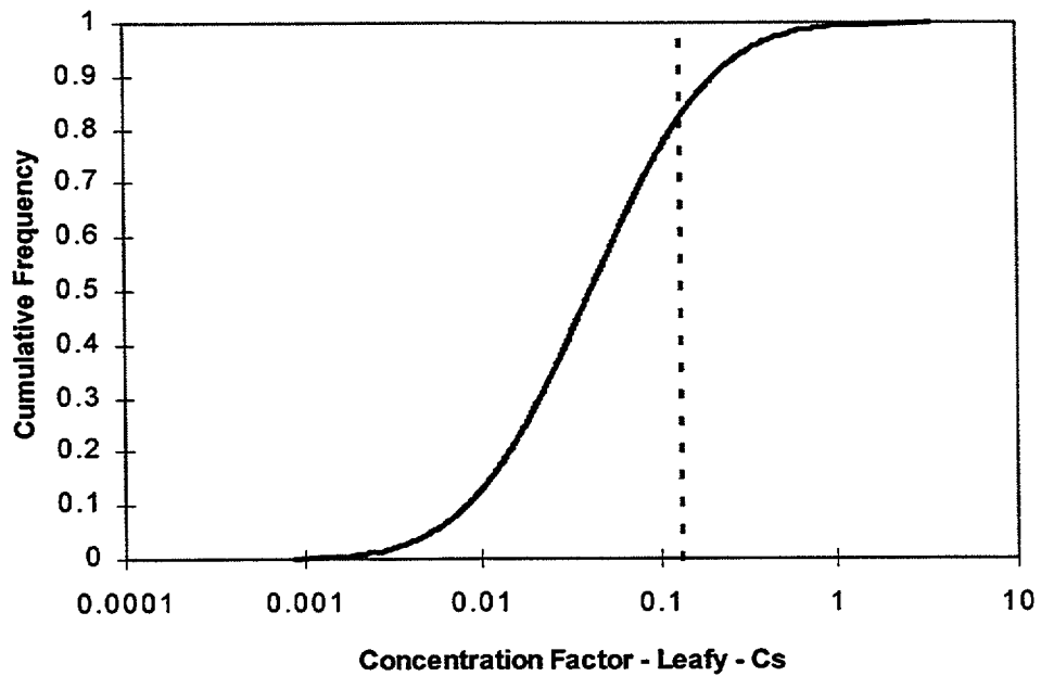
Figure 6.87 Cumulative frequency of sampled B_{jv} for Cs in leafy vegetables (dashed vertical line = NUREG/CR-5512, Vol. 1, default)
