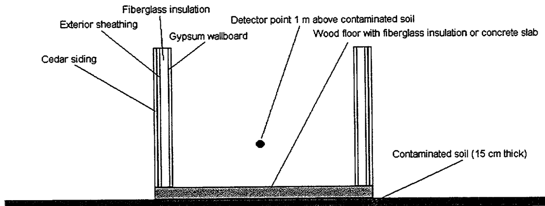
Figure 6.8 Cross section of building for calculating gamma activity from contaminants in soil
