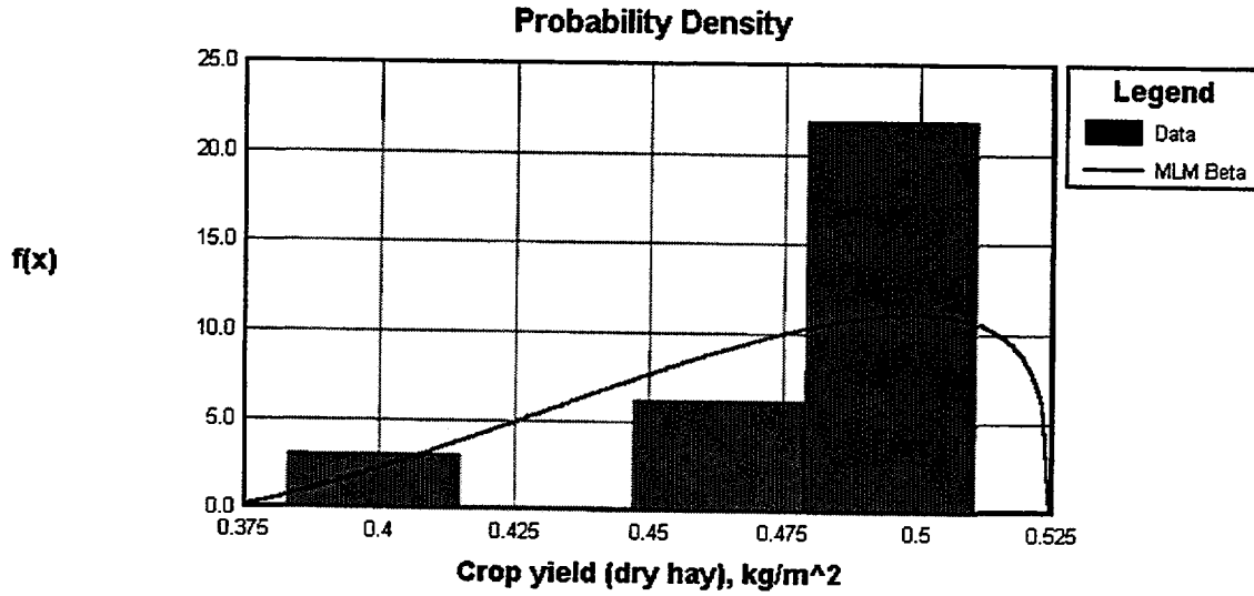
Figure 6.38 Frequency distribution and proposed PDF for Y_h
