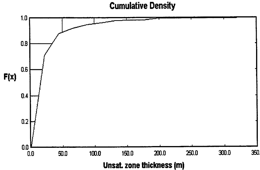
Figure 6.22 Empirical cumulative distribution function for H 2
