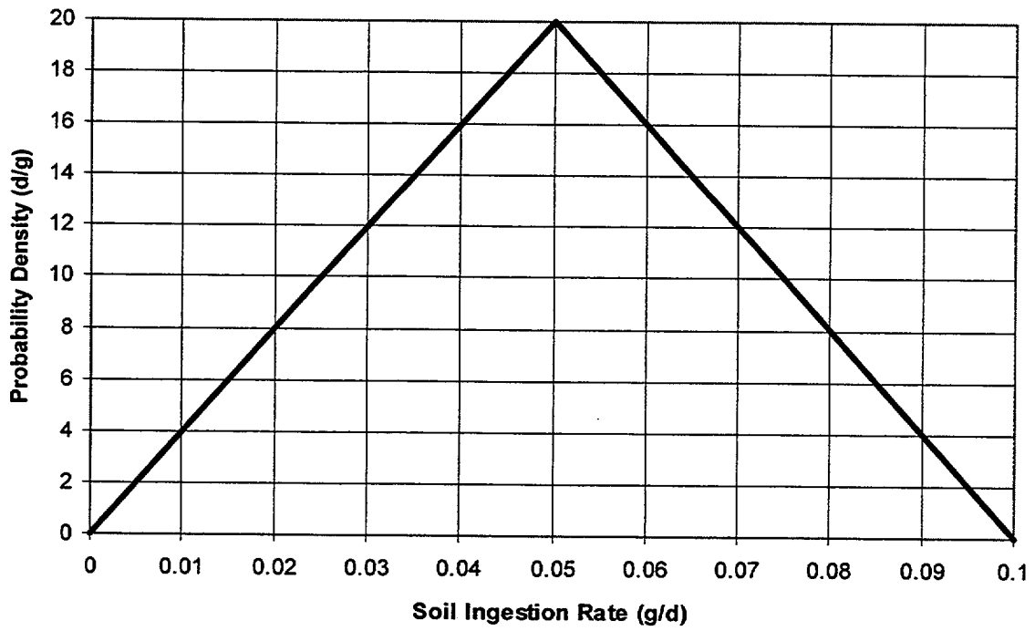
Figure 6.12 Probability density function for GR
