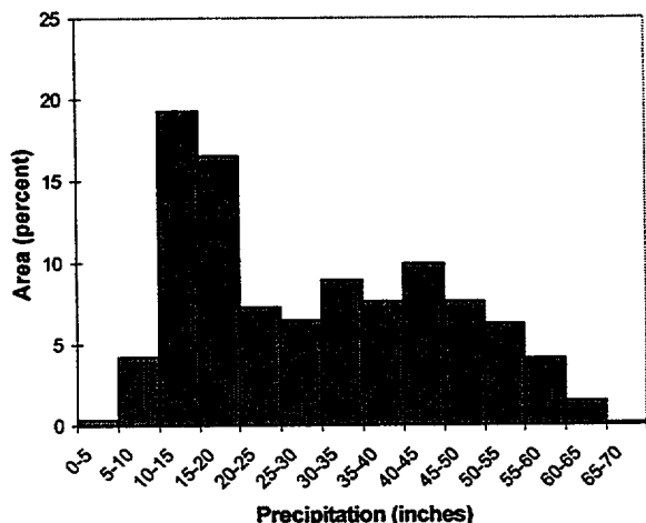
Figure 6.24 PDF for precipitation
