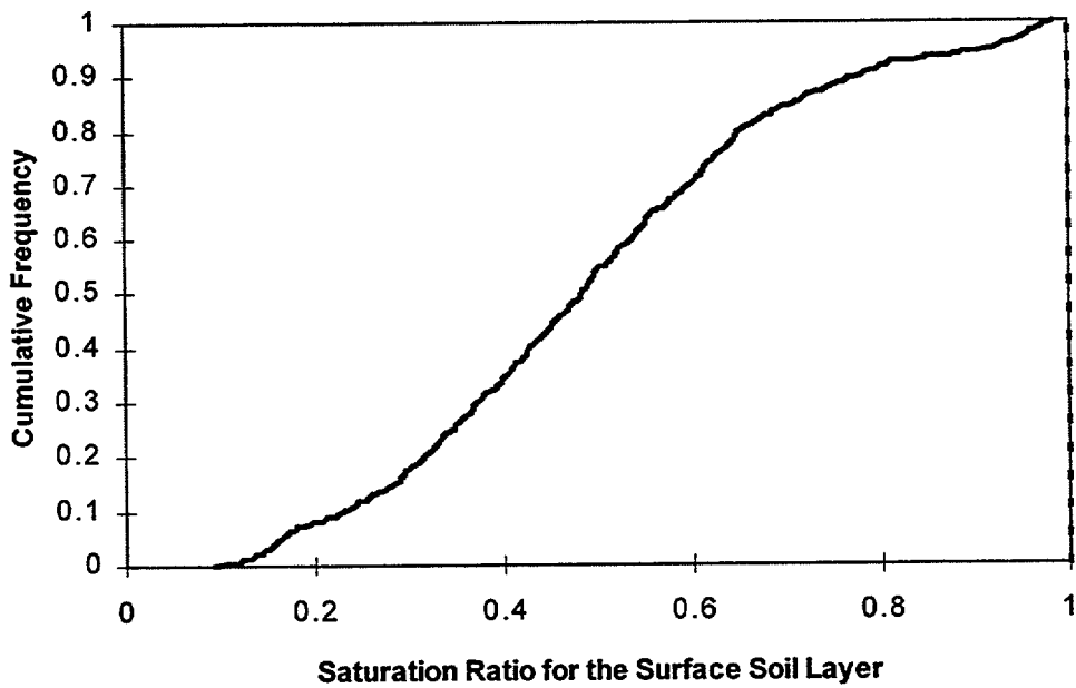
Figure 6.69 Cumulative frequency of sampled f1 values (NUREG/CR-5512, Vol. 1, default shown as vertical dashed line)
