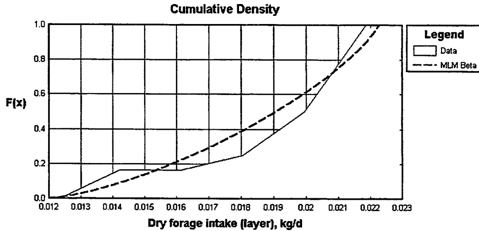
Figure 6.58 Cumulative distribution for forage consumed by layer hens
