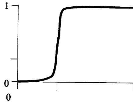
Figure 2 Solution count distributions (SCDs) for three idealized relationships among source constraints
