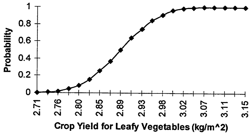
Figure 6.27 Cumulative distribution for Y, (leafy vegetables)
