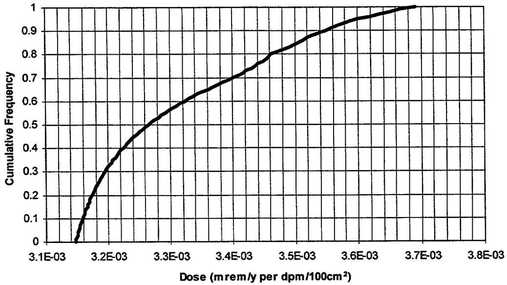
Figure 5.9 Calculated distribution of dose to the average member of the screening group due to a unit source of Co-60
