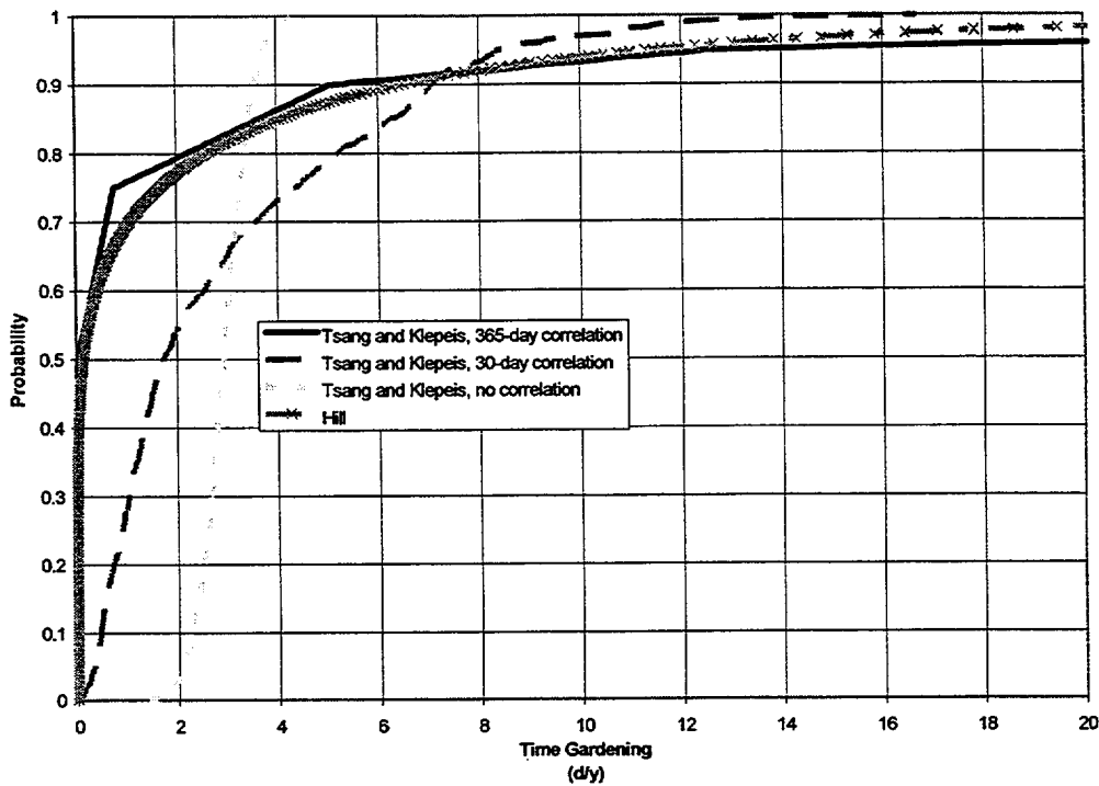
Figure 6.4 CDF of annual average time spent gardening based on data from Hill (1985) and daily data from Tsang and Klepeis (1996) for three assumed autocorrelations
