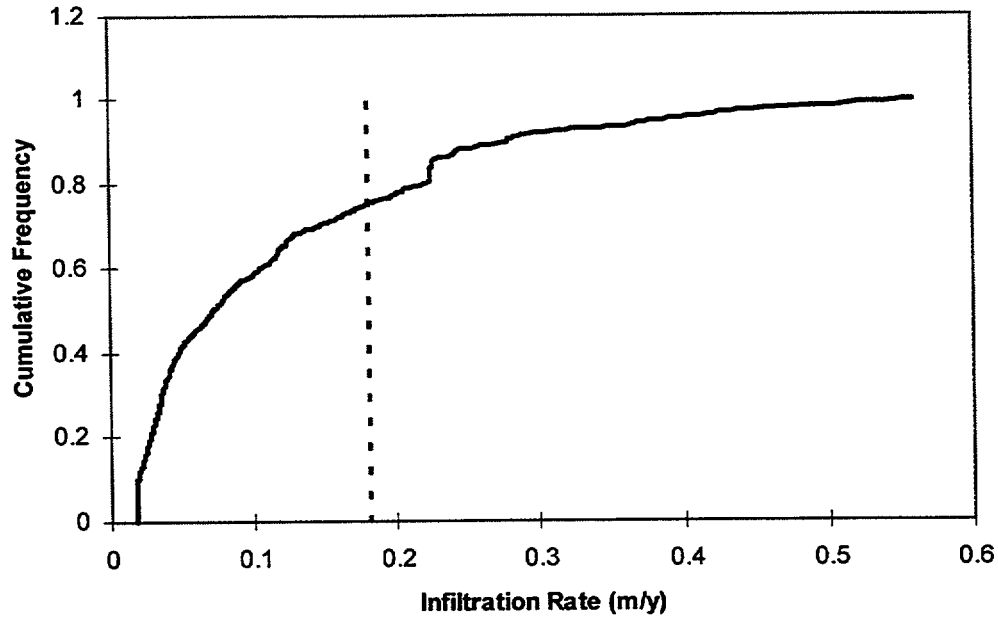
Figure 6.70 Cumulative frequency of sampled IR values (NUREG/CR-5512, Vol. 1, default shown as vertical dashed line)
