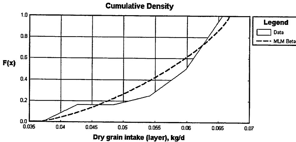
Figure 6.59 Cumulative distribution for stored grain consumed by layer hens
