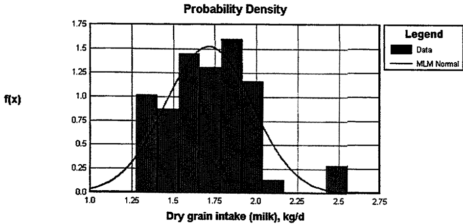
Figure 6.47 Calculated probability distribution for stored grain consumed by dairy cattle
