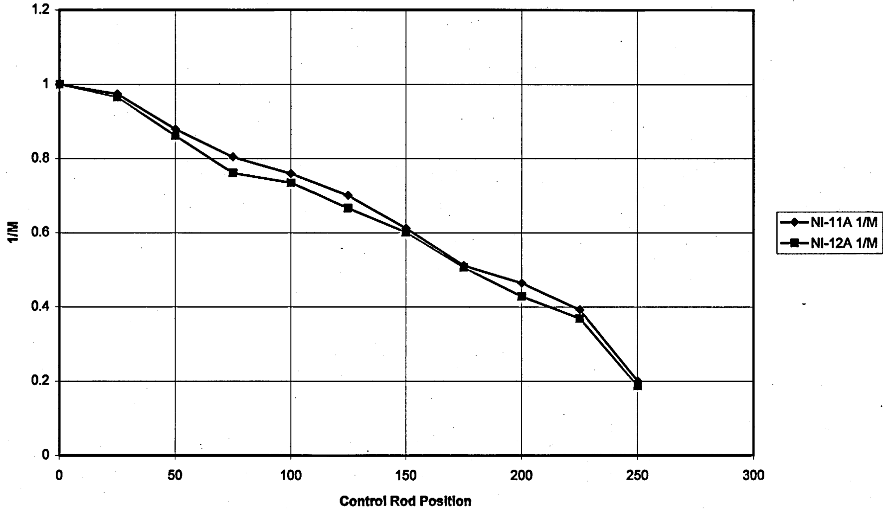
Figure 3.1-1 1/M vs. CRG Position
