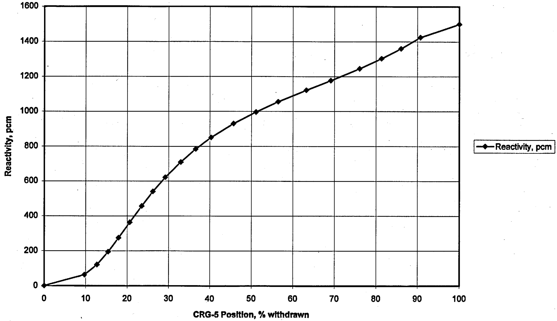
Figure 3.6-2 Integral Worth for CRG-5
