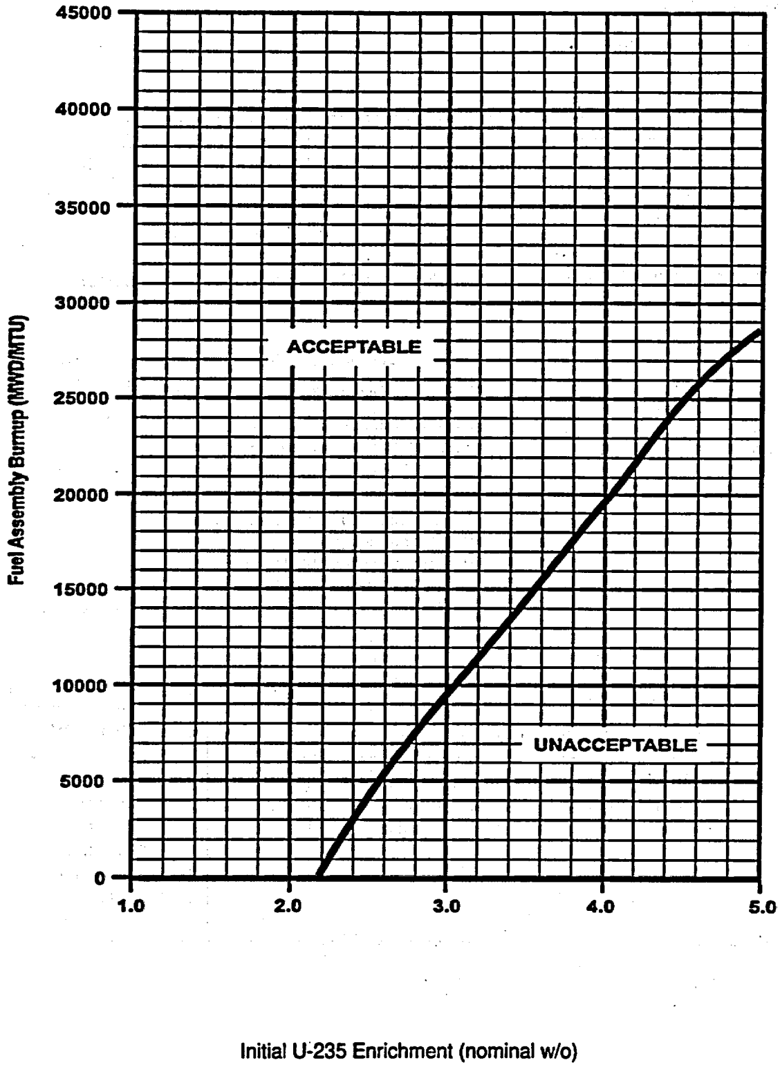
Figure 3.7.15-1 Fuel Assembly Burnup Limit Requirements For All Cell Storage
