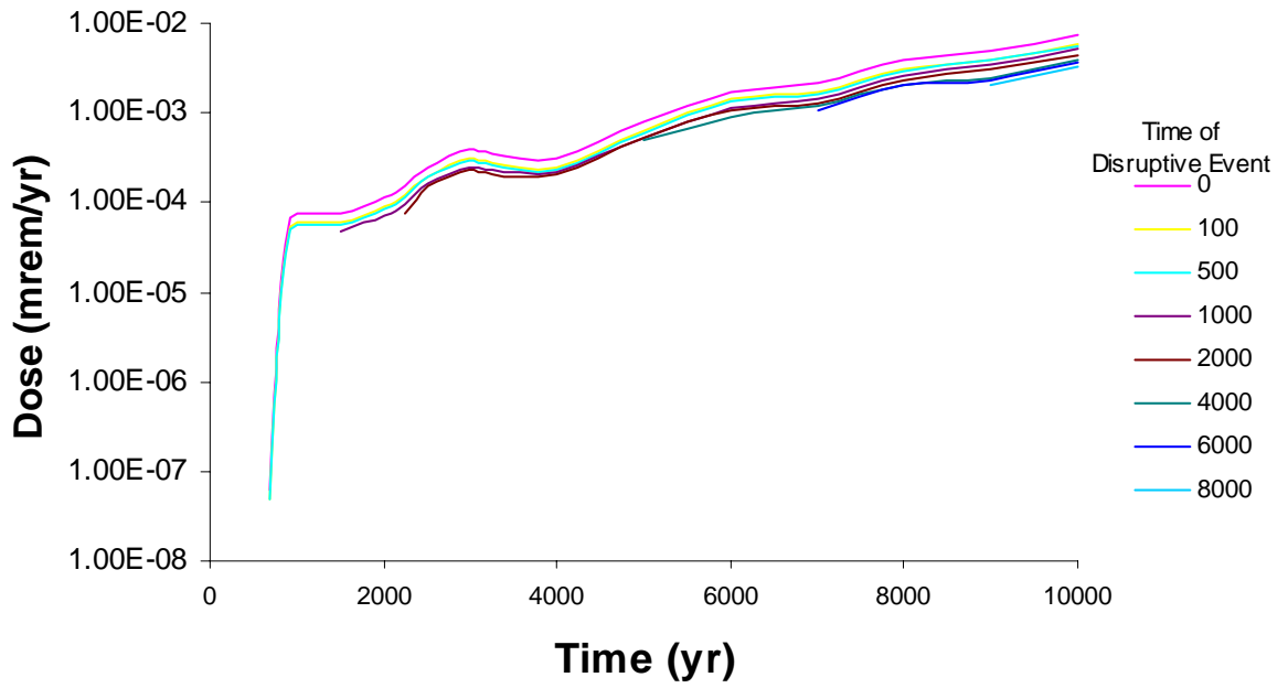
Figure 20. Scenario class dose history for scenario class \Theta based on time of occurrence of the disruptive event
