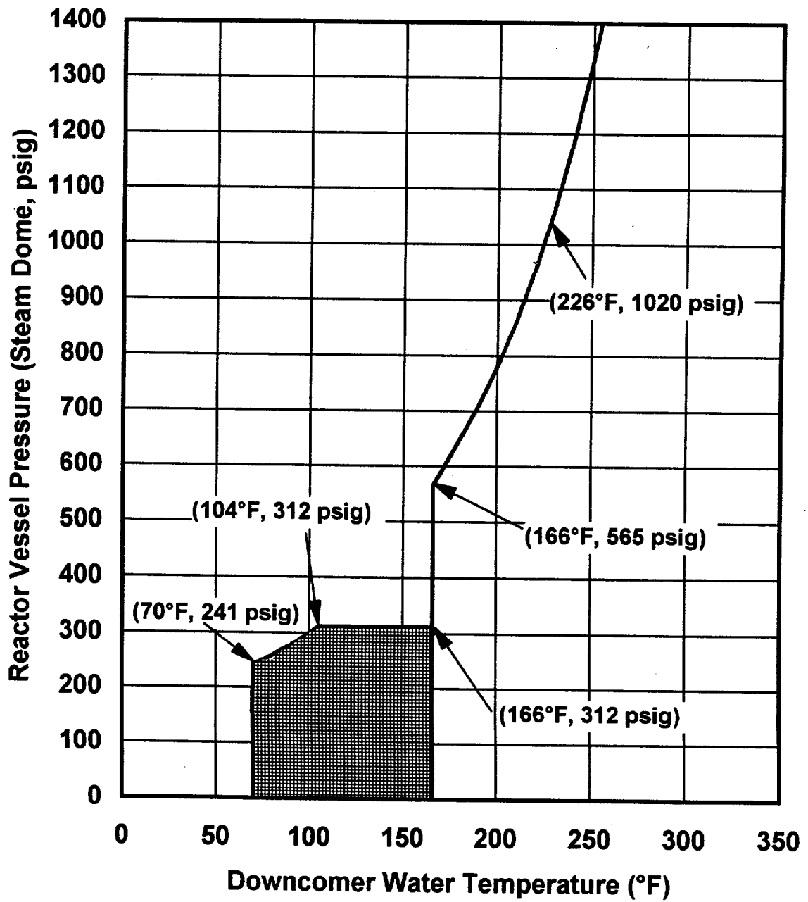
Figure 3.4.11-5 (Page 1 of 1) Nuclear Cooldown Curve
