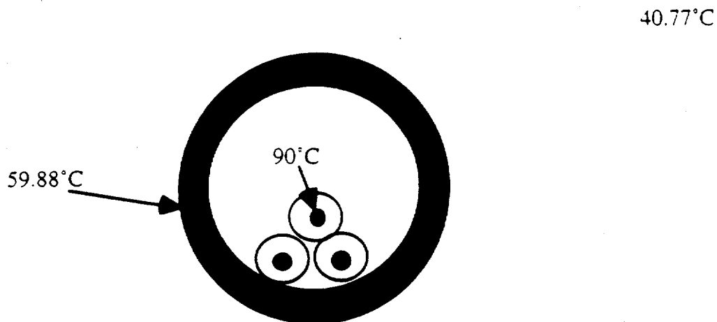
Figure A1: Schematic for calculation of conduit heat losses Source: Tanaka, 1994
