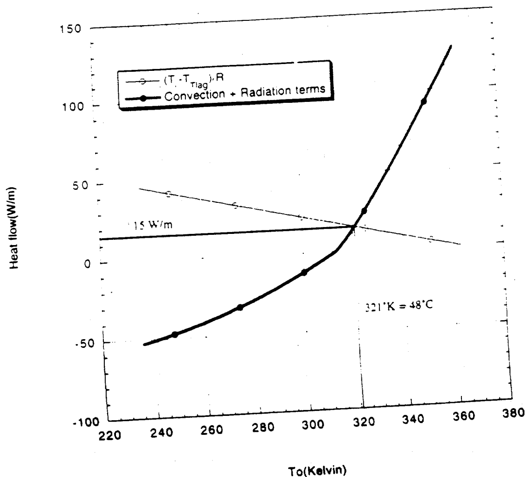
Figure A2: Protected 1-Inch Conduit Heat Flow Solution Source: Tanaka, 1994
