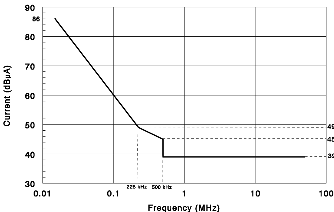
Figure 5.3 CE03 Narrowband Emissions Envelope
