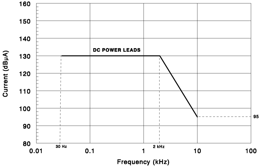
Figure 4.1 CE101 Emissions Envelopes for dc Power Leads
