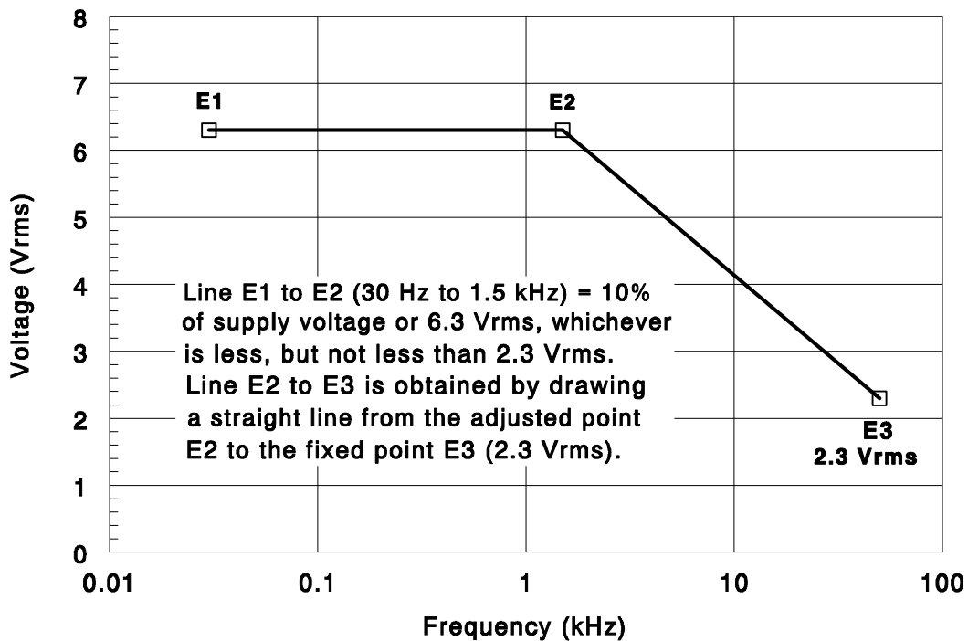
Figure 5.4 CS01 Operating Envelope
