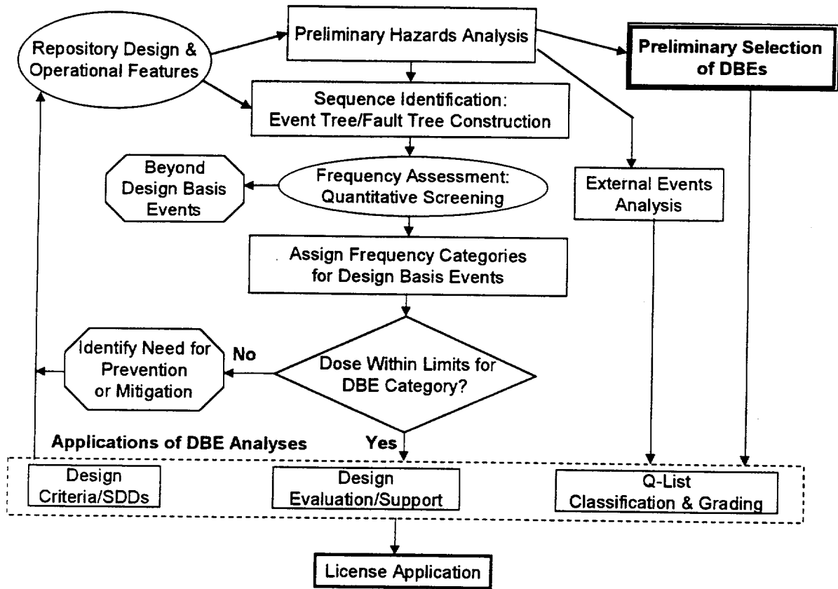
Figure 1. Integrated Safety Analysis Process (Preclosure)
