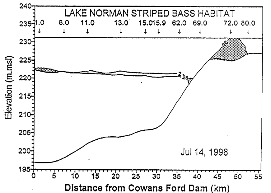
Figure 2-11. Striped bass habitat (temperatures \leq 26 C and dissolved oxygen \geq 2.0 mg/L in Lake Norman in June, July, August, September and October 1998.
