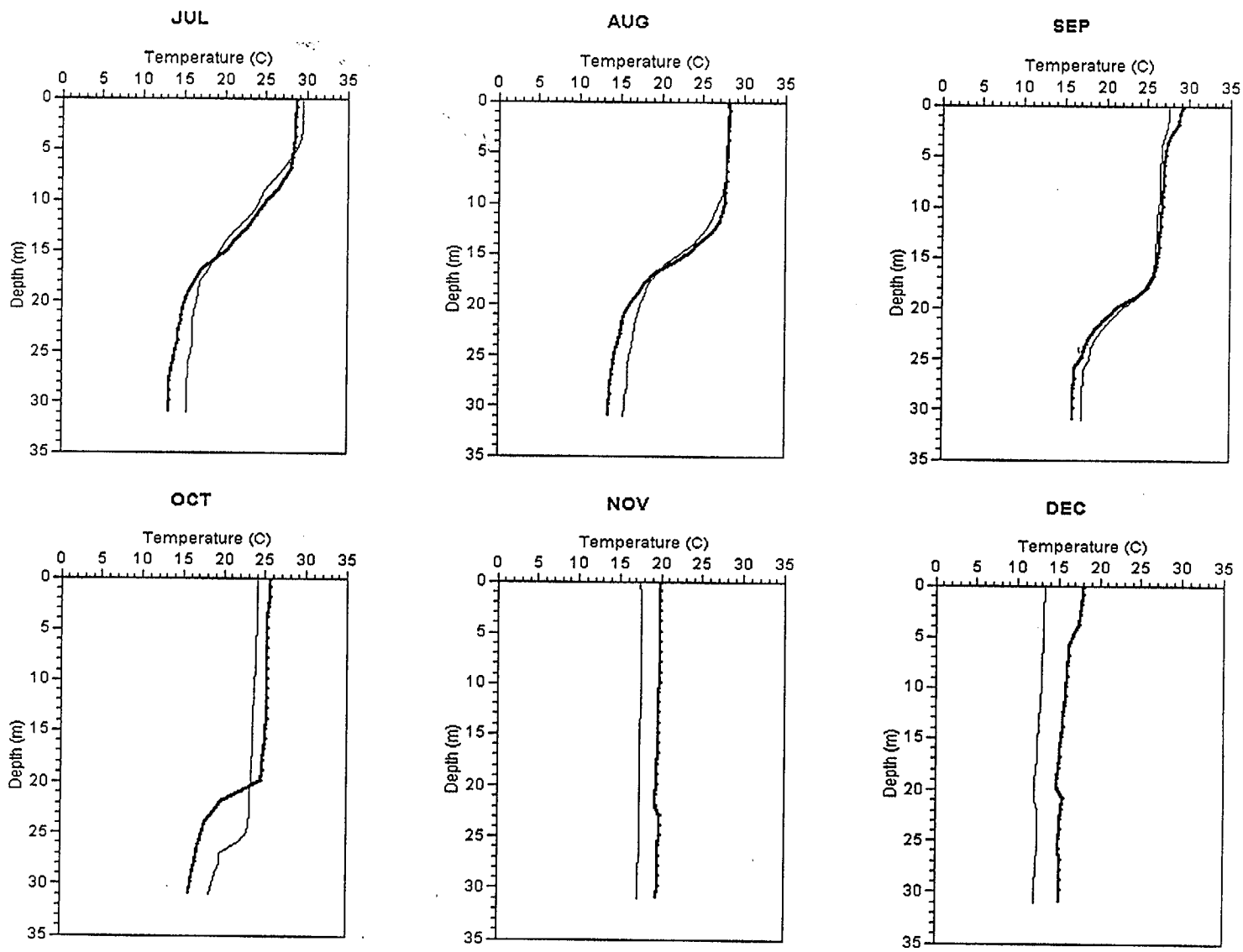
Figure 2-3. Monthly mean temperature profiles for McGuire Nuclear Station background zone in 1997 (—) and 1998 (---).
