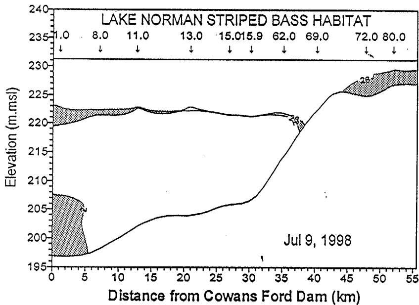
Figure 2-11. Striped bass habitat (temperatures \leq 26 C and dissolved oxygen \geq 2.0 mg/L in Lake Norman in June, July, August, September and October 1998.
