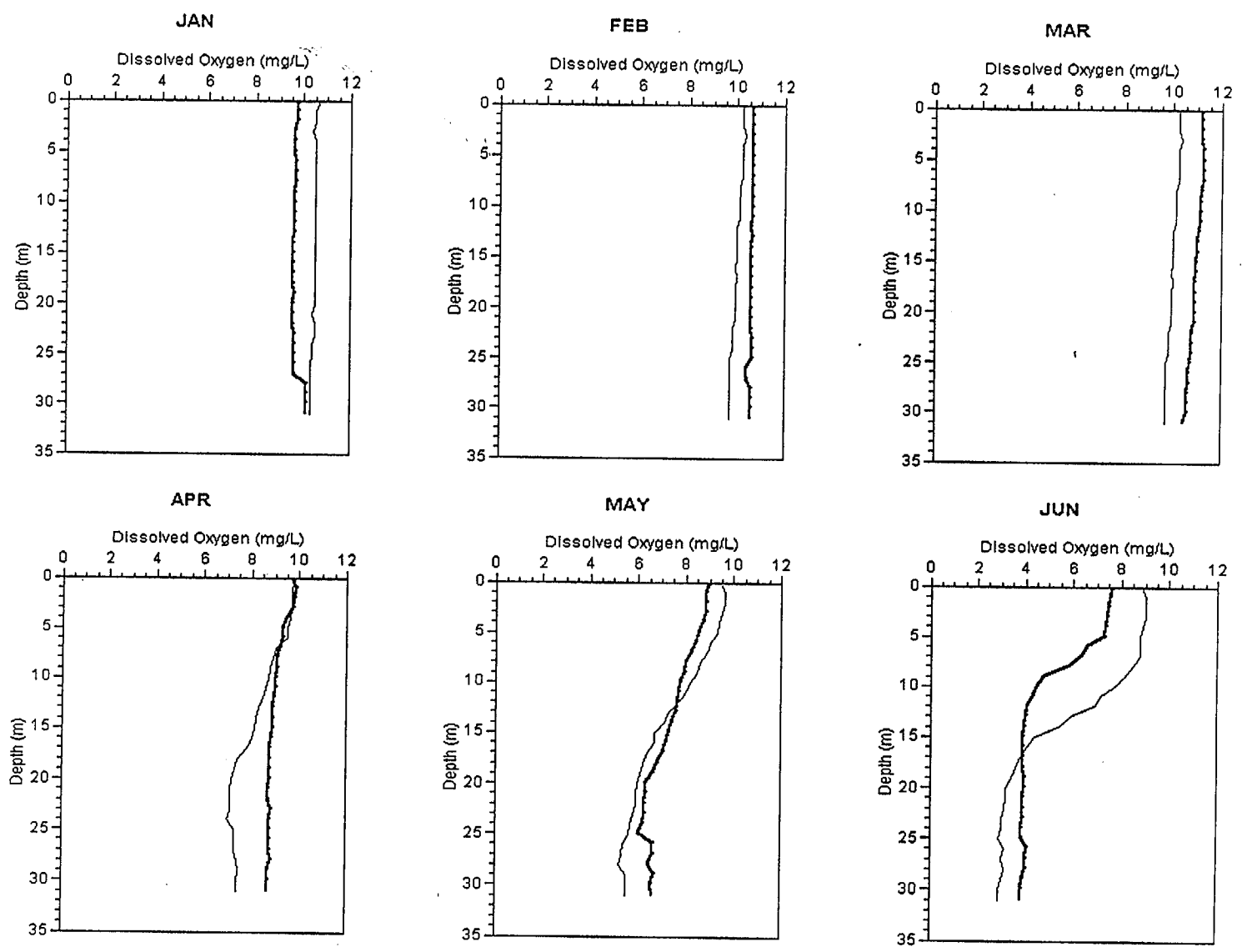
Figure 2-6. Monthly mean dissolved oxygen profiles for the McGuire Nuclear Station background zone in 1997 (—) and 1998 (—).
