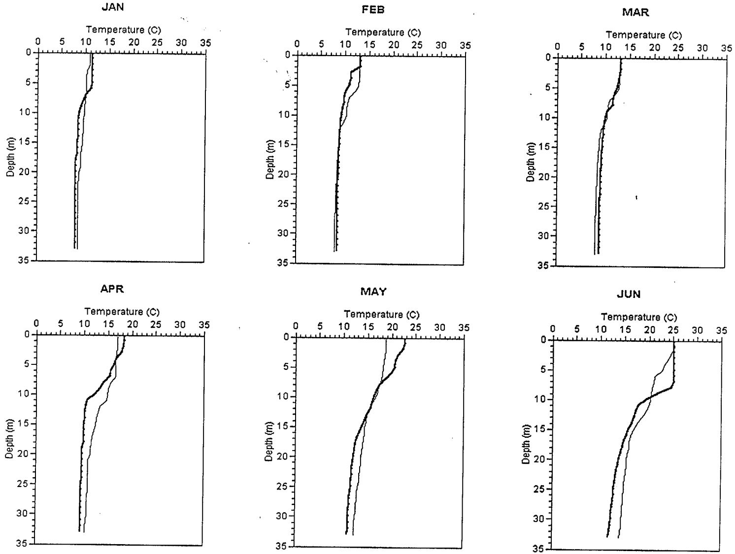
Figure 2-4. Monthly mean temperature profiles for the McGuire Nuclear Station mixing zone in 1997 (—) and 1998 (---).
