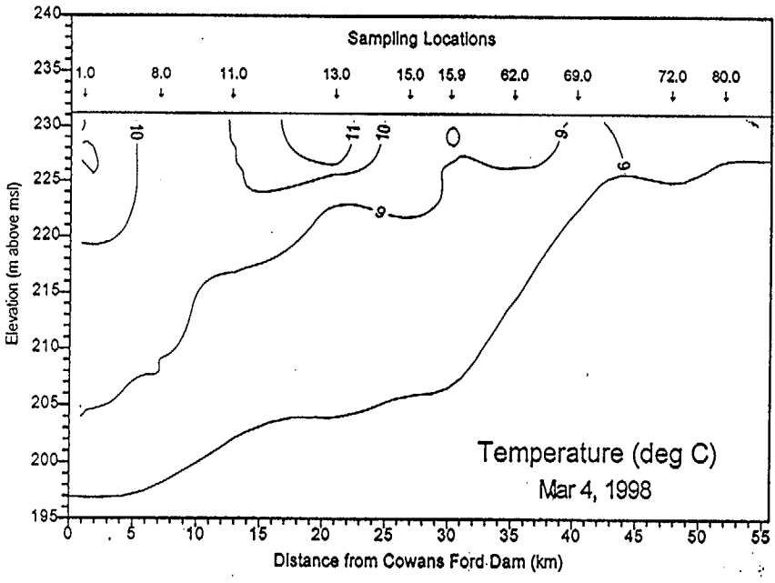
Figure 2-8. Monthly reservoir-wide temperature isotherms for Lake Norman in 1998.
