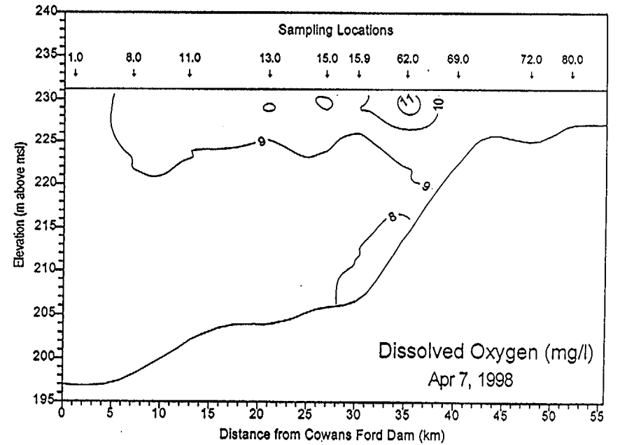
Figure 2-9. Monthly reservoir-wide dissolved oxygen isopleths for Lake Norman in 1998.
