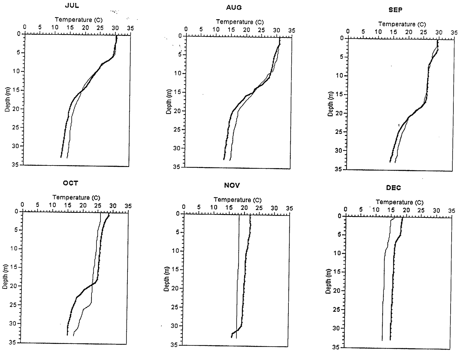
Figure 2-4. Monthly mean temperature profiles for the McGuire Nuclear Station mixing zone in 1997 (—) and 1998 (▲).
