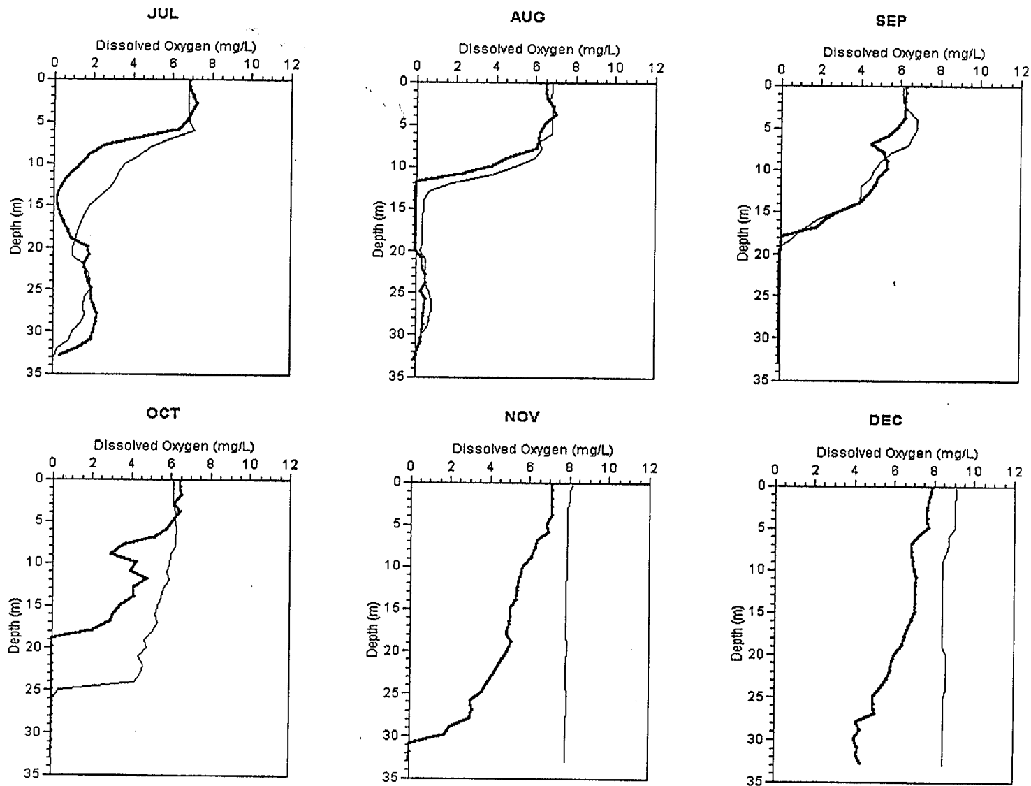
Figure 2-7. Monthly mean dissolved oxygen profiles for the McGuire Nuclear Station mixing zone in 1997 (—) and 1998 (---).
