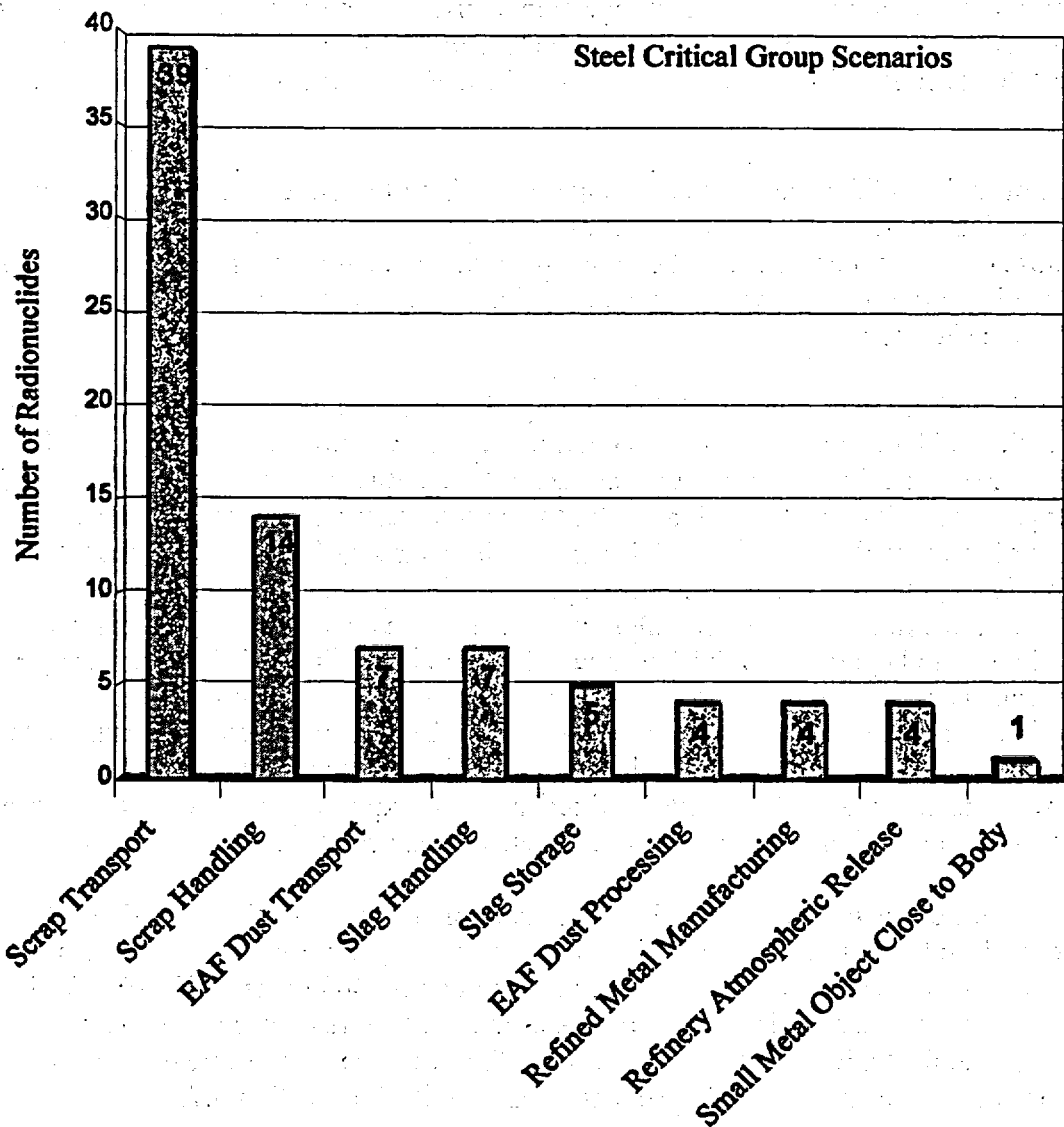
Figure 4.7 Scenarios describing critical groups for steel recycle
