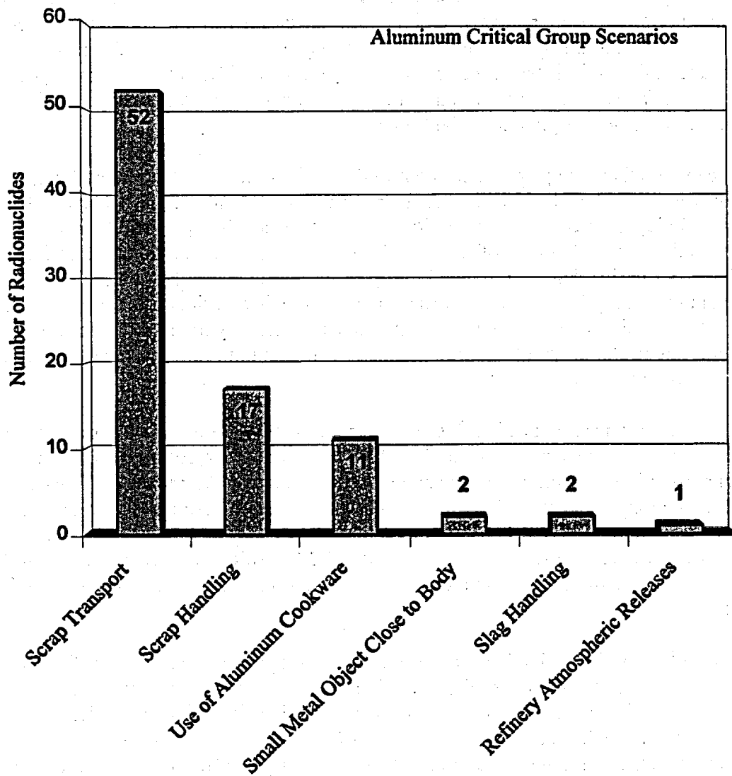
Figure 6.2 Scenarios describing critical groups for aluminum recycle
