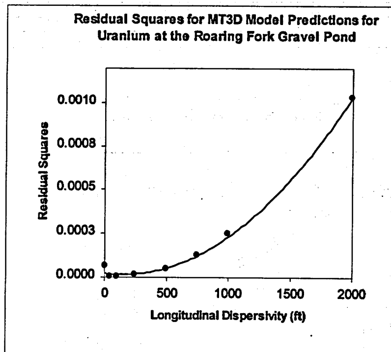
Figure 12. MT3D Calibration—Longitudinal Dispersivity Prediction
