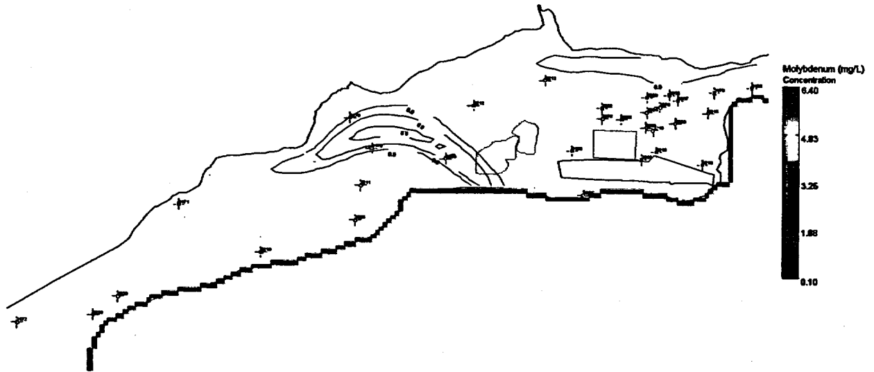
Figure 67. Predicted Molybdenum Concentrations in the Ground Water at the New Rifle Site at 25 Years—100 Simulations
