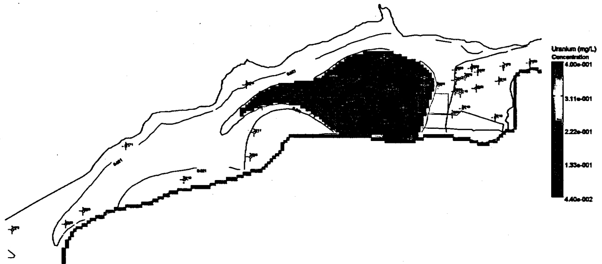
Figure 34. Predicted Uranium Concentrations in the Ground Water at the New Rifle Site at 20 Years — 100 Simulations
