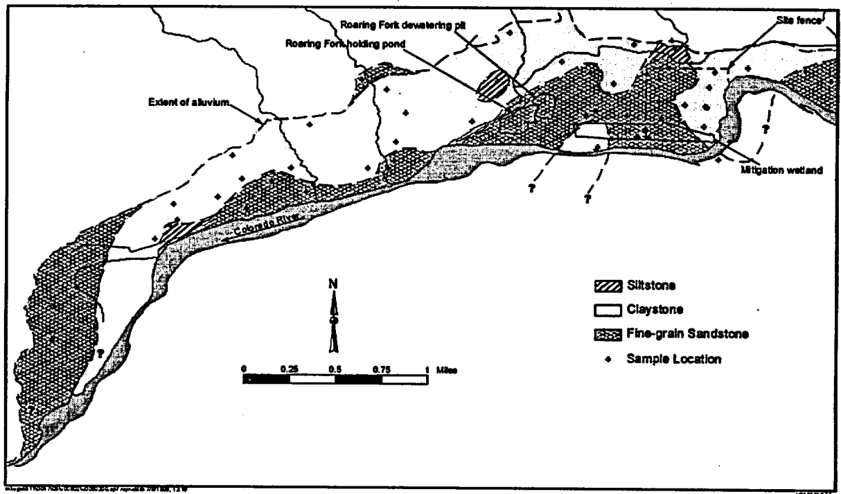
Figure 5-15. Areal Characteristics of Subsurface Bedrock Units
