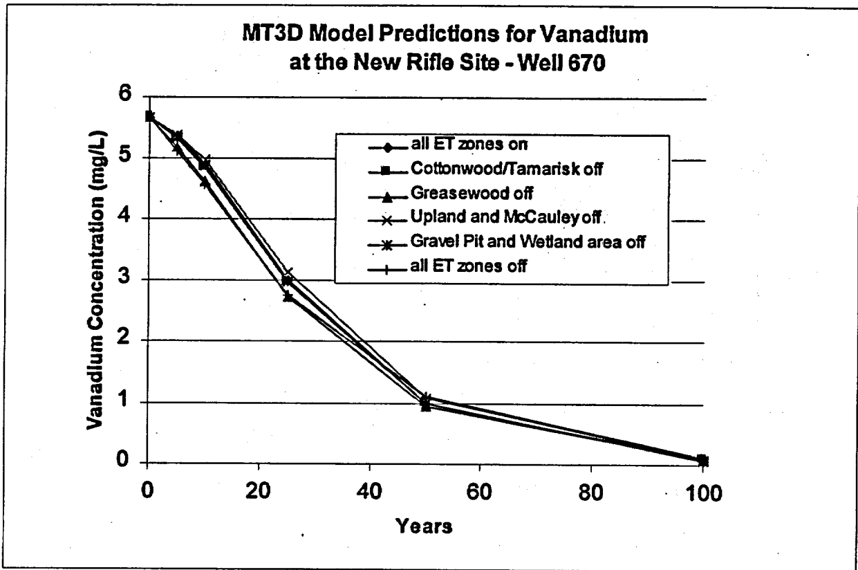
Figure 19. MT3D Sensitivity Analysis—ET
