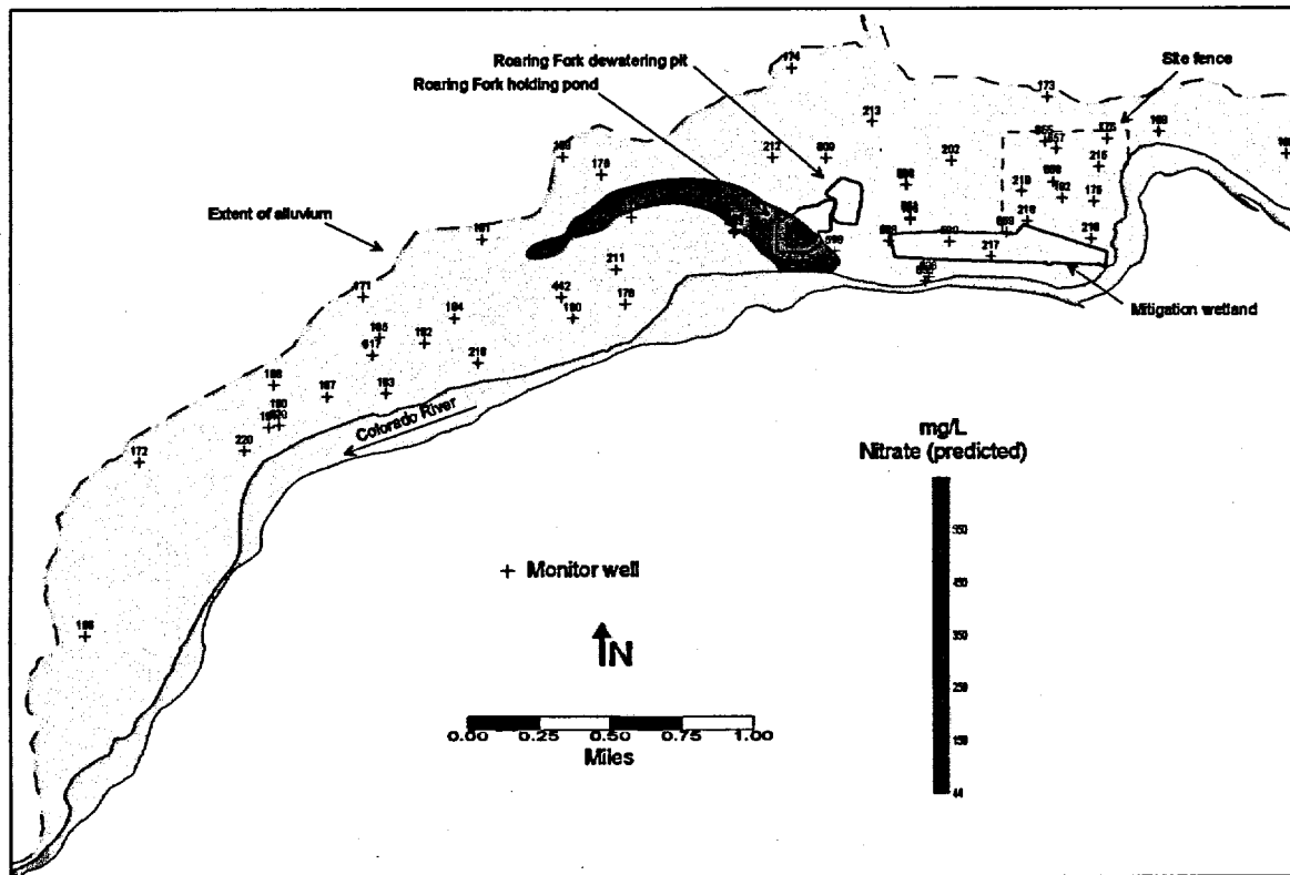
Figure 5-50. Predicted Nitrate Concentrations in the Ground Water at the New Rifle Site at 10 Years Based on the August 1998 Sampling Data—100 Simulations
