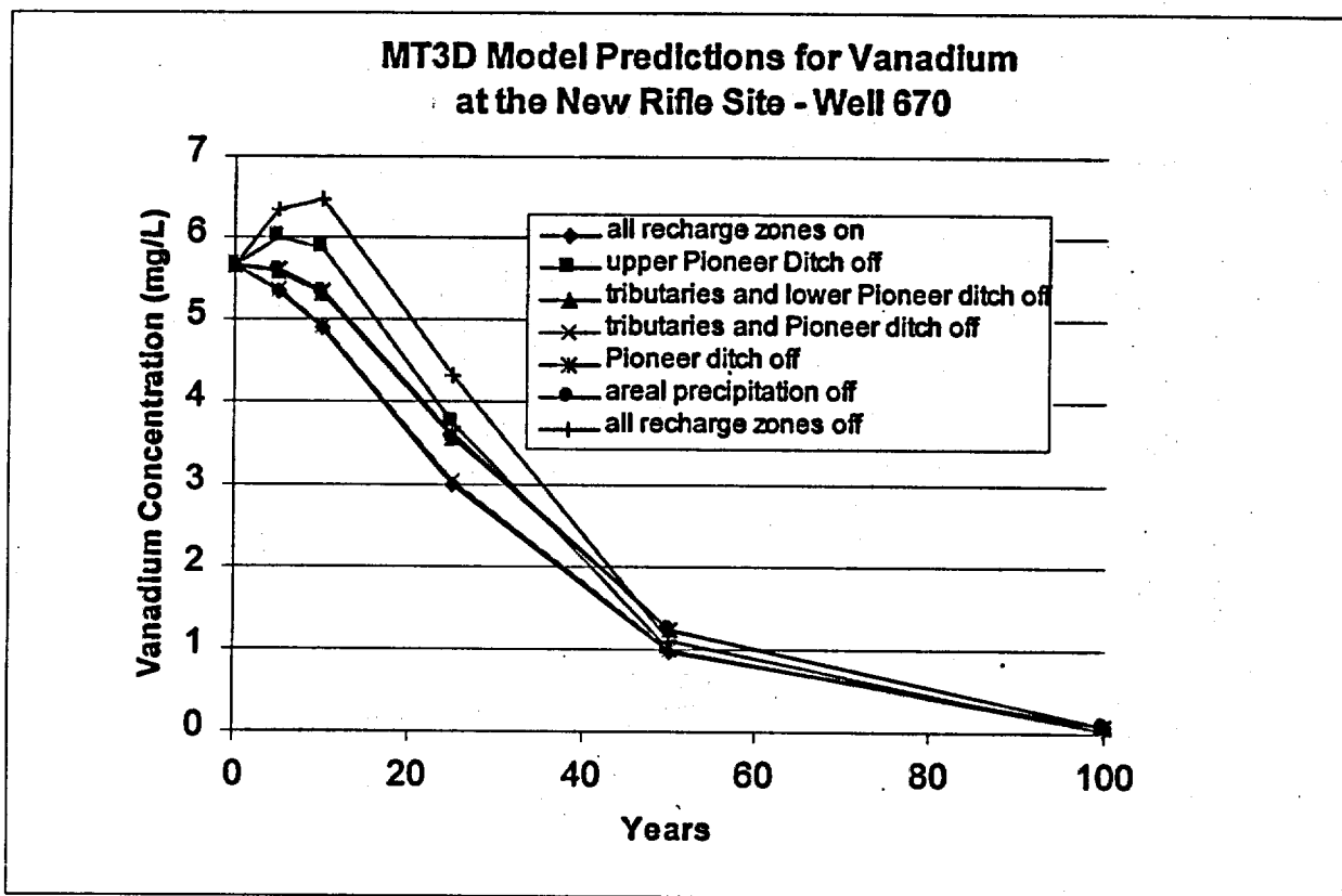
Figure 17. MT3D Sensitivity Analysis—Recharge
