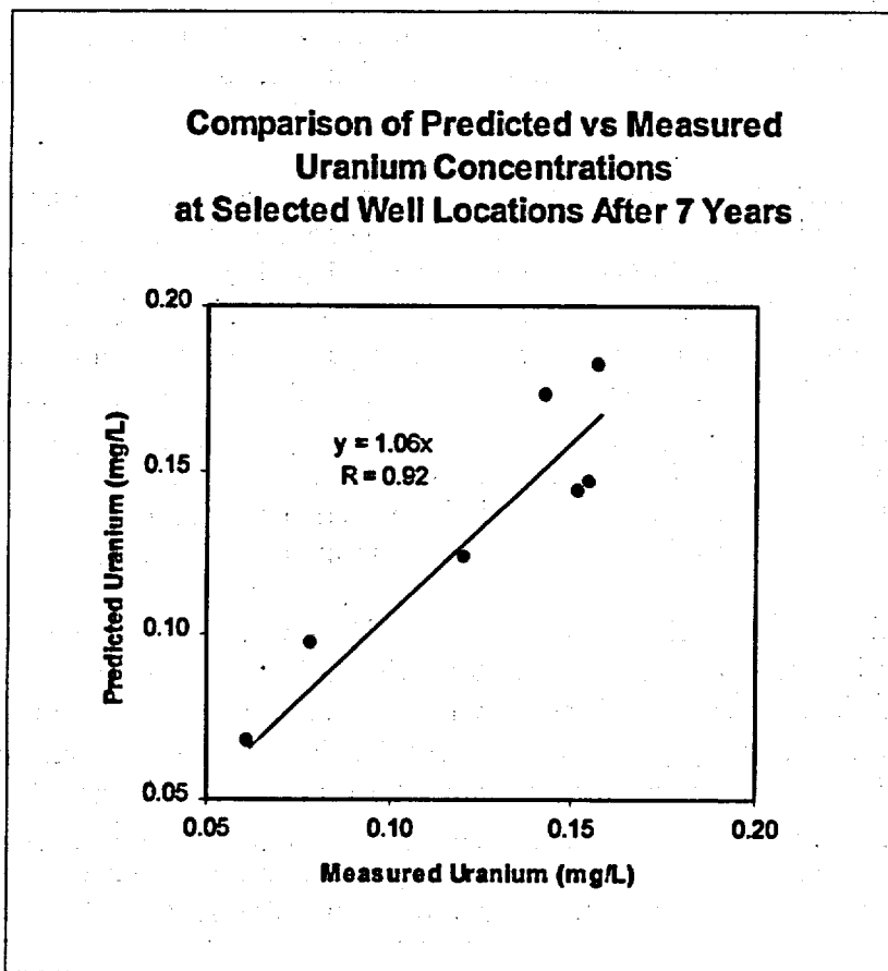
Figure 13. MT3D Calibration—Longitudinal Dispersivity Selected Wells Verification
