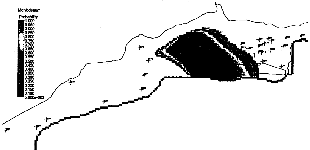
Figure 69. Probability of Molybdenum Concentrations Exceeding the 0.1 mg/L UMTRA Ground Water Standard at the New Rifle Site at 10 Years
