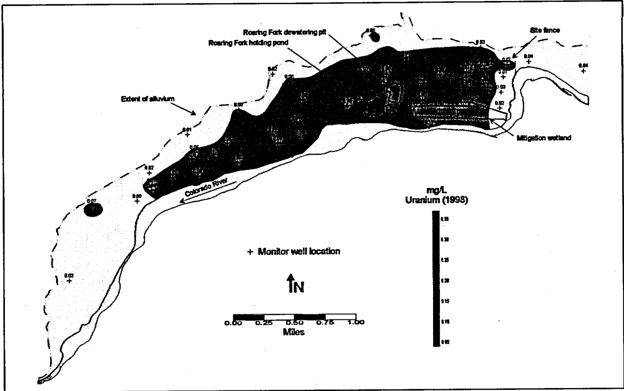
Figure 5-36. Uranium Distribution in Alluvial Ground Water—New Rifle, 1998
