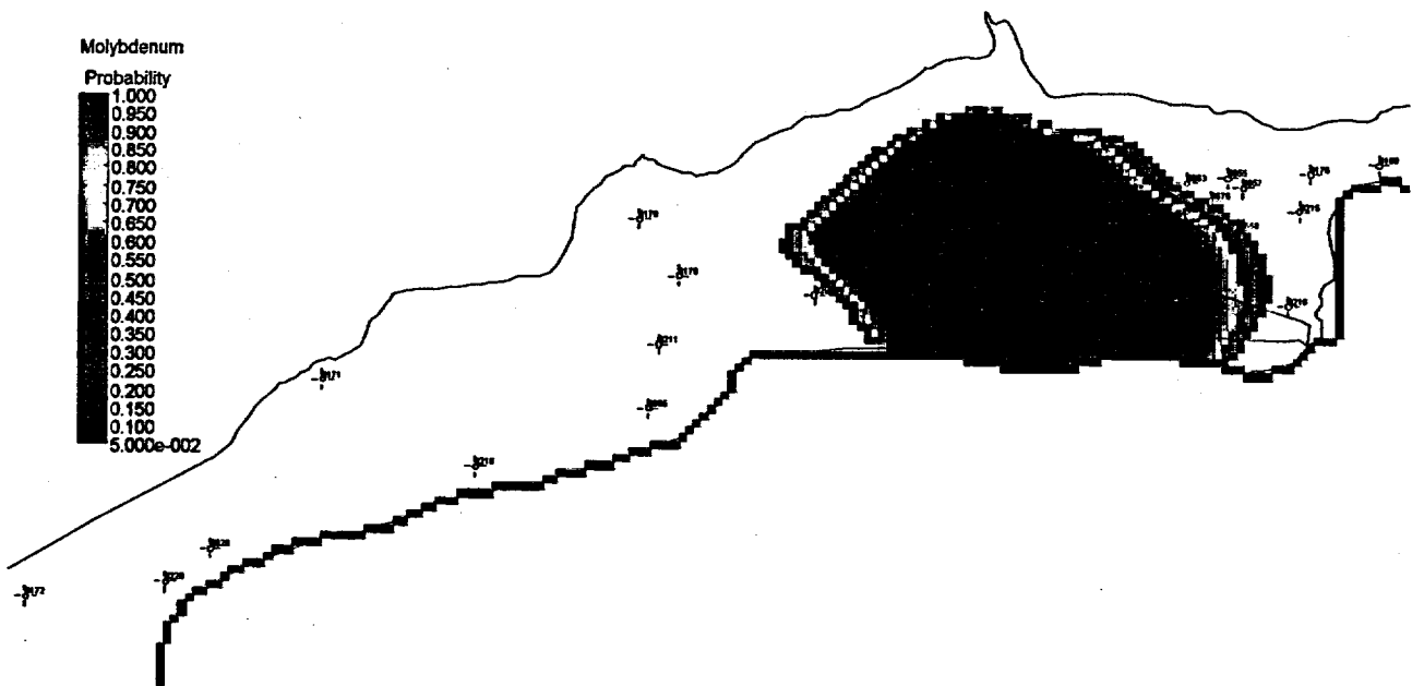
Figure 68. Probability of Molybdenum Concentrations Exceeding the 0.1 mg/L UMTRA Ground Water Standard at the New Rifle Site at 5 Years
