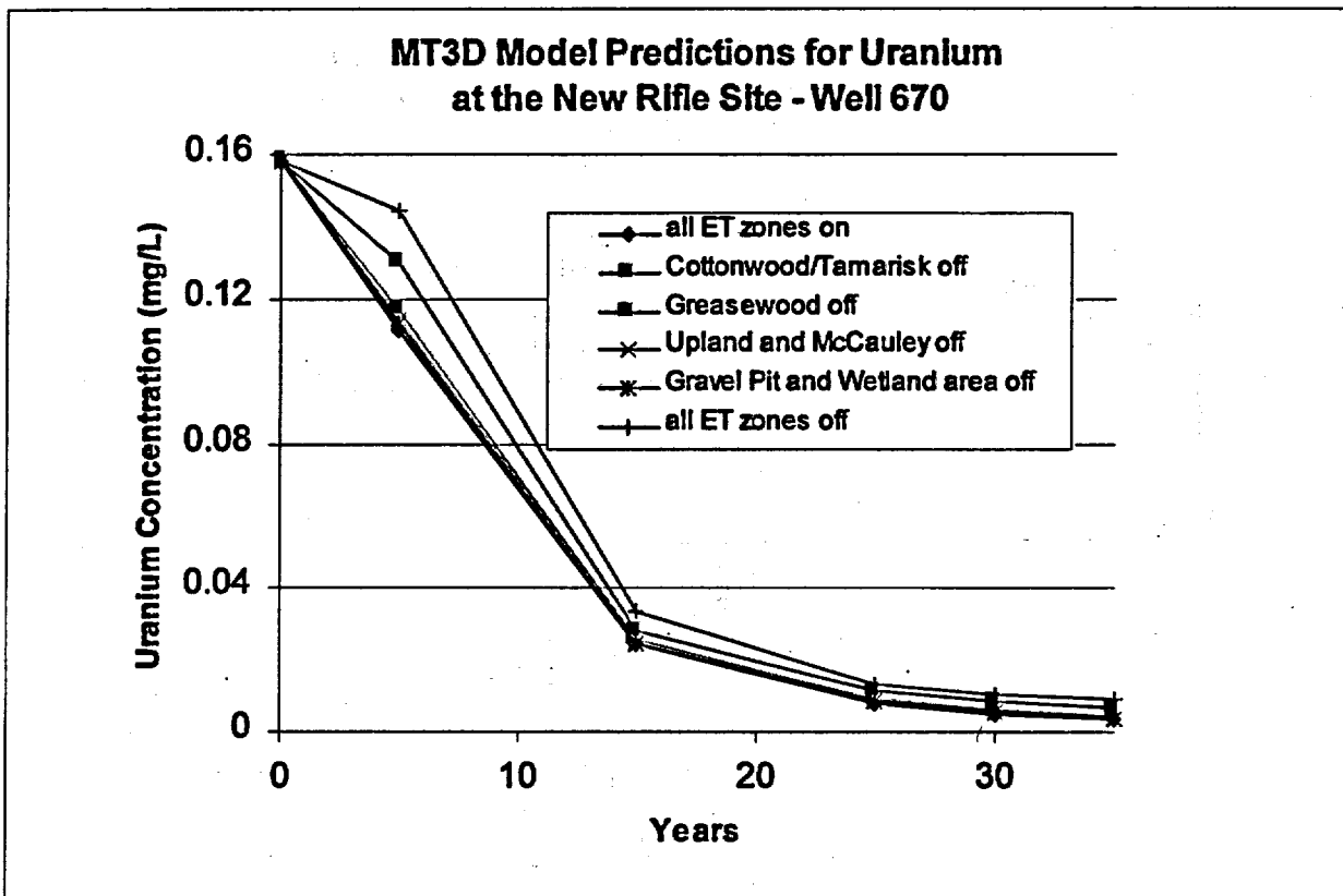
Figure 18. MT3D Sensitivity Analysis—ET
