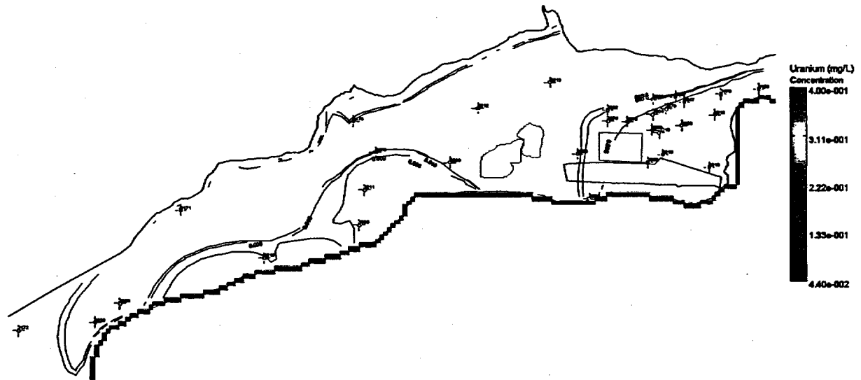
Figure 36. Predicted Uranium Concentrations in the Ground Water at the New Rifle Site at 40 Years —100 Simulations
