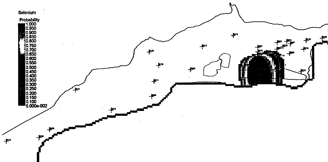
Figure 59. Probability of Selenium Concentrations Exceeding the 0.05 mg/L SDWA Ground Water Standard at the New Rifle Site at 50 Years
