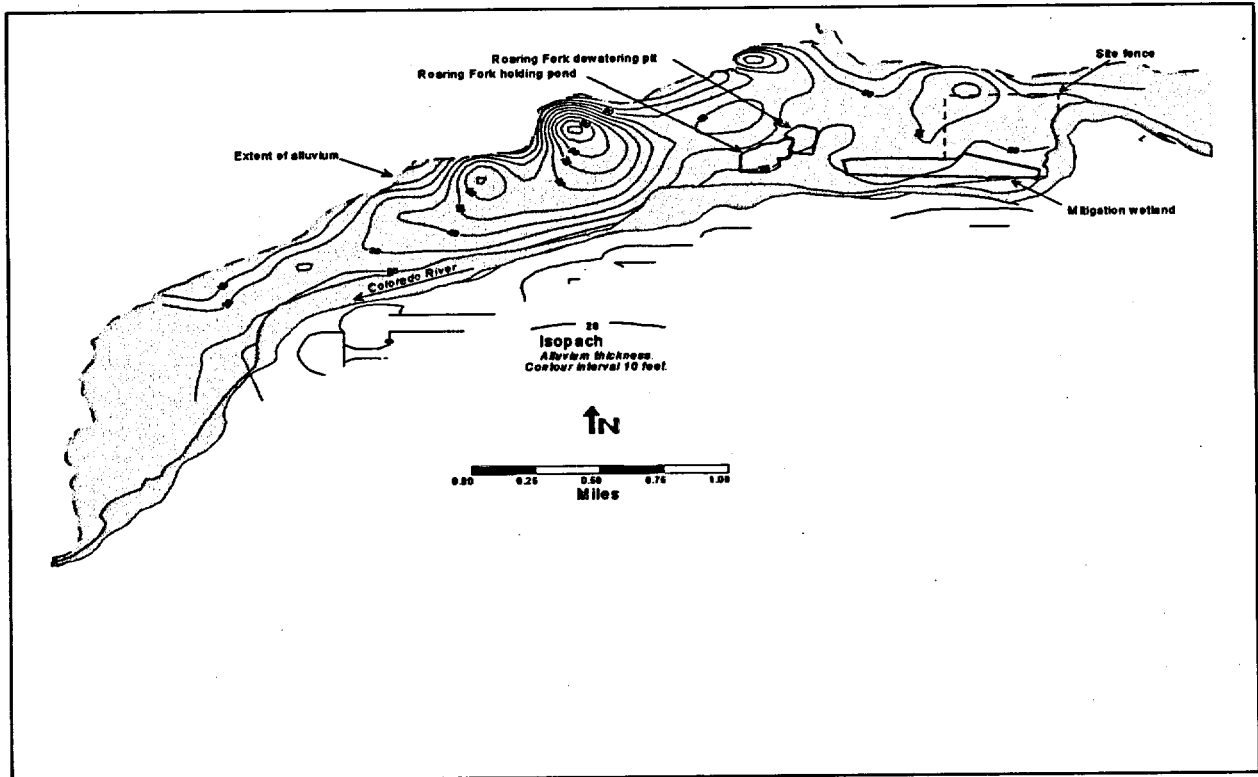
Figure 5-6. Isopach Map of the Alluvium at the New Rifle Site
