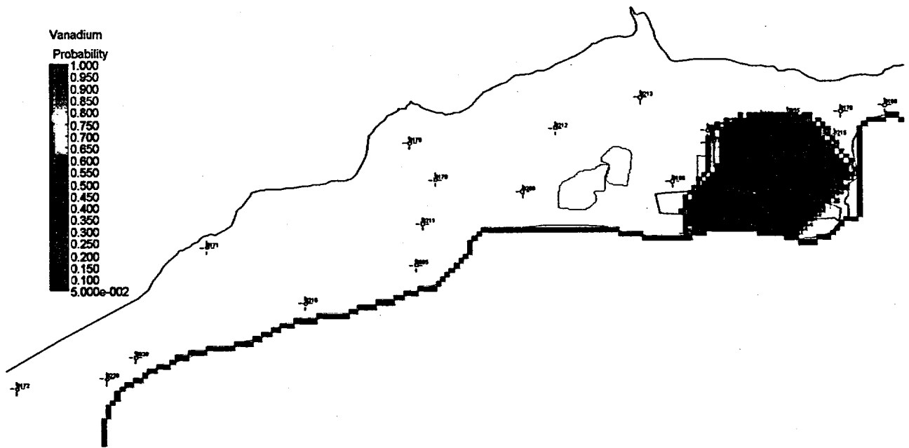
Figure 45. Probability of Vanadium Concentrations Exceeding the 0.33 mg/L Proposed Ground Water Cleanup Goal at the New Rifle Site at 25 Years
