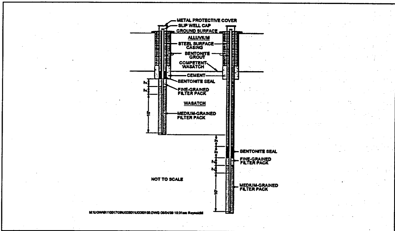
Figure 4-3. Completion Diagram for Shallow and Deep Wells Installed in the Wasatch Formation
