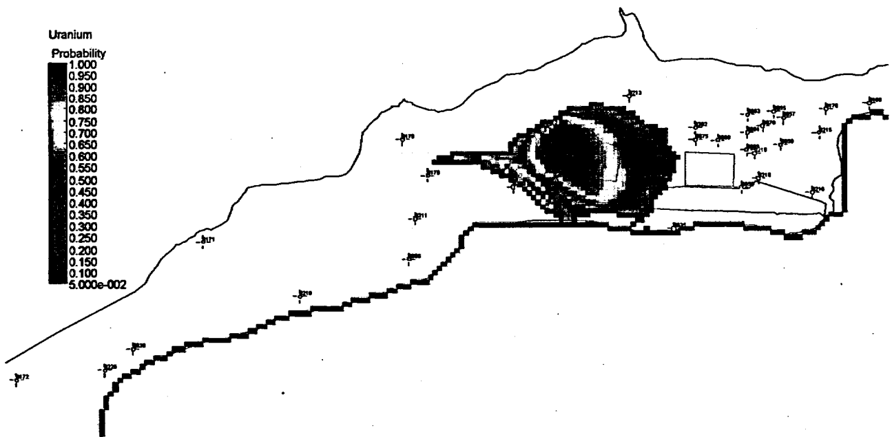
Figure 39. Probability of Uranium Concentrations Exceeding the 0.044 mg/L UMTRA Ground Water Standard at the New Rifle Site at 30 Years
