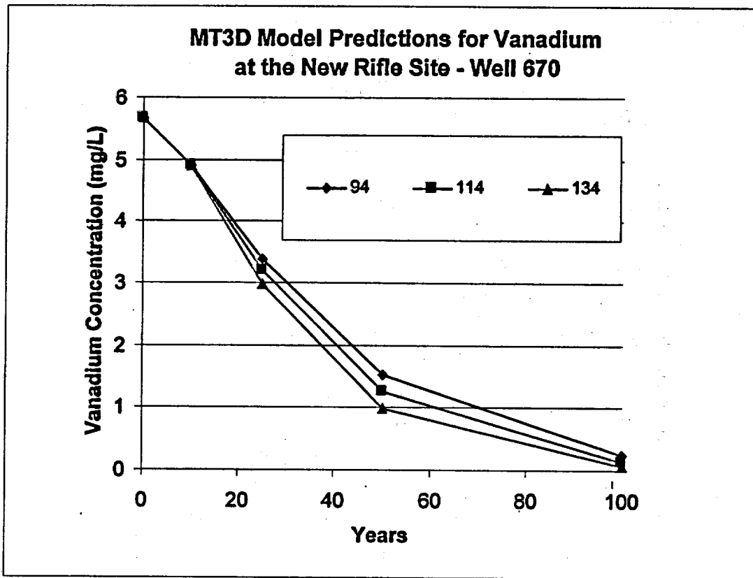
Figure 15. MT3D Sensitivity Analysis—Hydraulic Conductivity ( K_x )
