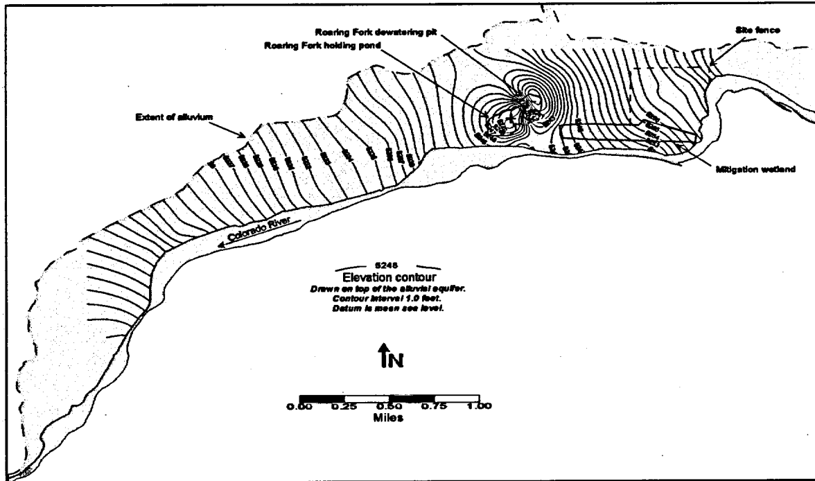
Figure 5-11. Alluvial Ground Water Elevations at the New Rifle Site—January 1999
