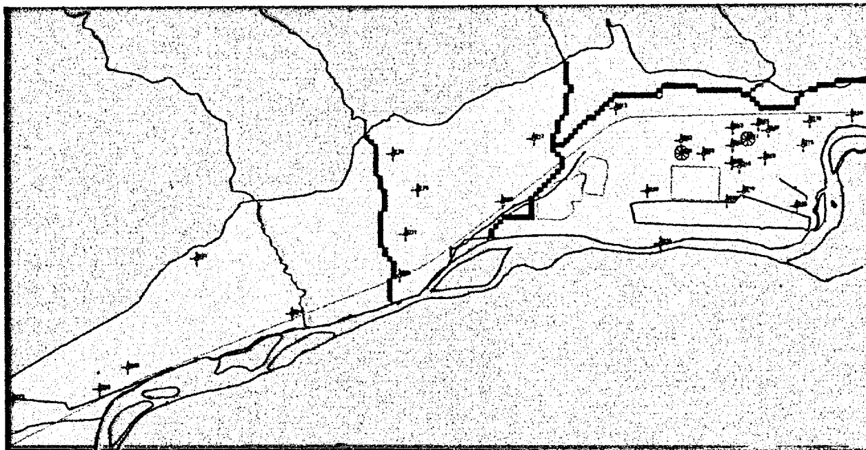
Figure 6. Recharge Zones
