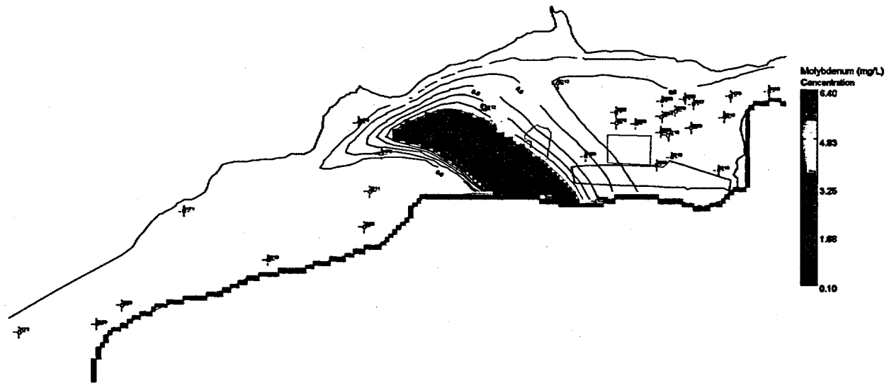
Figure 65. Predicted Molybdenum Concentrations in the Ground Water at the New Rifle Site at 15 Years—100 Simulations
