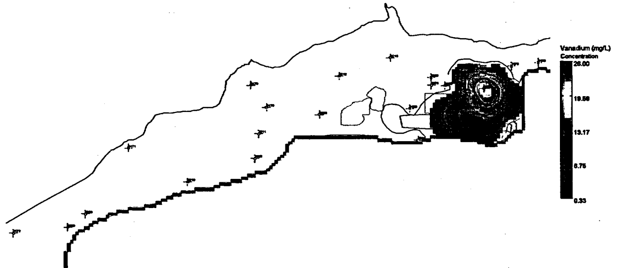
Figure 41. Initial Vanadium Concentrations in the Ground Water at the New Rifle Site Measured in July 1998
