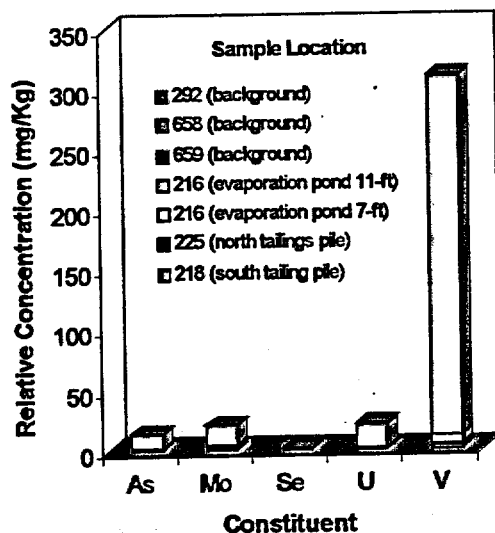
Figure 5-17. Comparison of Constituents Extracted by Synthetic Ground Water from Background and Subpile Soils
