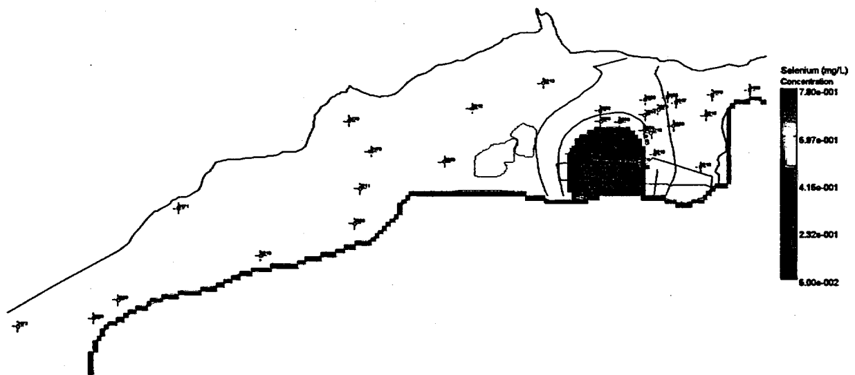
Figure 56. Predicted Selenium Concentrations in the Ground Water at the New Rifle Site at 50 Years —100 Simulations
