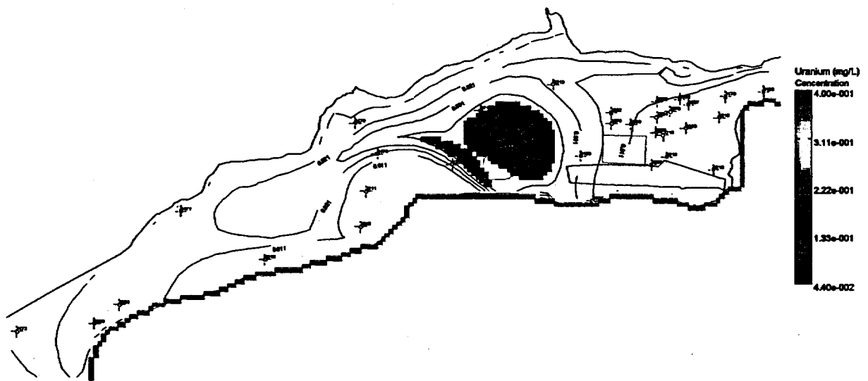
Figure 35. Predicted Uranium Concentrations in the Ground Water at the New Rifle Site at 30 Years — 100 Simulations
