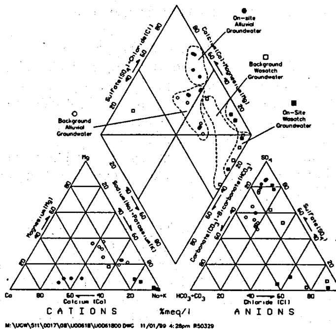
Figure 5-27. Piper Diagram
