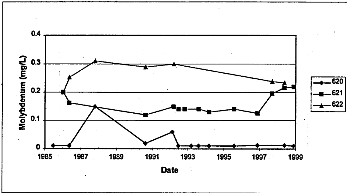
Figure 5-42. Time Concentration Plots for Background Wasatch Ground Water—Molybdenum
