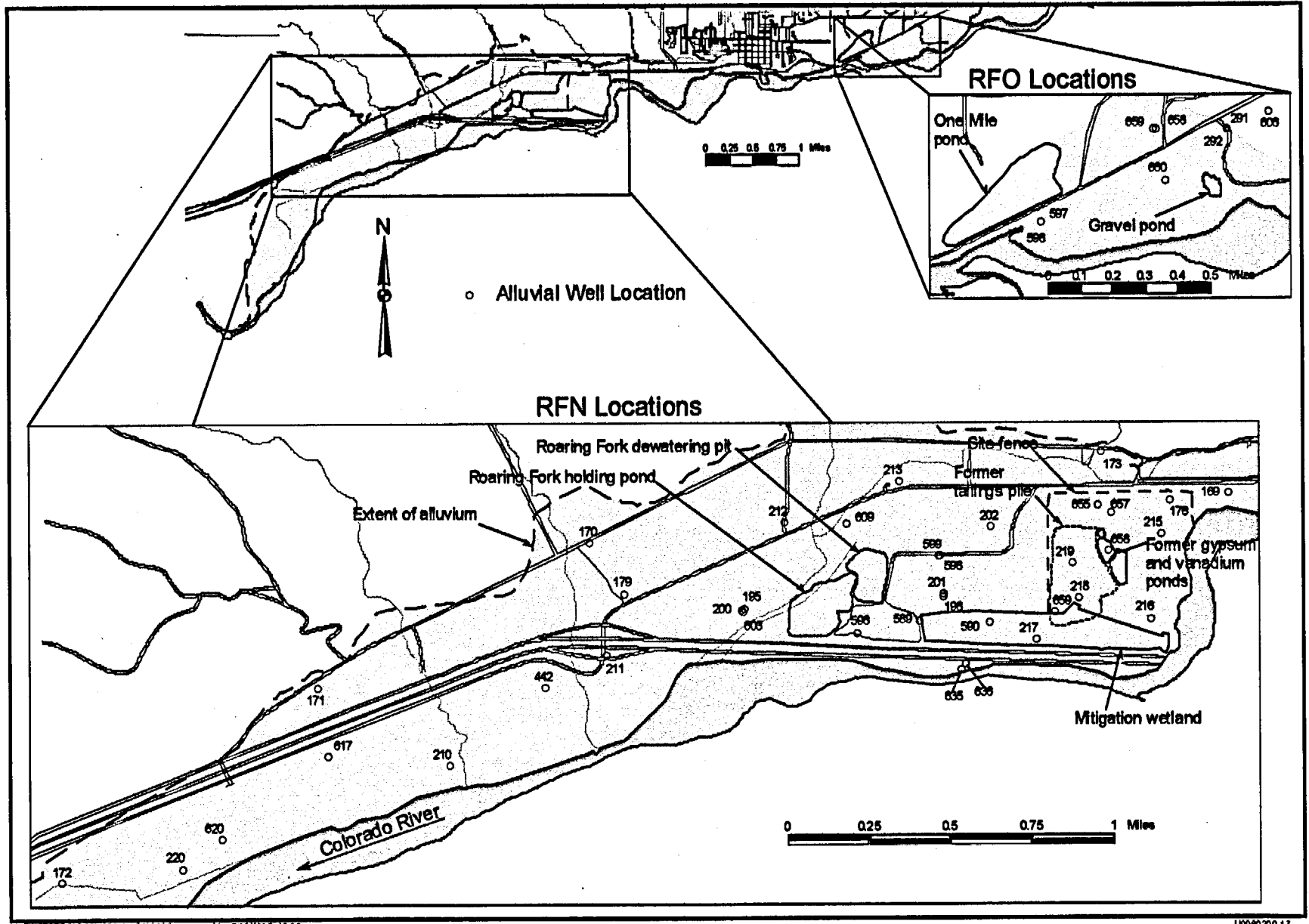
Figure 5-23. Alluvial Ground Water Monitor Well Sampling Locations
