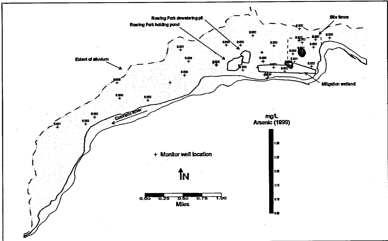
Figure 5-30. Arsenic Distribution in Alluvial Ground Water—New Rifle, 1999
