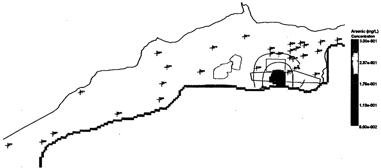
Figure 51. Predicted Arsenic Concentrations in the Ground Water at the New Rifle Site at 100 Years —100 Simulations
