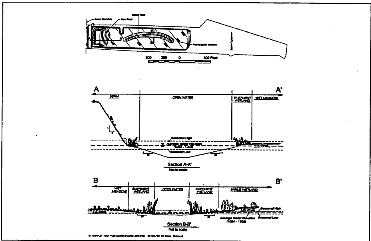
Figure 5-14. Mitigation Wetland Reconstruction Design
