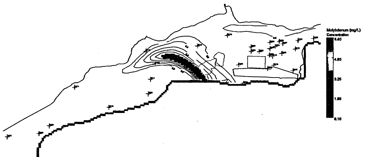
Figure 66. Predicted Molybdenum Concentrations in the Ground Water at the New Rifle Site at 20 Years—100 Simulations
