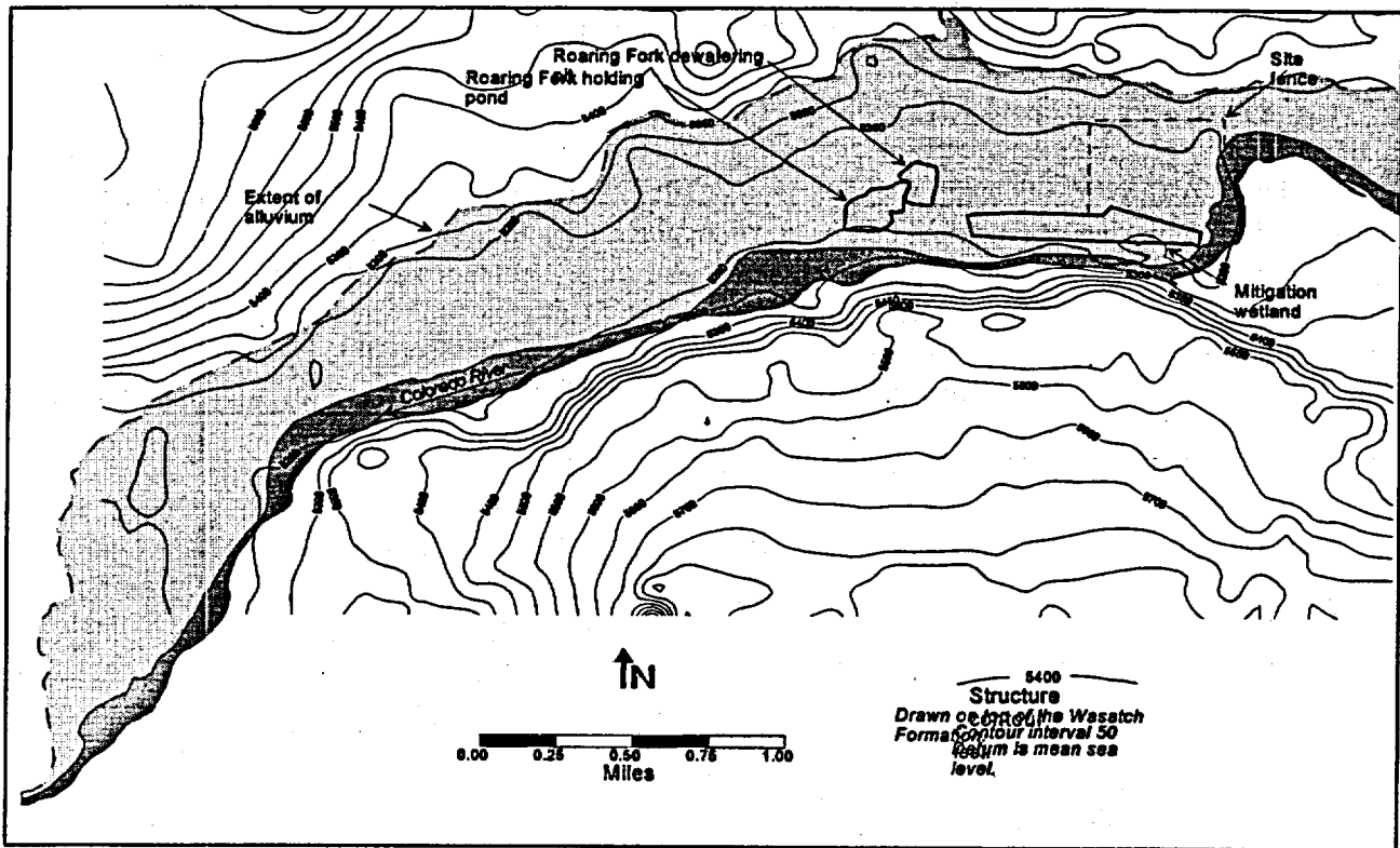
Figure 3. Bedrock Contour Map for the Wasatch Formation at New Rifle
