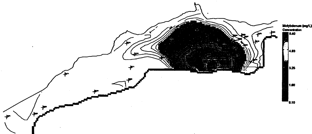
Figure 63. Predicted Molybdenum Concentrations in the Ground Water at the New Rifle Site at 5 Years—100 Simulations
