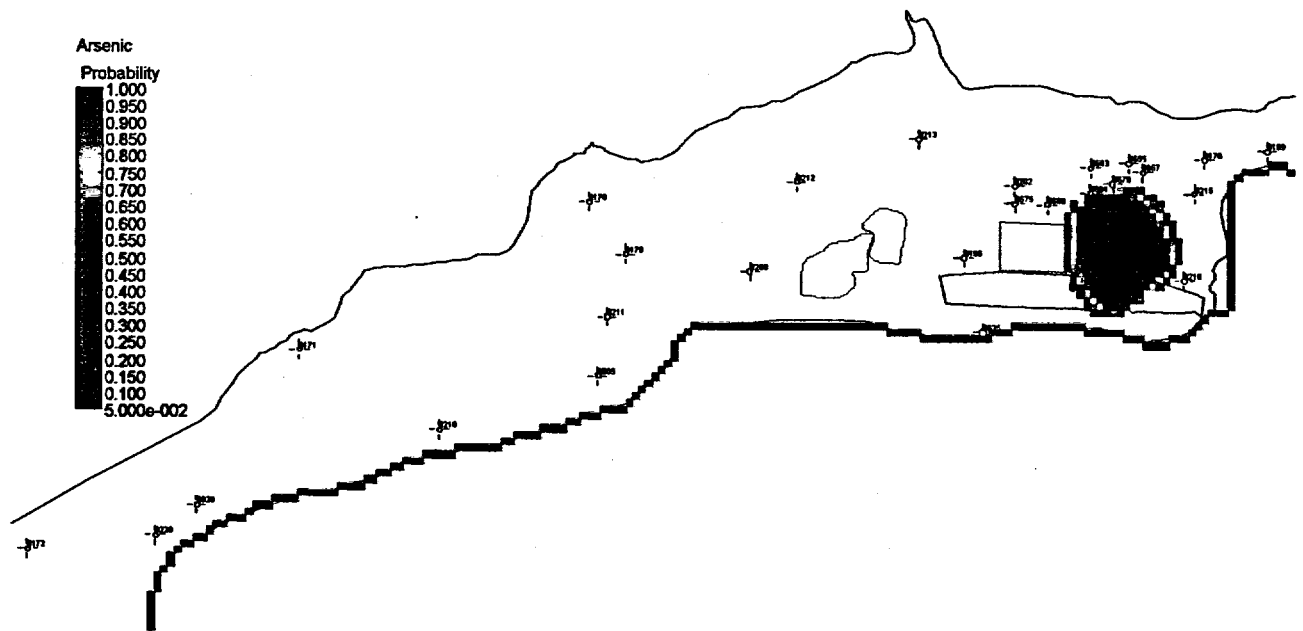
Figure 52. Probability of Arsenic Concentrations Exceeding the 0.05 mg/L UMTRA Ground Water Standard at the New Rifle Site at 25 Years
