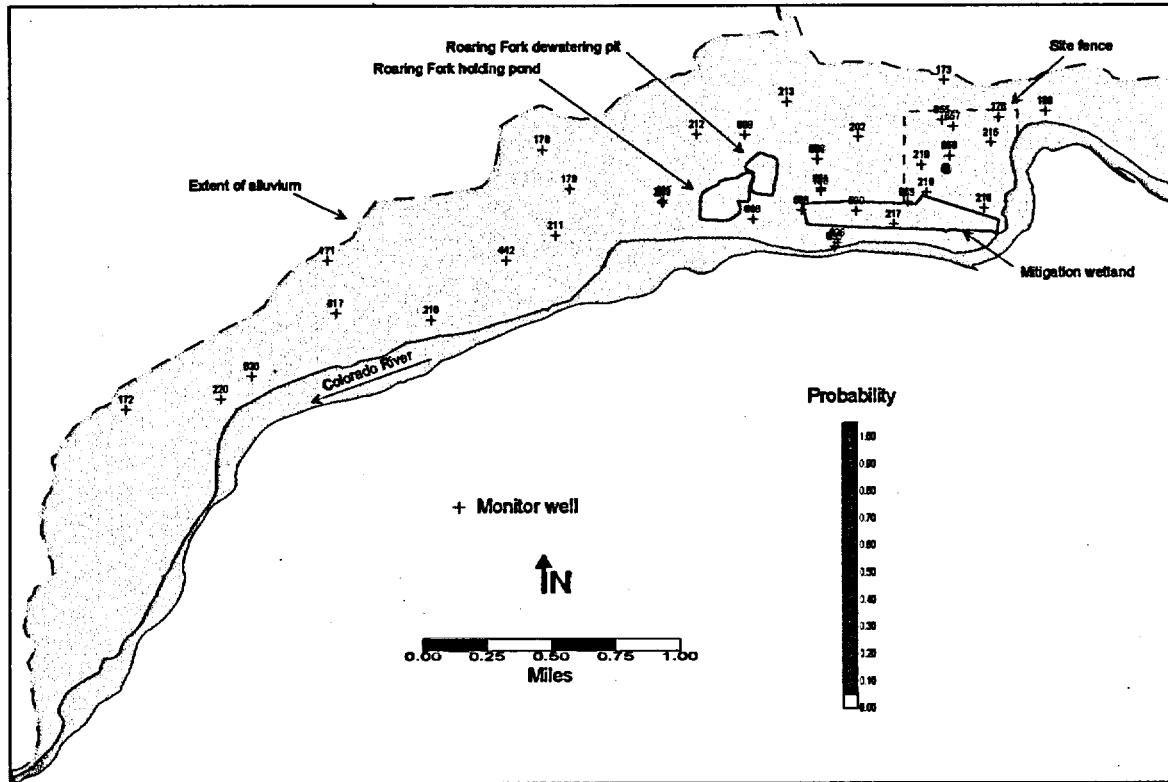
Figure 5-48. Probability of Arsenic Concentrations Exceeding the 0.05 mg/L UMTA Ground Water Standard at the New Rifle Site at 15 Years Based on the January 1999 Sampling Data—100 Simulations
