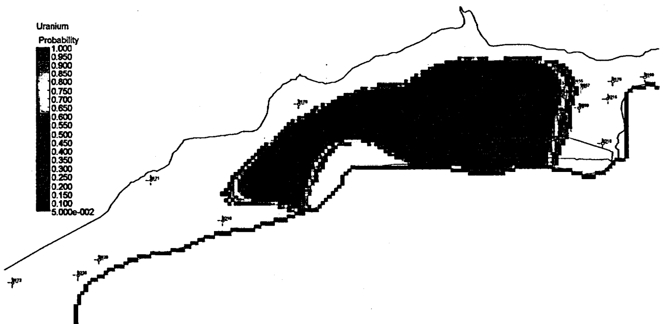
Figure 37. Probability of Uranium Concentrations Exceeding the 0.044 mg/L UMTRA Ground Water Standard at the New Rifle Site at 10 Years
