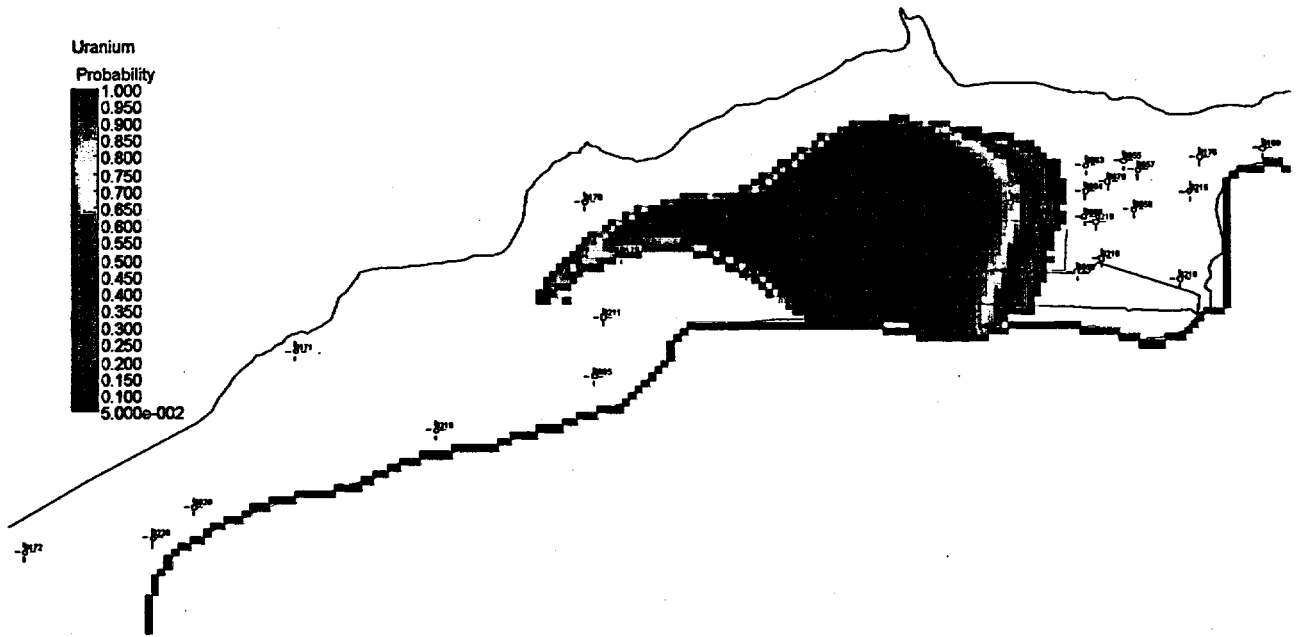
Figure 38. Probability of Uranium Concentrations Exceeding the 0.044 mg/L UMTRA Ground Water Standard at the New Rifle Site at 20 Years
