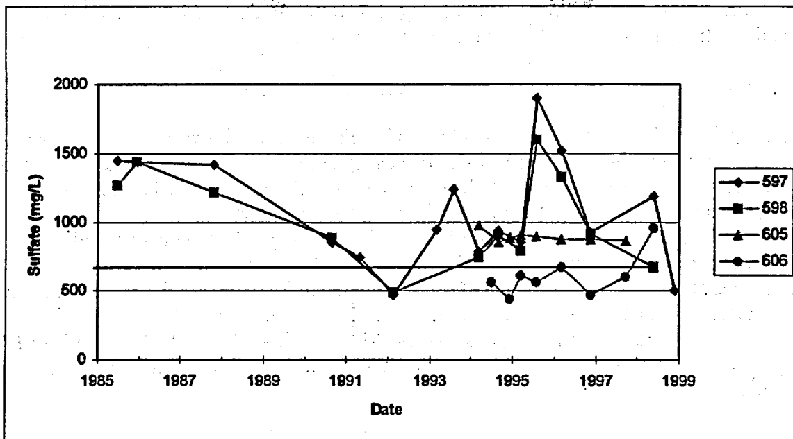
Figure 5-26. Time Concentration Plot for Background Alluvial Ground Water—Sulfate
