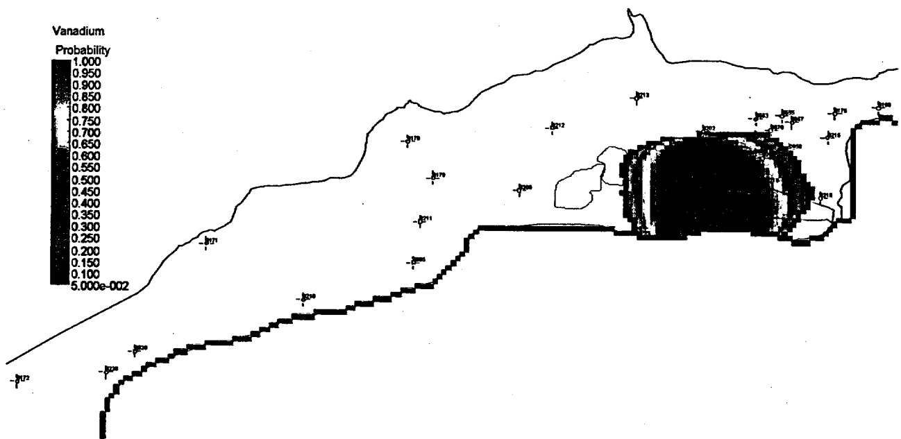
Figure 47. Probability of Vanadium Concentrations Exceeding the 0.33 mg/L Proposed Ground Water Cleanup Goal at the New Rifle Site at 100 Years
