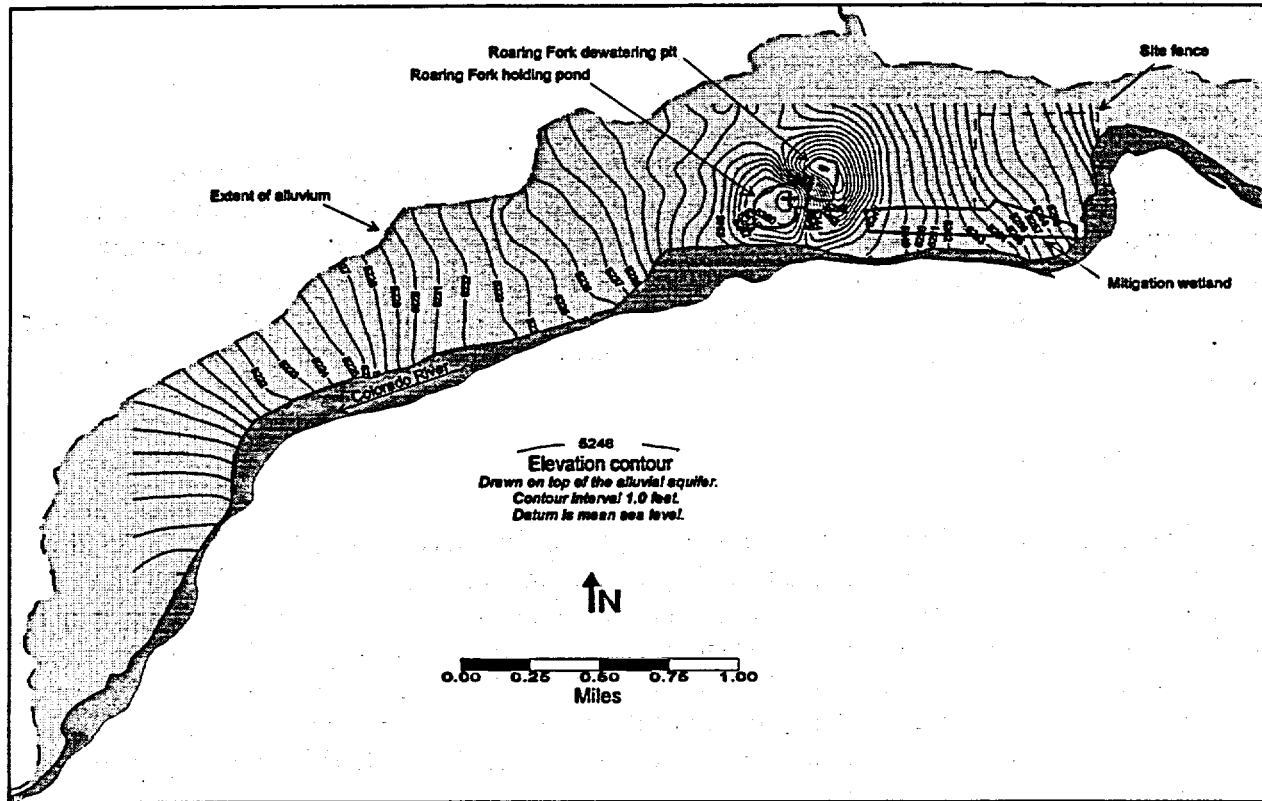
Figure 4. Alluvial Ground Water Elevations at New Rifle Site
