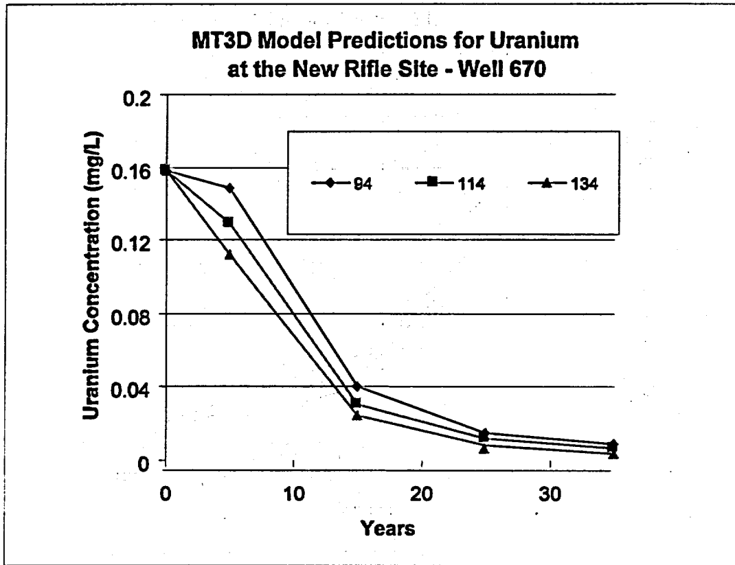
Figure 14. MT3D Sensitivity Analysis—Hydraulic Conductivity ( K_x )
