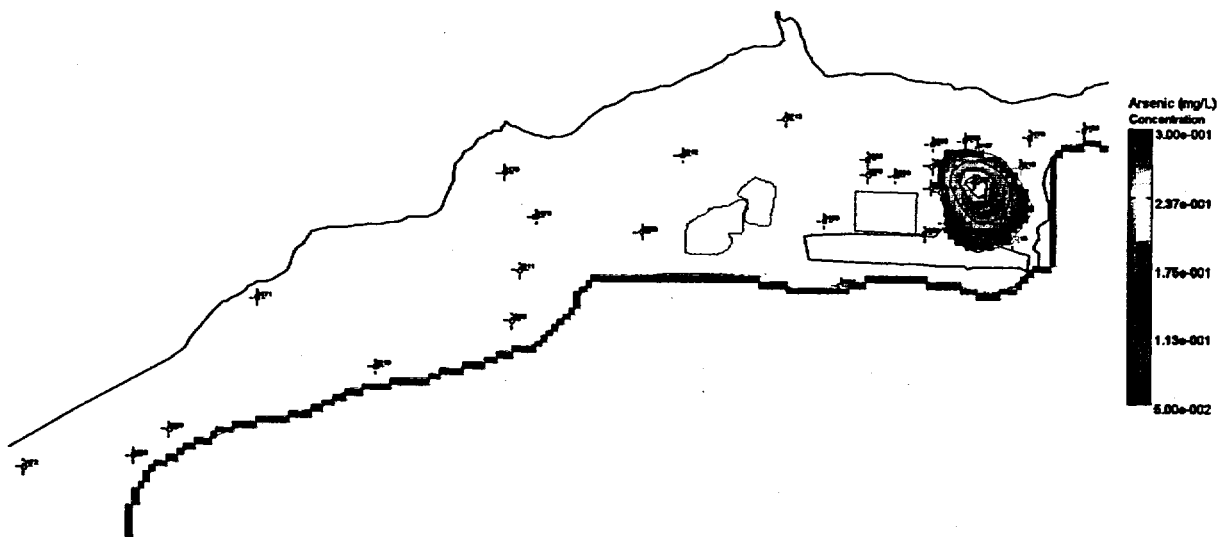
Figure 48. Initial Arsenic Concentrations in the Ground Water at the New Rifle Site Measured in July 1998
