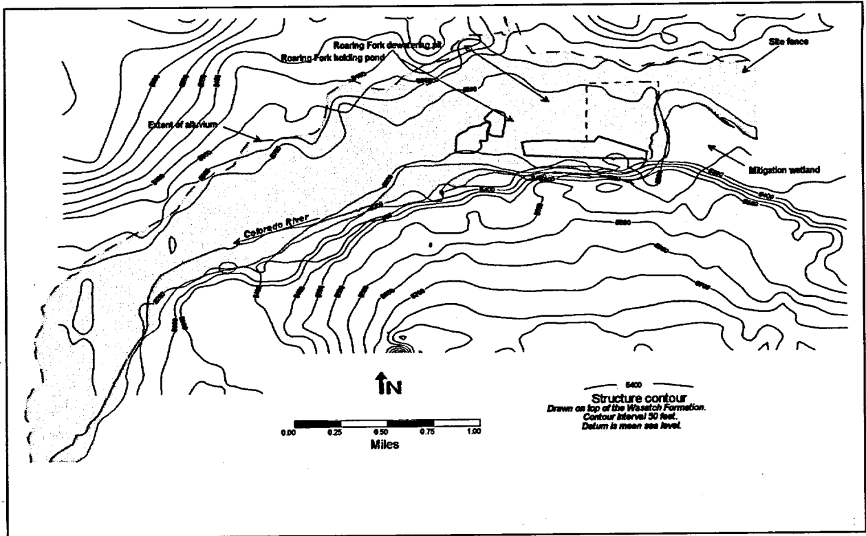
Figure 5-5. Contour Map Drawn on Top of the Wasatch Formation at the New Rifle Site
