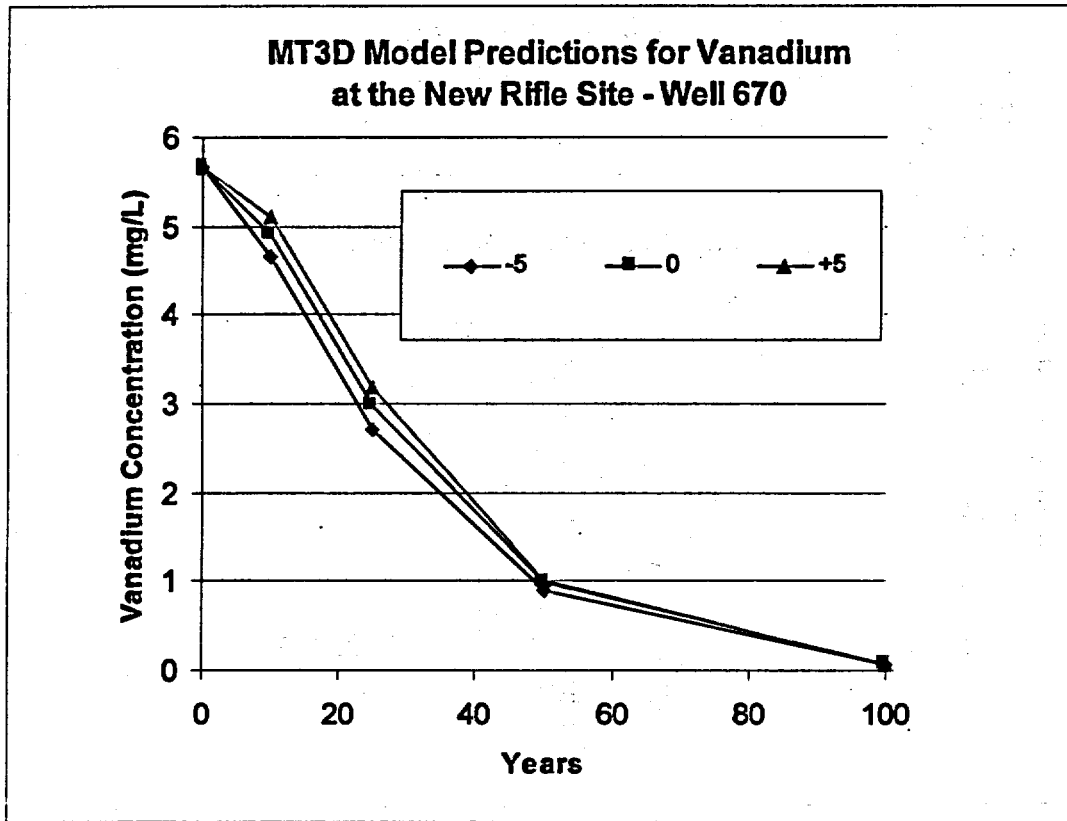
Figure 21. MT3D Sensitivity Analysis—River Stage
