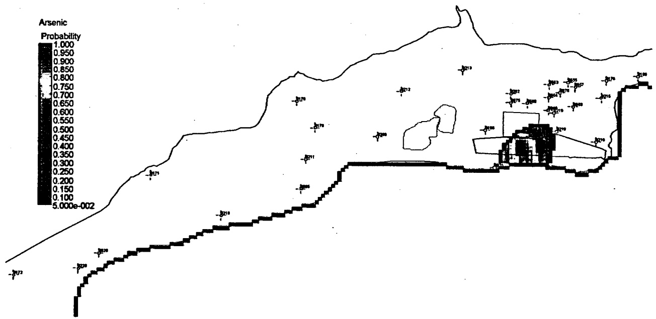
Figure 54. Probability of Arsenic Concentrations Exceeding the 0.05 mg/L UMTRA Ground Water Standard at the New Rifle Site at 100 Years
