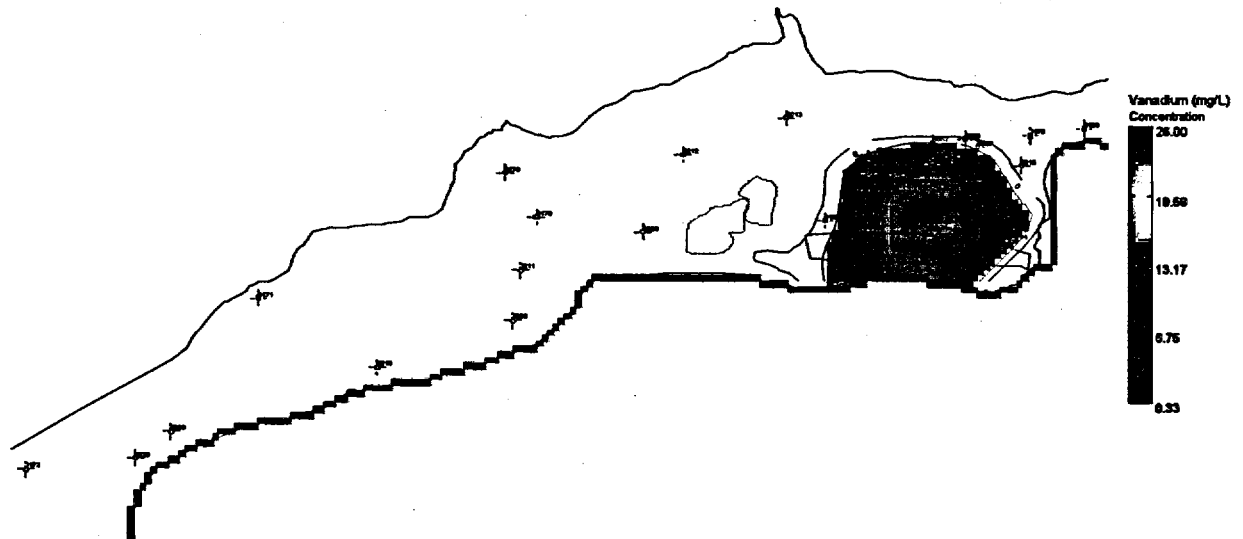
Figure 43. Predicted Vanadium Concentrations in the Ground Water at the New Rifle Site at 50 Years —100 Simulations
