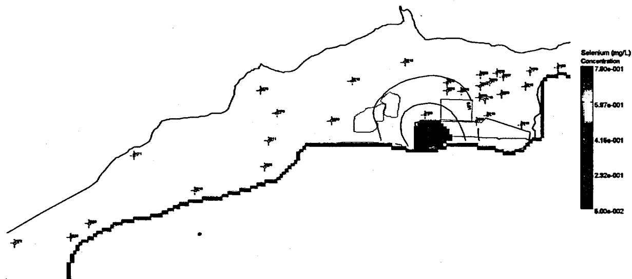
Figure 57. Predicted Selenium Concentrations in the Ground Water at the New Rifle Site at 75 Years —100 Simulations
