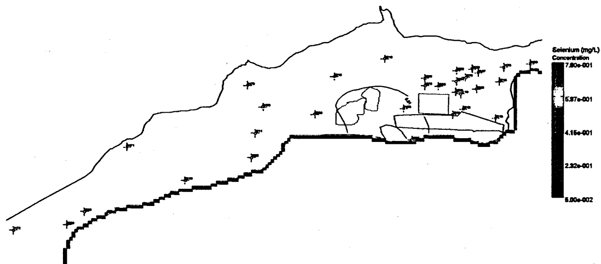
Figure 58. Predicted Selenium Concentrations in the Ground Water at the New Rifle Site at 100 Years —100 Simulations
