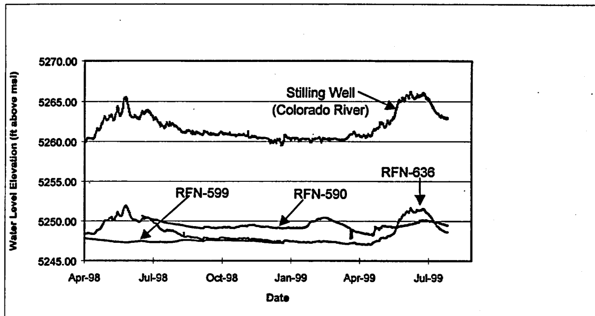
Figure 5-10. River Stage and Aquifer Response Measured at the New Rifle Site, April 1998 through July 1999
