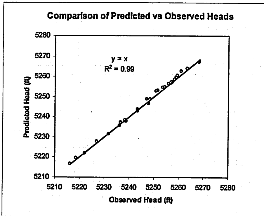
Figure 10. Comparison of Predicted vs. Observed Heads
