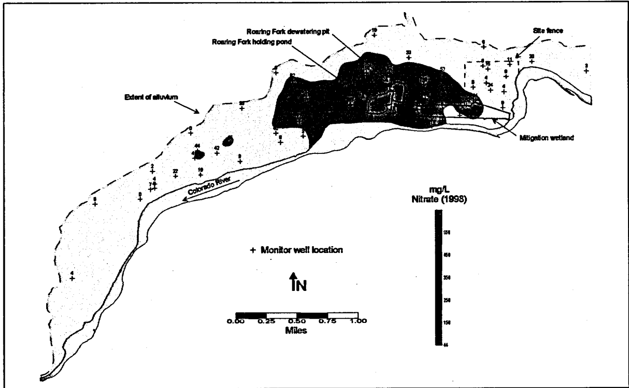
Figure 5-32. Nitrate Distribution in Alluvial Ground Water—New Rifle, 1998
