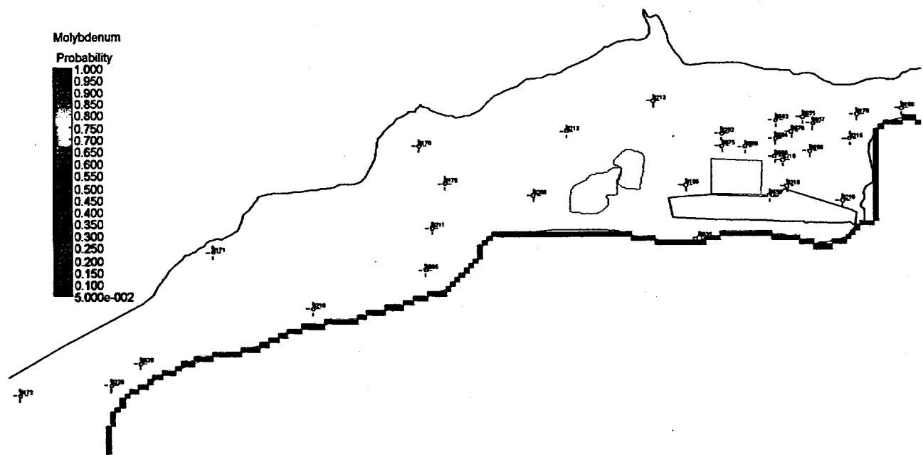
Figure 72. Probability of Molybdenum Concentrations Exceeding the 0.1 mg/L UMTRA Ground Water Standard at the New Rifle Site at 25 Years
