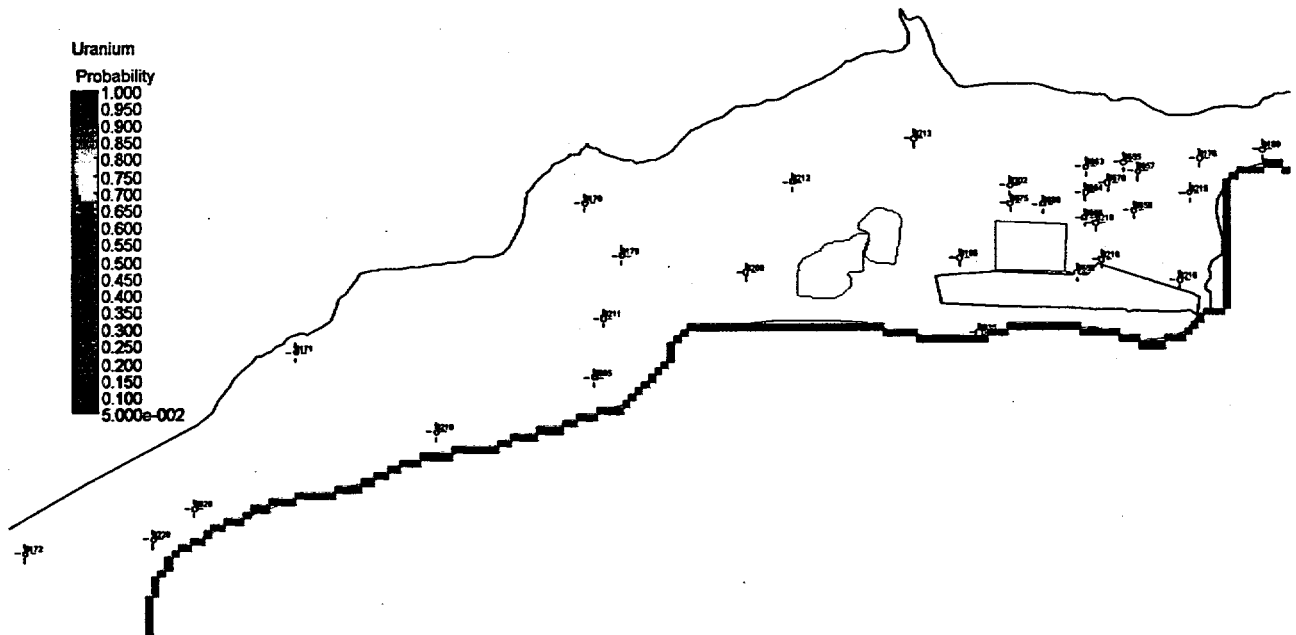
Figure 40. Probability of Uranium Concentrations Exceeding the 0.044 mg/L UMTRA Ground Water Standard at the New Rifle Site at 40 Years
