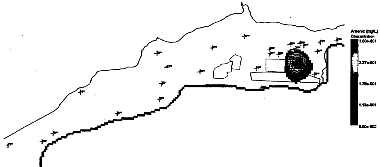
Figure 49. Predicted Arsenic Concentrations in the Ground Water at the New Rifle Site at 25 Years —100 Simulations
