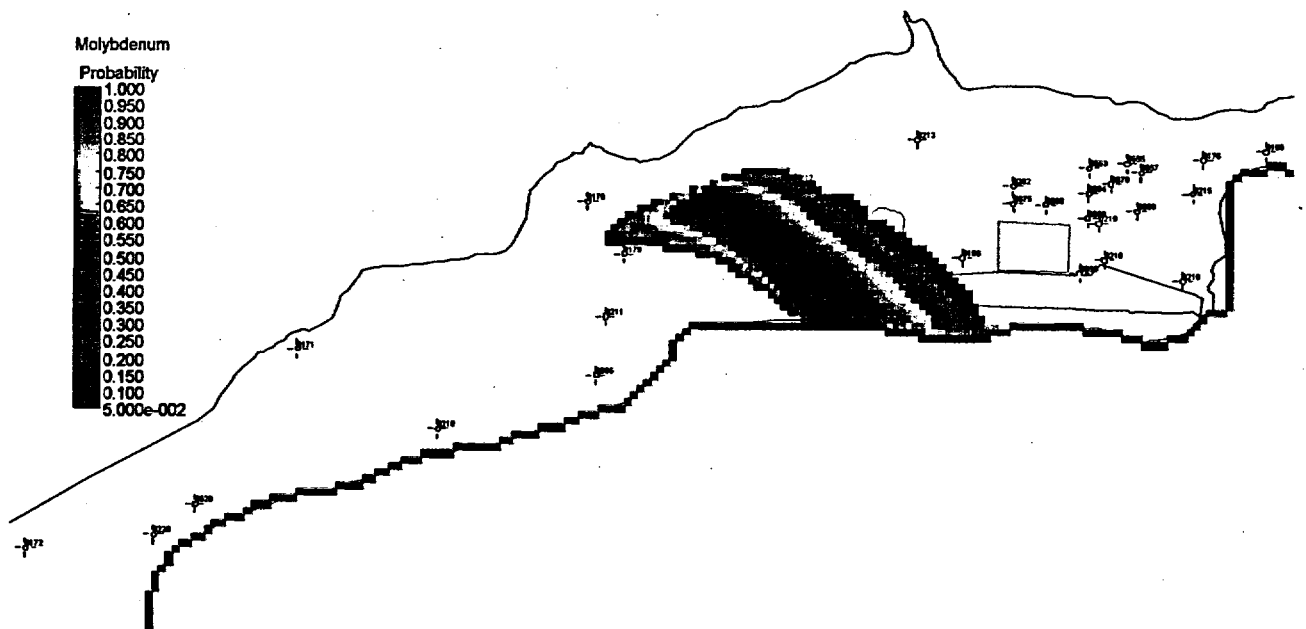
Figure 70. Probability of Molybdenum Concentrations Exceeding the 0.1 mg/L UMTRA Ground Water Standard at the New Rifle Site at 15 Years
