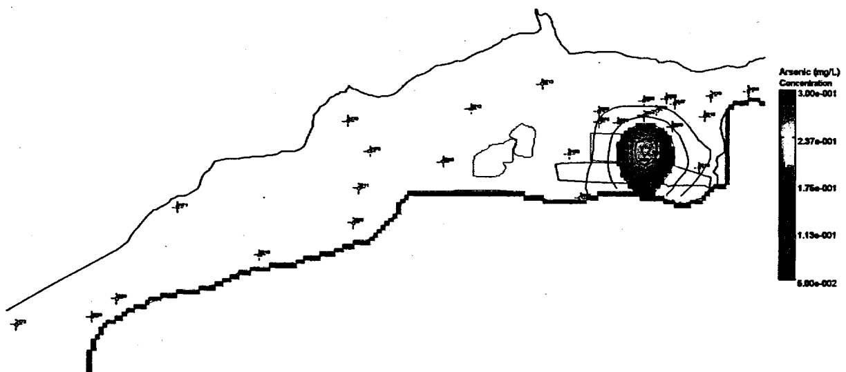
Figure 50. Predicted Arsenic Concentrations in the Ground Water at the New Rifle Site at 50 Years —100 Simulations
