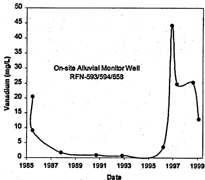
Figure 5-38. Vanadium Concentrations versus Time at On-Site Monitor Well Located near Former Gypsum/Vanadium Evaporation Pond
