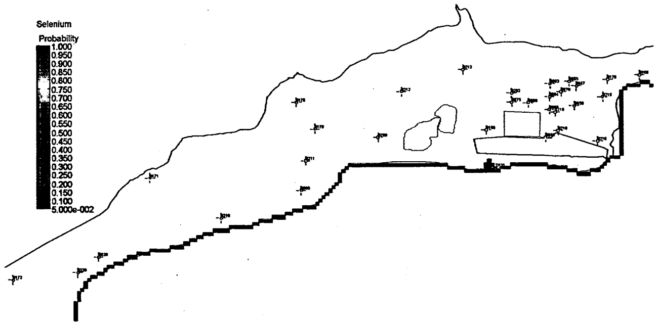
Figure 61. Probability of Selenium Concentrations Exceeding the 0.05 mg/L SDWA Ground Water Standard at the New Rifle Site at 100 Years
