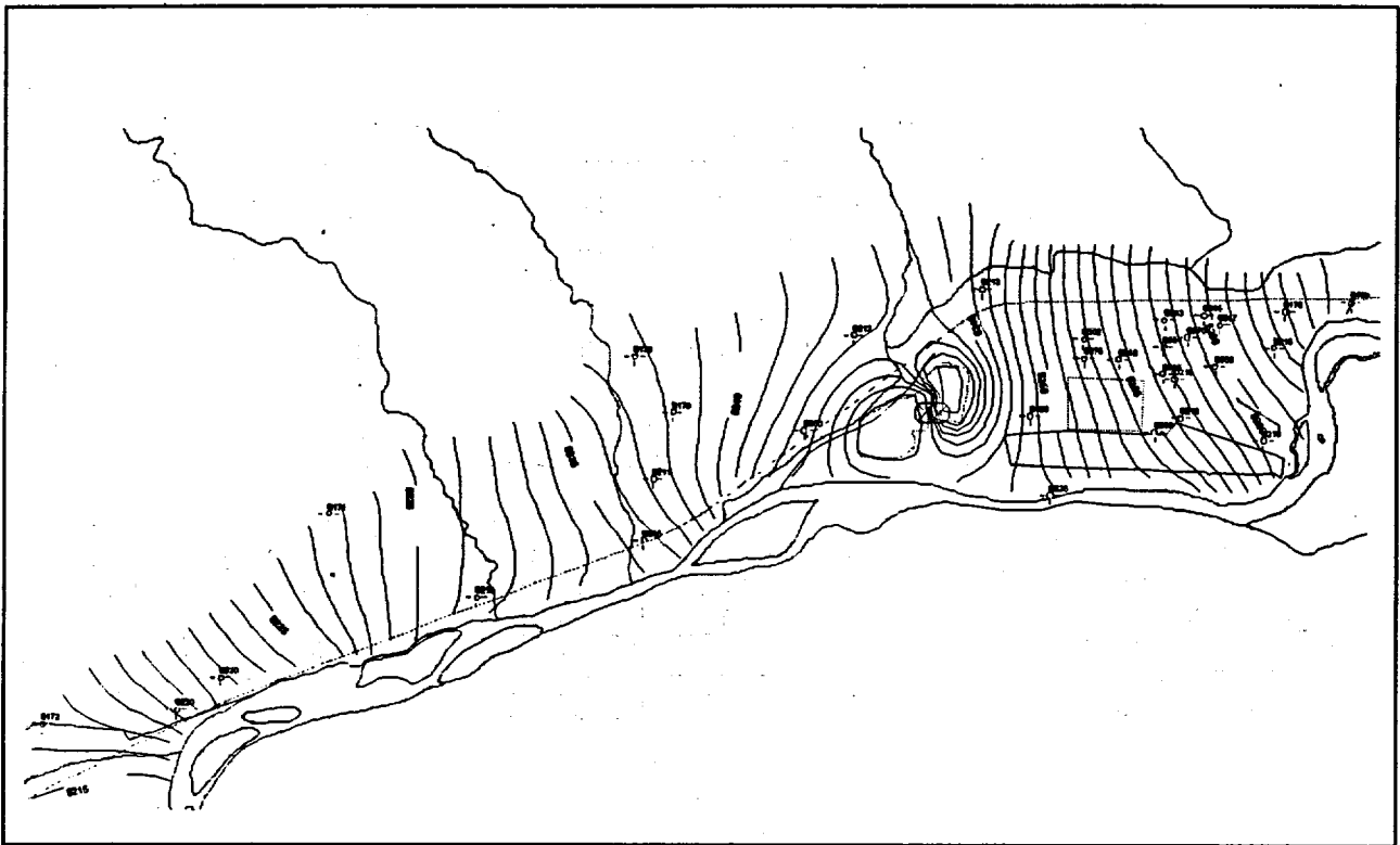
Figure 8. Simulated Steady State Ground Water Elevations
