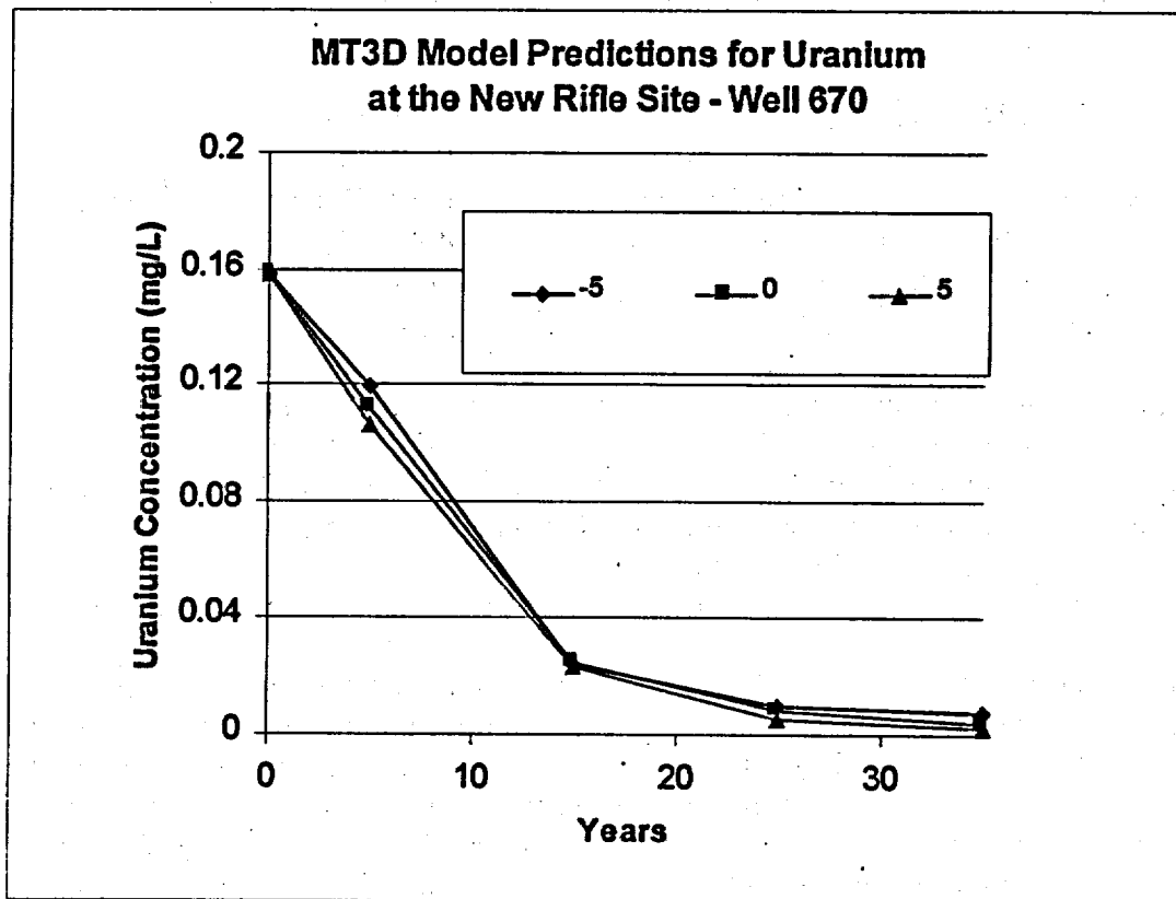
Figure 20. MT3D Sensitivity Analysis—River Stage
