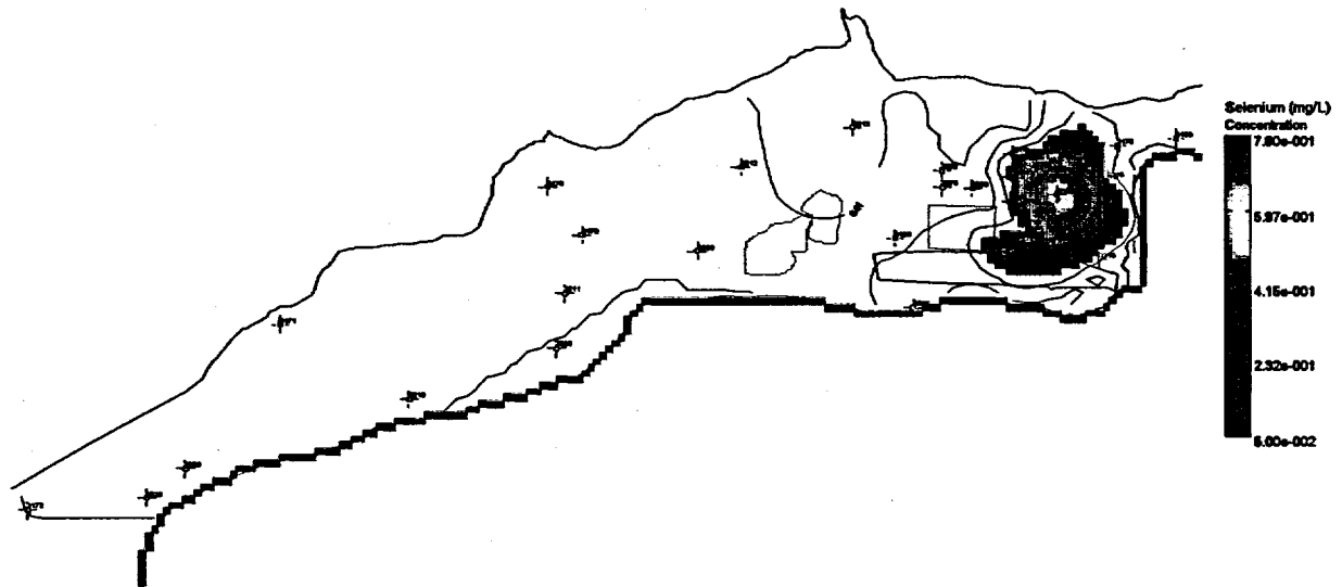
Figure 55. Initial Selenium Concentrations in the Ground Water at the New Rifle Site Measured in July 1998
