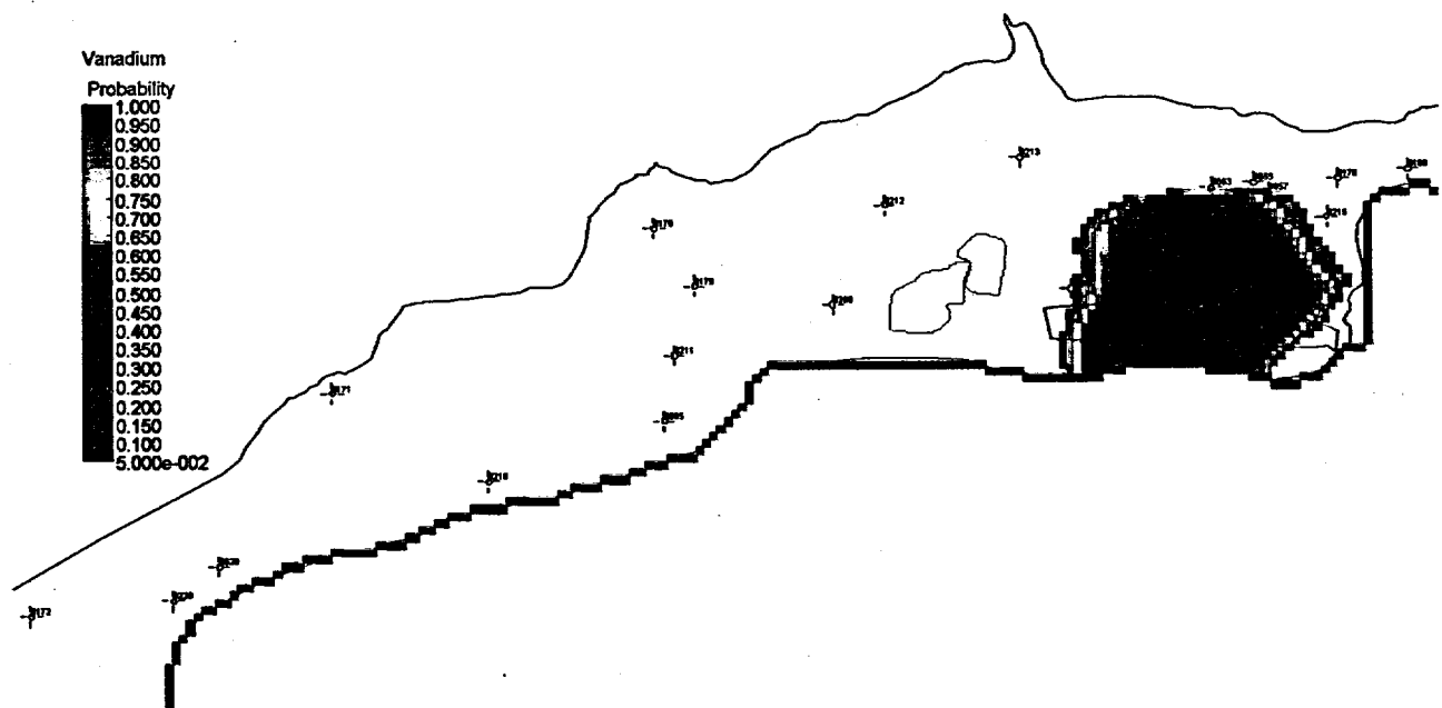
Figure 46. Probability of Vanadium Concentrations Exceeding the 0.33 mg/L Proposed Ground Water Cleanup Goal at the New Rifle Site at 50 Years
