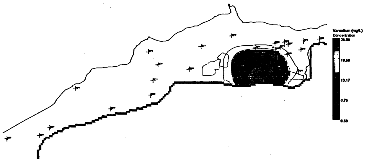
Figure 44. Predicted Vanadium Concentrations in the Ground Water at the New Rifle Site at 100 Years —100 Simulations
