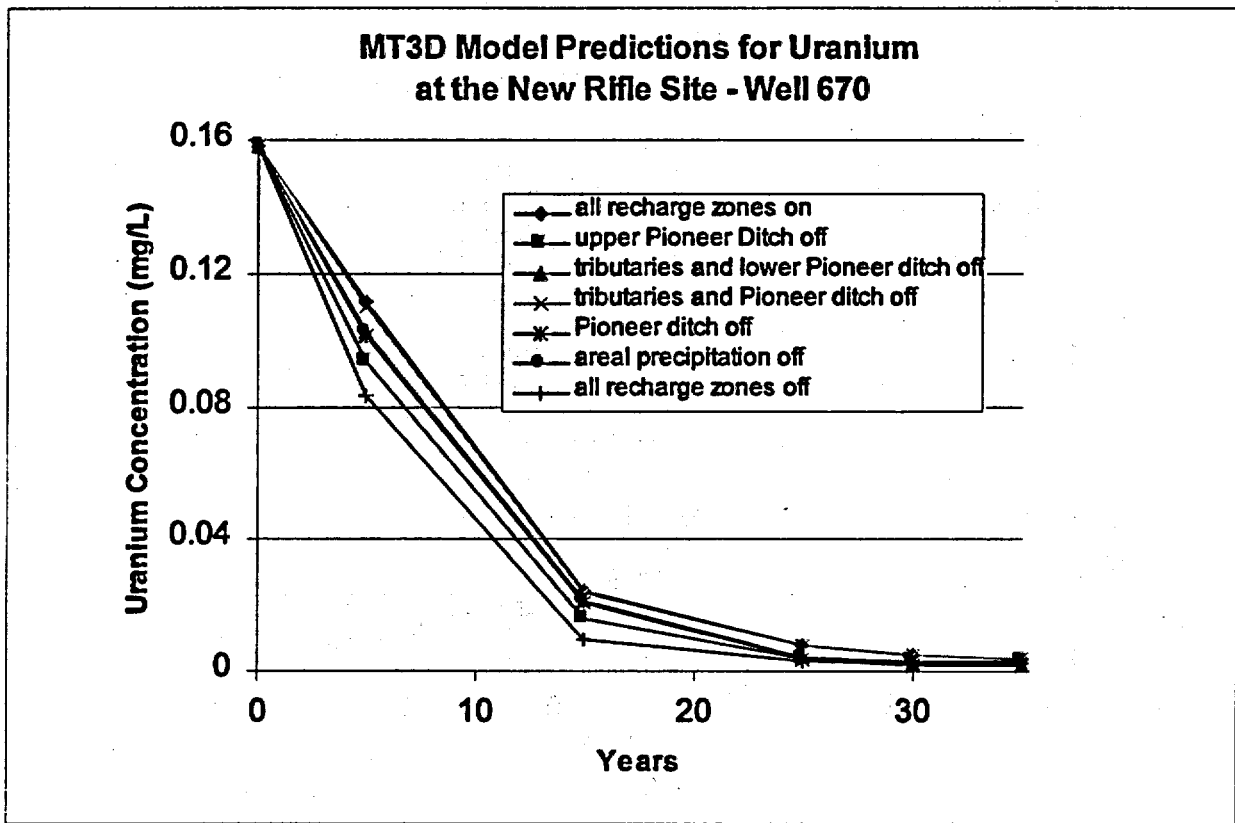
Figure 16. MT3D Sensitivity Analysis—Recharge
