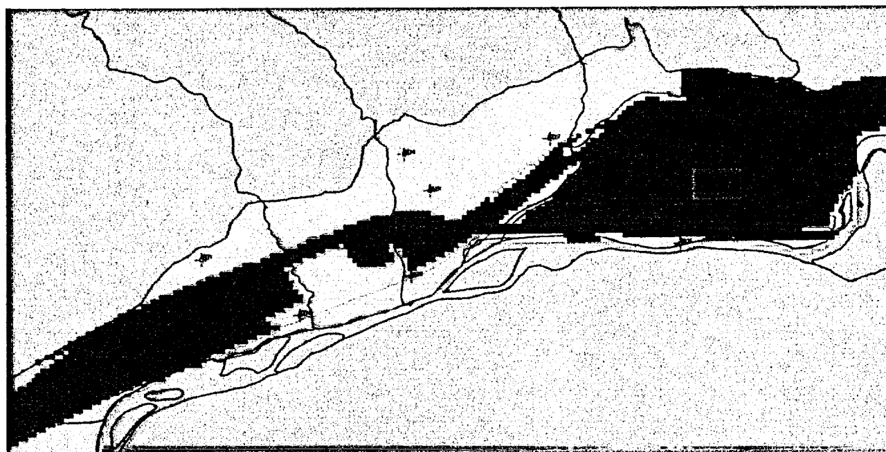
Figure 7. Evapotranspiration Zones
