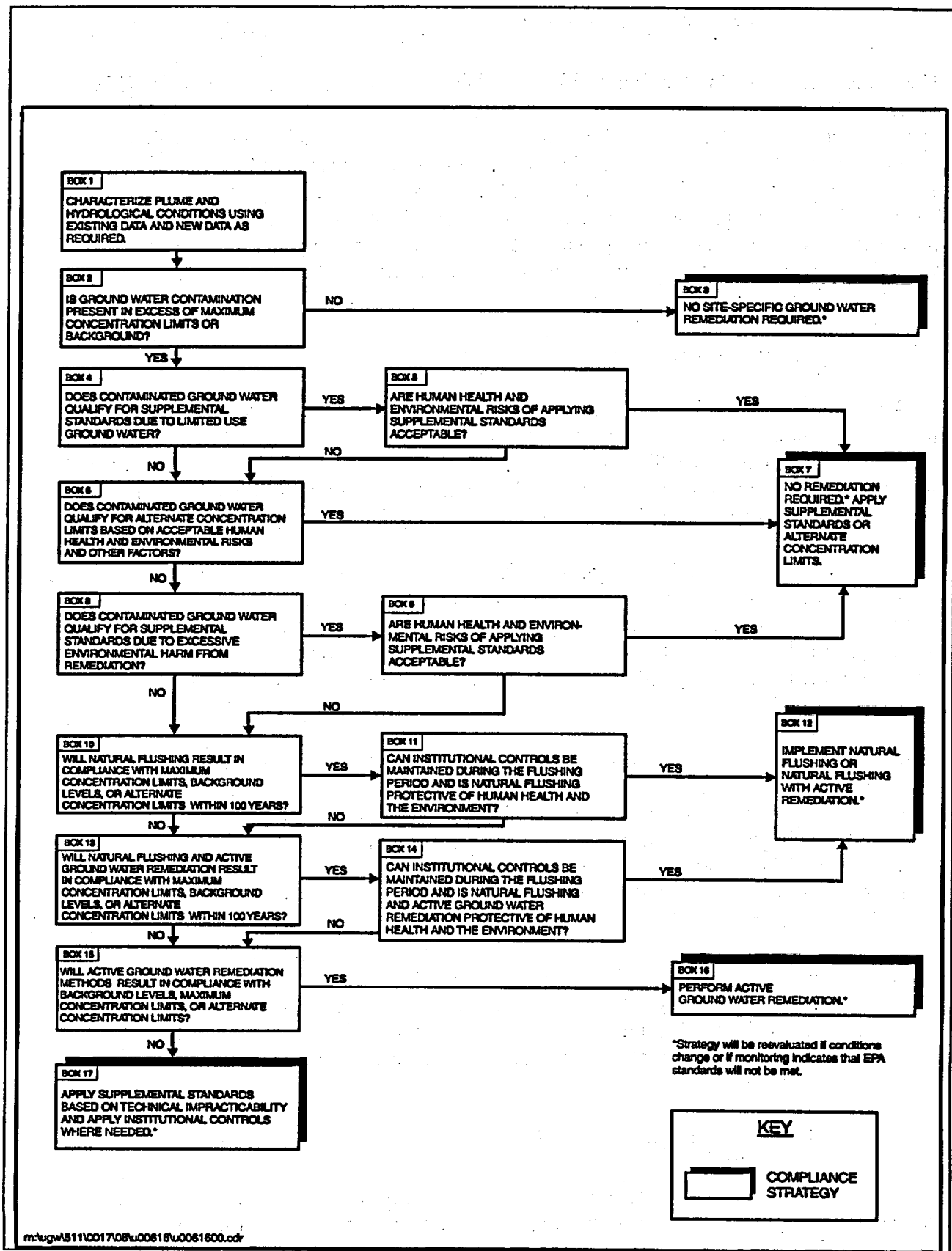
Figure 7-1. Summary of Ground Water Compliance Selection Framework
