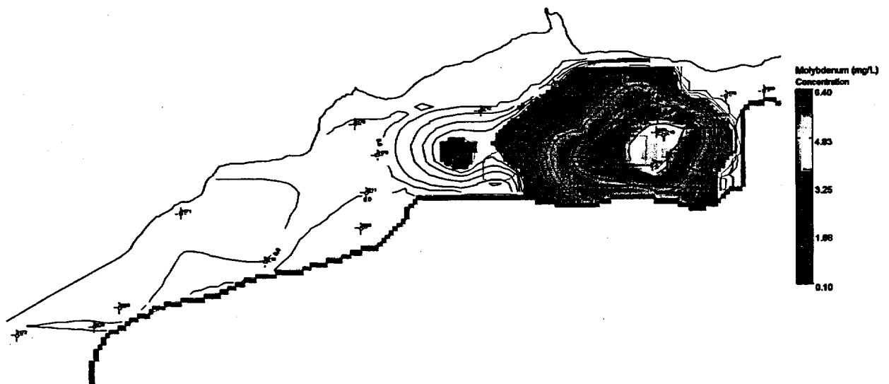
Figure 62. Initial Molybdenum Concentrations in the Ground Water at the New Rifle Site Measured in July 1998
