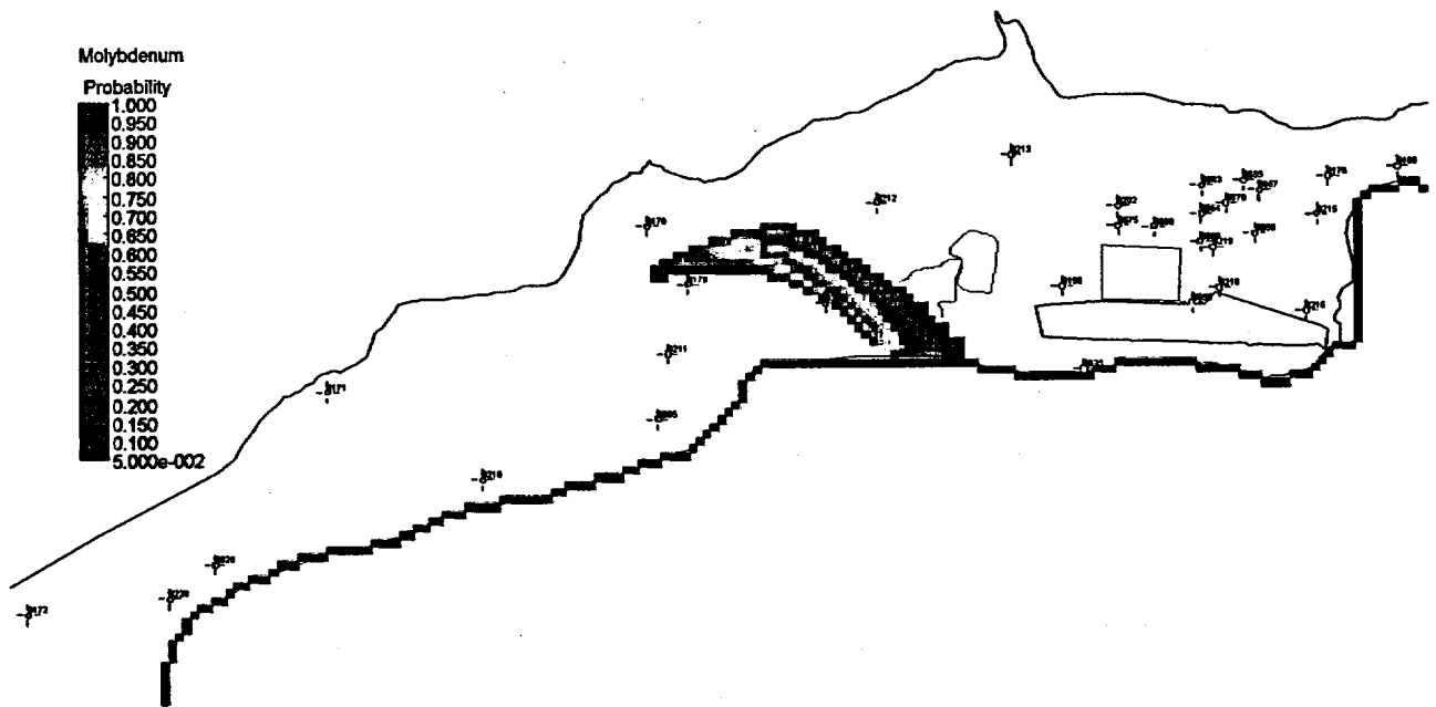
Figure 71. Probability of Molybdenum Concentrations Exceeding the 0.1 mg/L UMTRA Ground Water Standard at the New Rifle Site at 20 Years
