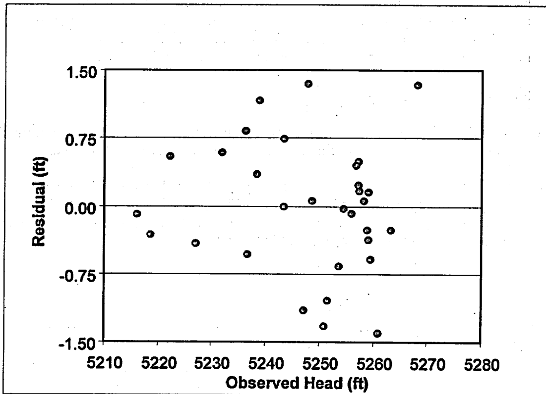
Figure 9. Comparison of Residual vs. Observed Head
