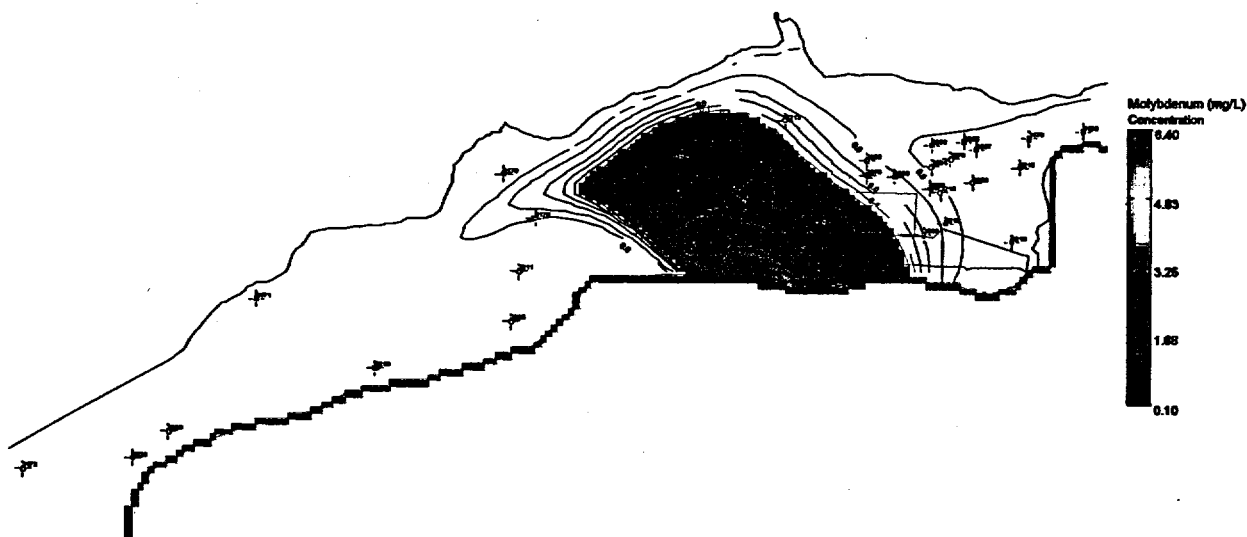
Figure 64. Predicted Molybdenum Concentrations in the Ground Water at the New Rifle Site at 10 Years—100 Simulations
