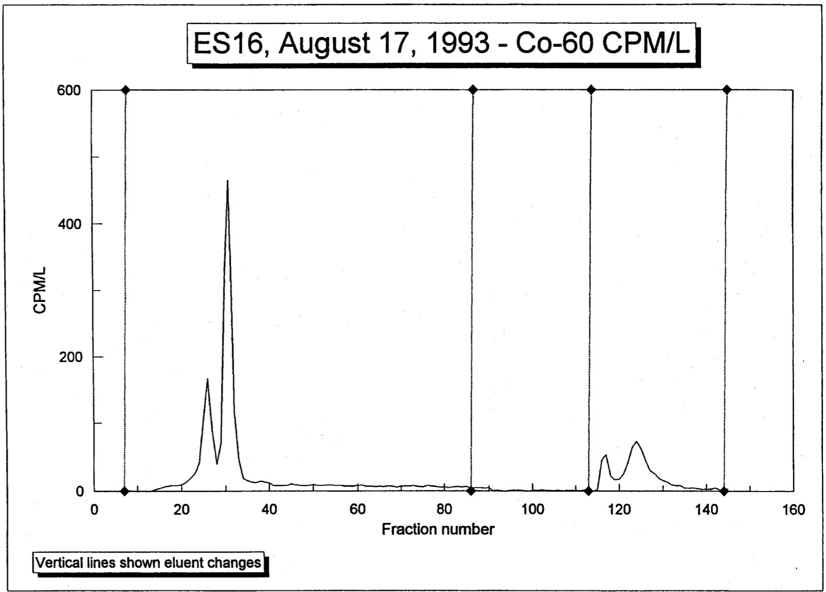
Figure 3.16 Cobalt-60 chromatogram for well ES16 August 17, 1993 sample
