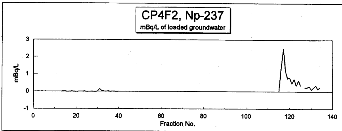
Figure 3.9 Np-237 chromatograms for samples from the three wells
