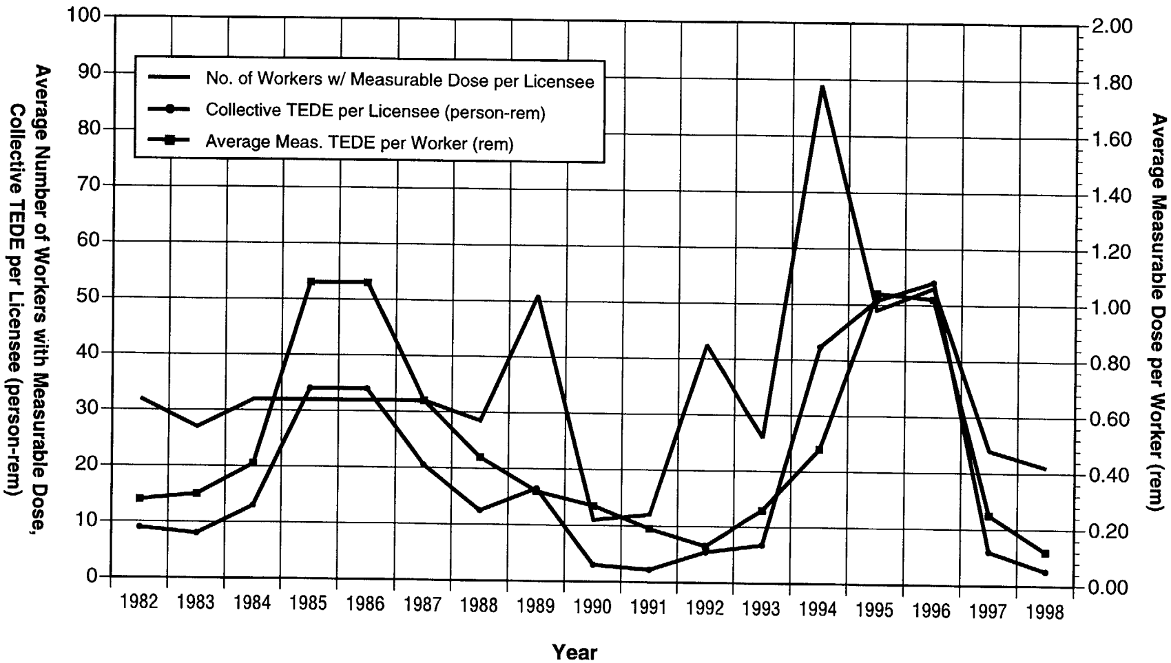
FIGURE 3.9. Average Annual Values at Independent Spent Fuel Storage Facilities 1982 - 1998
