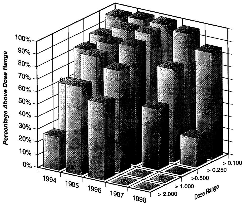
FIGURE 3.10. Collective TEDE Distribution by Dose Range Independent Spent Fuel Storage Licensees
