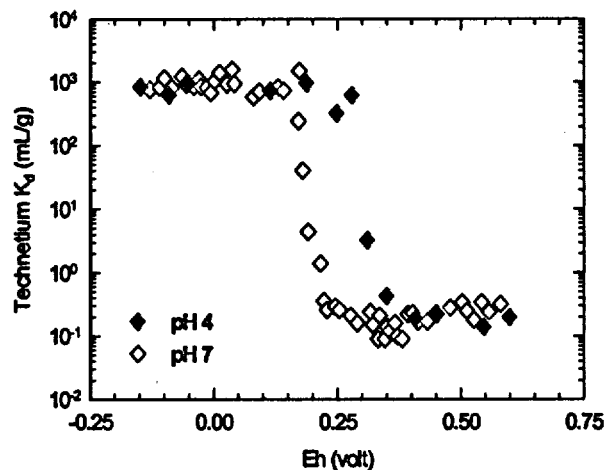
Figure 2. Technetium sorption coefficient, K_d , as a function of Eh. Values taken from Lieser and Bauscher 1
