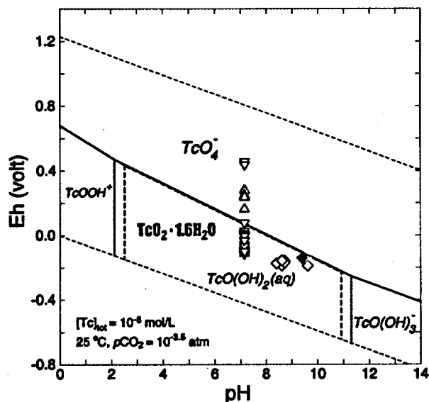
Figure 1. Eh-pH diagram for aqueous Tc species calculated using the NEA thermodynamic data. 9 Also shown are Eh measured in well UE-25 WT#17 ( \Delta, \nabla ) 5 , and on samples from wells USW H-3 ( \diamond ) and USW H-4 ( \diamond ). 6
