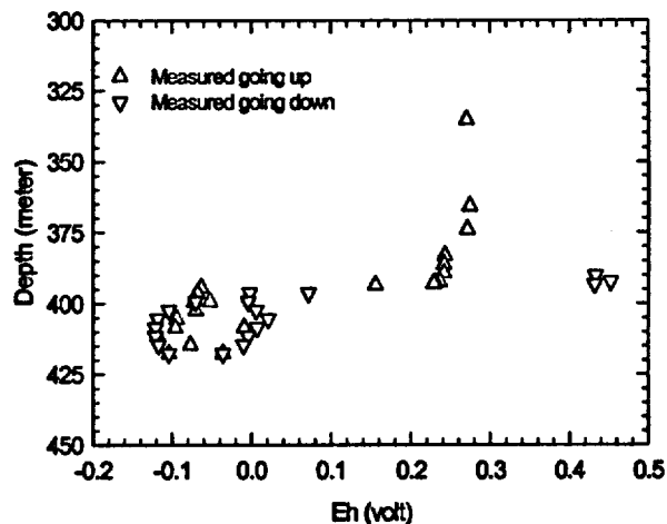
Figure 3. Eh measured downhole in well UE-25 WT#17. Data taken from DOE (1999; data tracking number LAAM831311AQ98.003) 5
