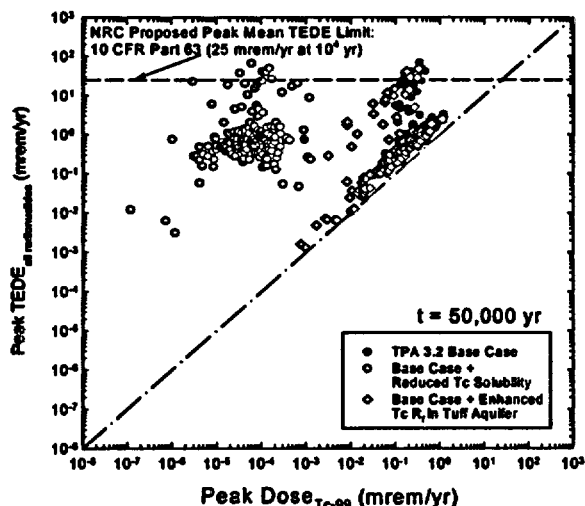
Figure 6. Calculated peak TEDE and Tc-99 dose. Values for each of 250 realizations are plotted. Symbols as in Fig. 4. Calculations with enhanced retardation along the full length of the saturated zone or in the alluvial aquifer only resulted in zero Tc-99 dose and are not plotted. The dashed-dotted line represents a 1:1 relationship between log (Peak TEDE) and log (Dose Tc-99 ). Points along the line indicate that the peak dose is all due to Tc-99.
