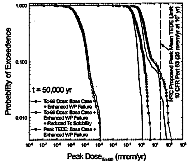
Figure 5. CCDF for Tc-99 dose calculated using Alloy 625, instead of Alloy C-22, properties to simulate earlier WP failure, and the base case parameter set 8 or the base case parameters with decreased Tc solubility limit. Calculations with enhanced retardation along the full length of the saturated zone, which resulted in zero Tc-99 dose, are not plotted. The heavy lines are the CCDFs for Tc dose and TEDE for the base case with Alloy C-22 taken from Fig. 4.
