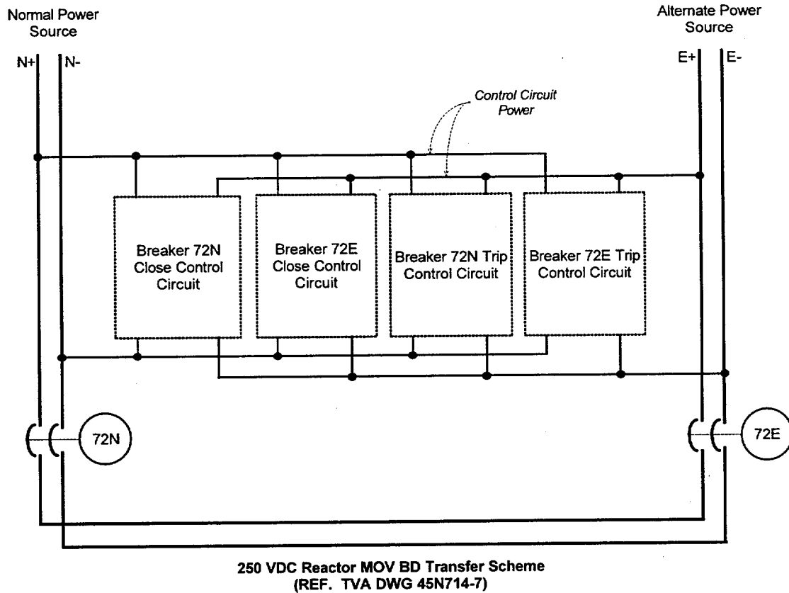
Figure C-7. Breaker control circuit block diagram. Note control power is tapped off both sources. (Detail of the 72N Trip Control Circuit is provided in Fig. 8.)
