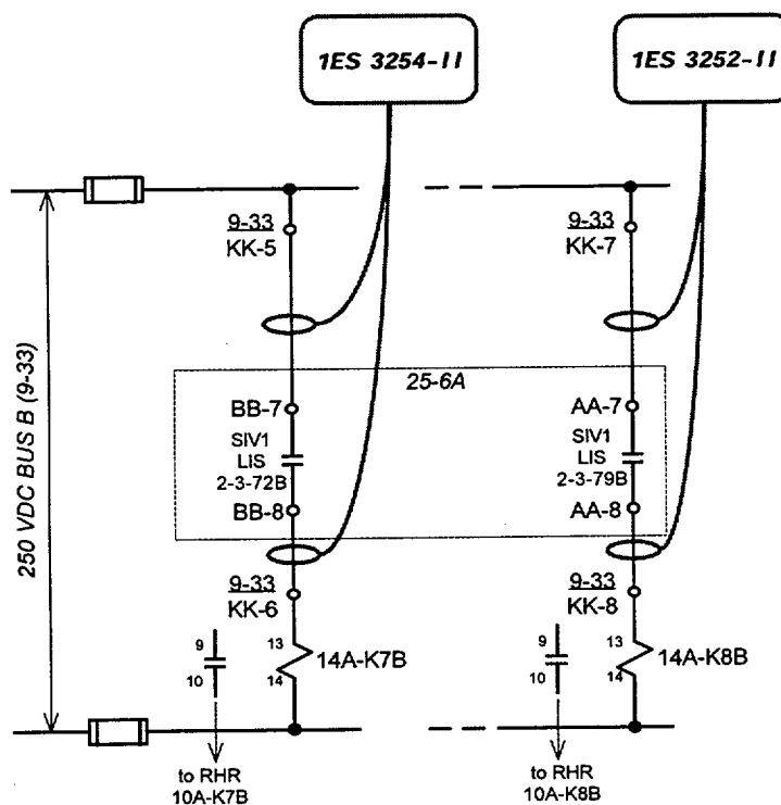
Figure C-2. Partial schematic of Core Spray relay logic circuit.
