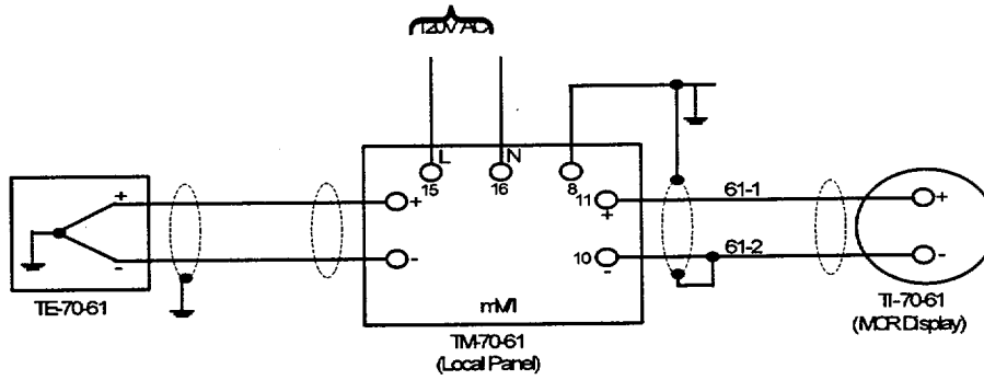
Figure B-4. Thermocouple sensor circuit.
