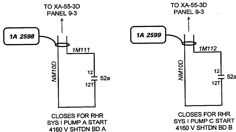
Figure C-3. Partial schematic of annunciator circuit for the RHR Pump Start alarms.
