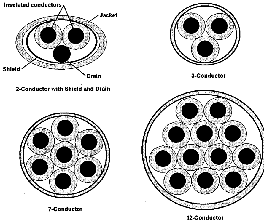
Figure 2-1: Illustration of common multi-conductor cable arrangements.
