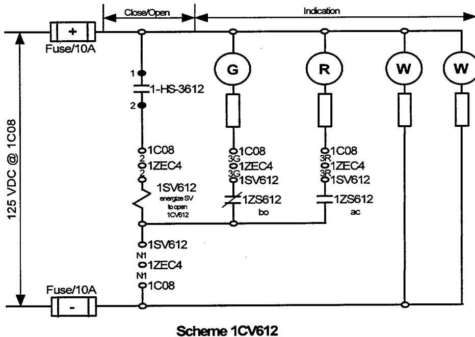
Figure B-1. Solenoid-operated valve control circuit.
