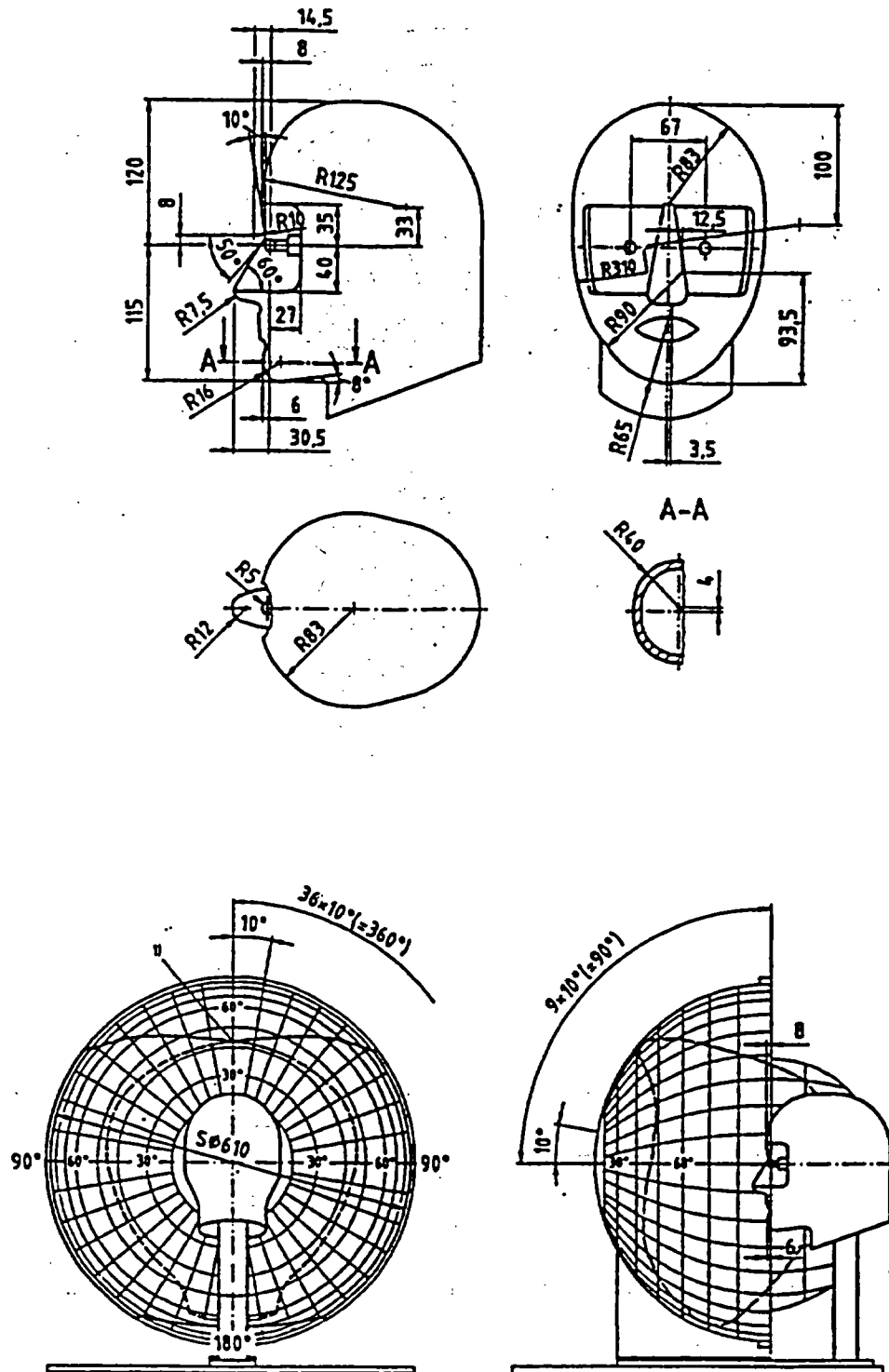
Figure 3 — Stoll apertometer
